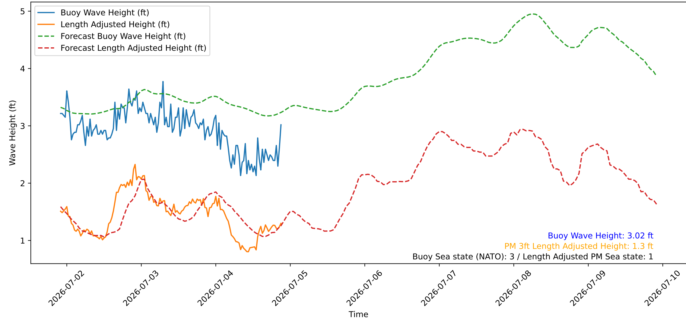
Wave Heights over Time for Oceanside Harbor at 2026-07-04 21:50:26
