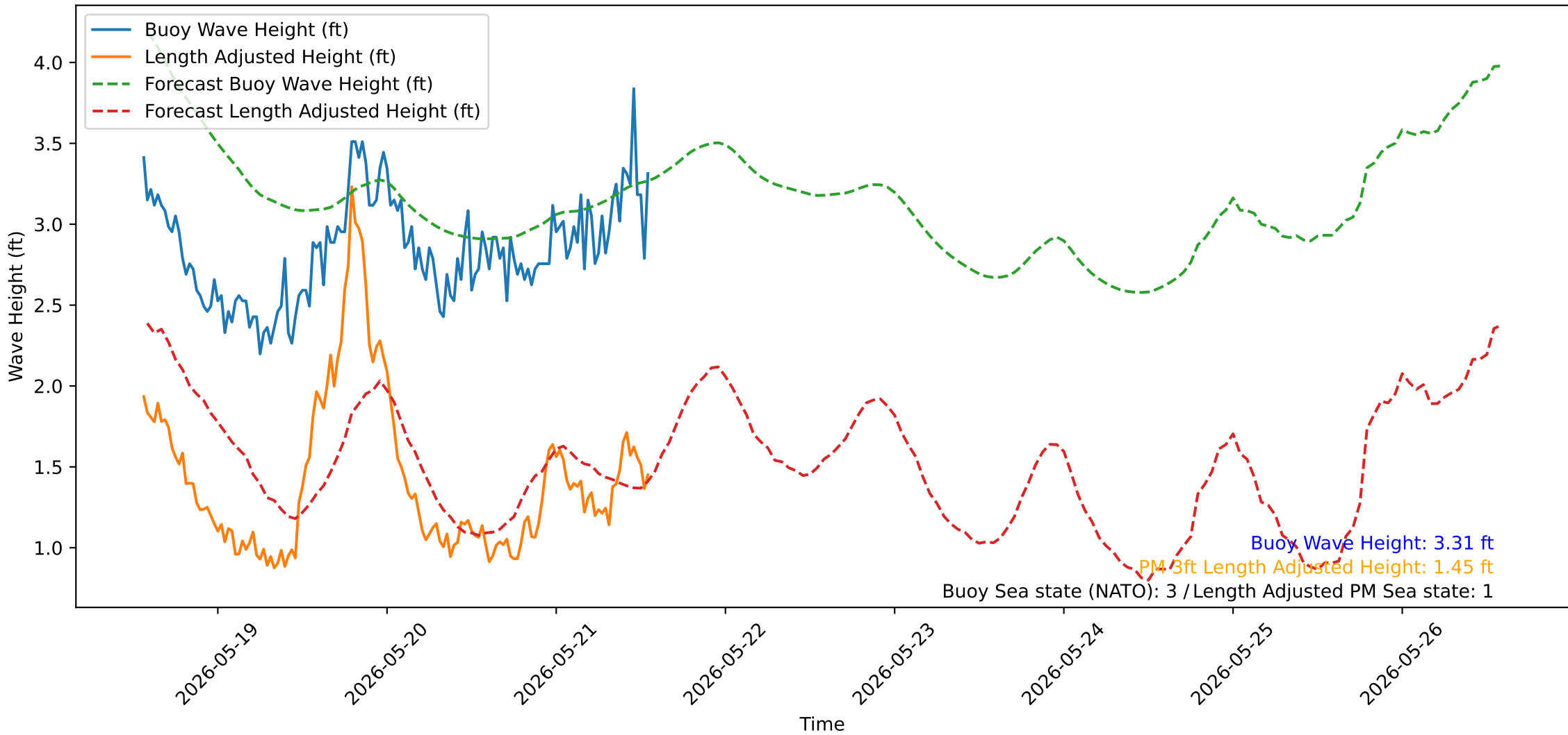
Wave Heights over Time for Oceanside Harbor at 2026-05-21 13:30:31
