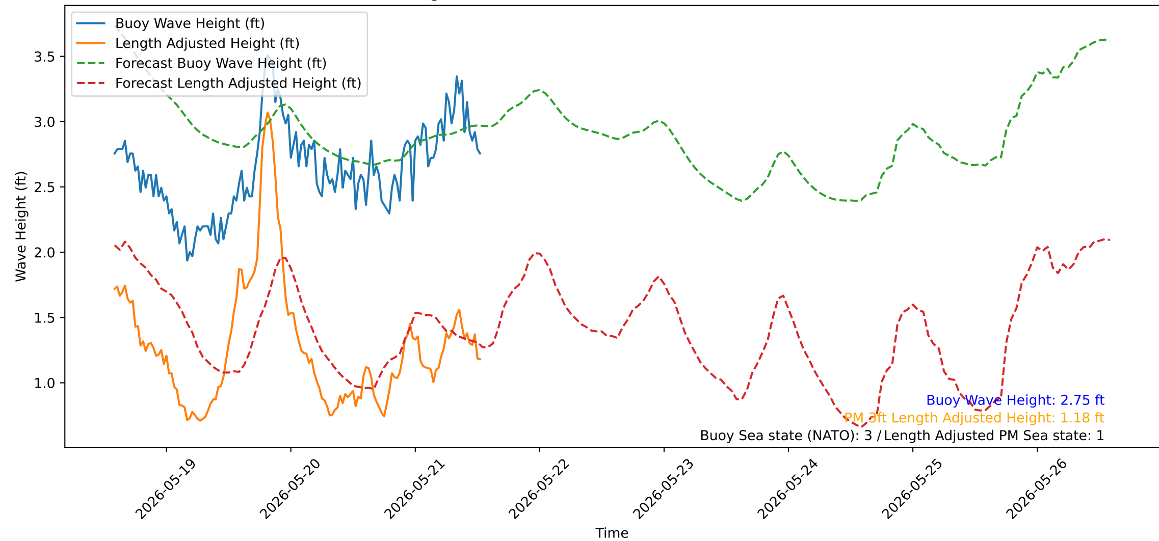
Wave Heights over Time for Red Beach at 2026-05-21 13:30:51
