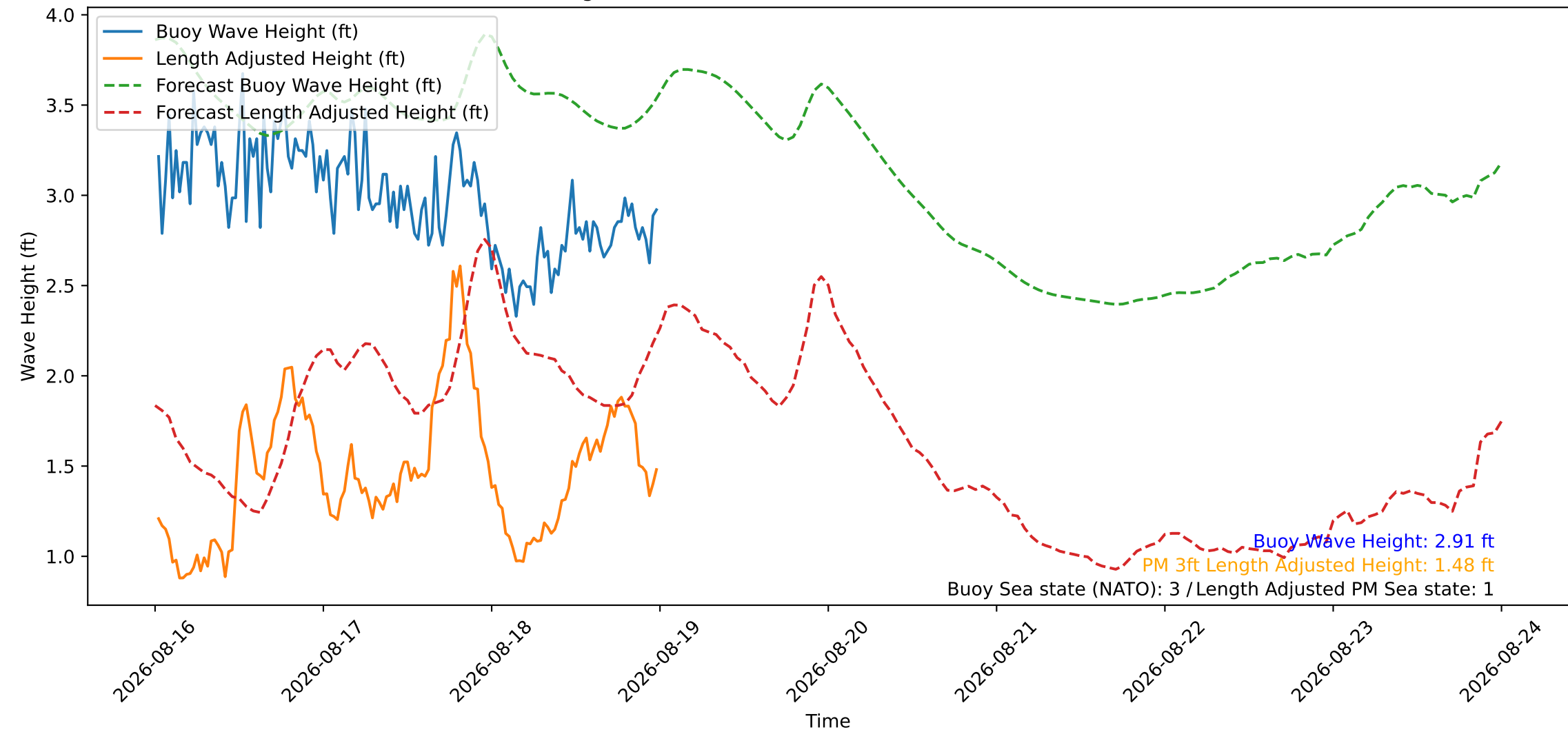
Wave Heights over Time for Red Beach at 2026-08-19 00:20:47
