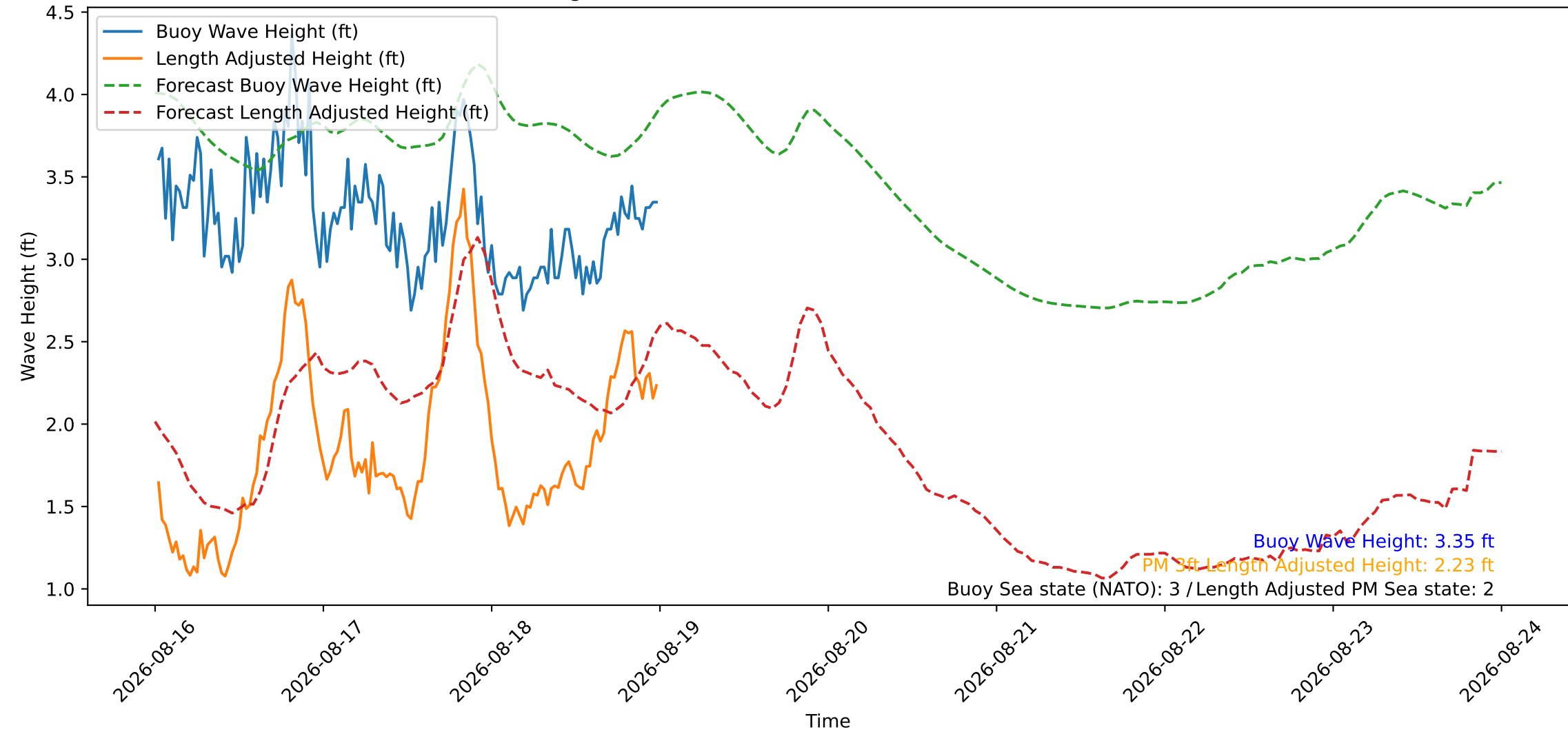
Wave Heights over Time for Green Beach at 2026-08-19 00:21:10
