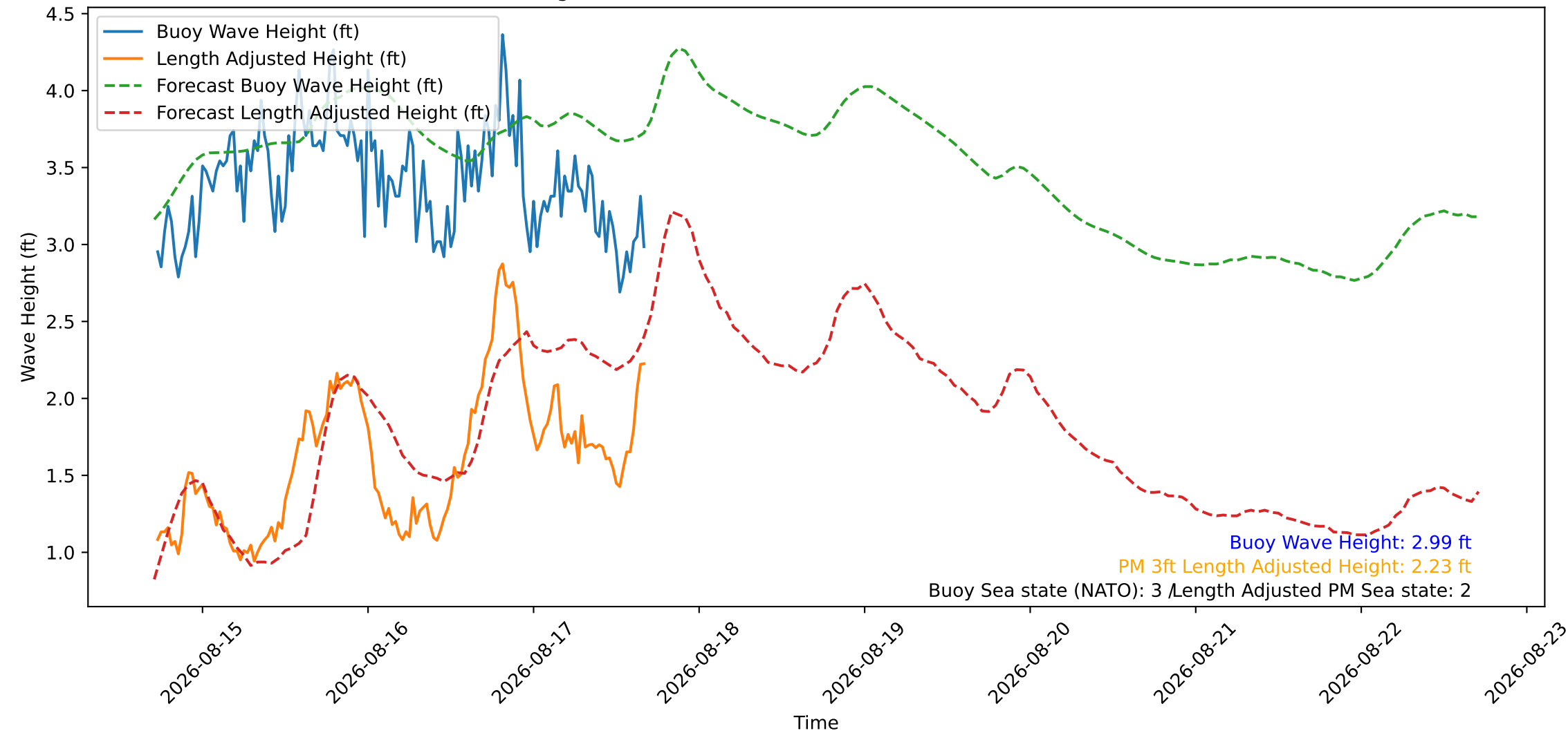
Wave Heights over Time for Green Beach at 2026-08-17 17:01:08
