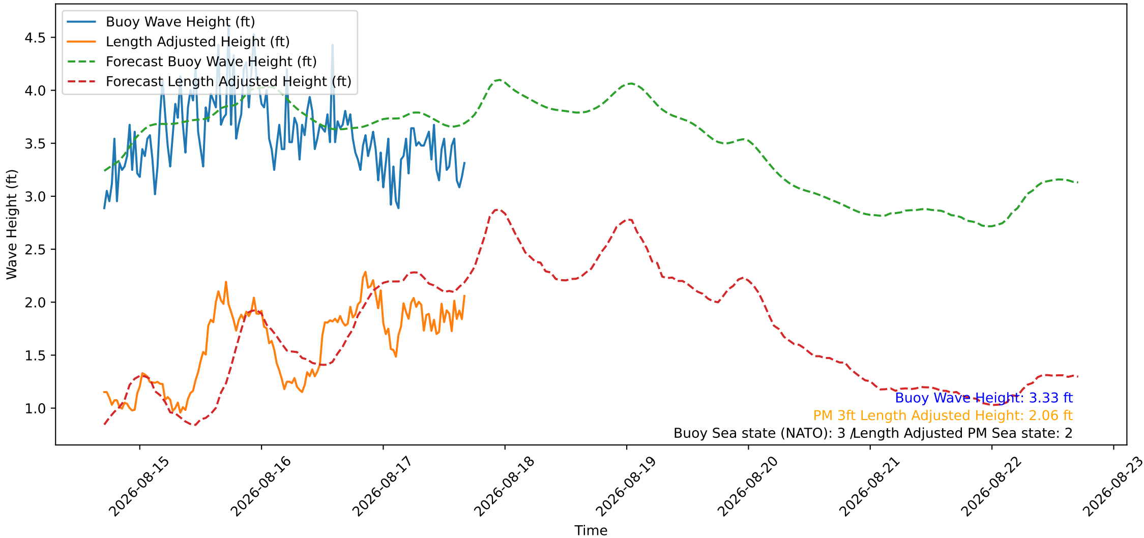
Wave Heights over Time for Oceanside Harbor at 2026-08-17 17:00:26
