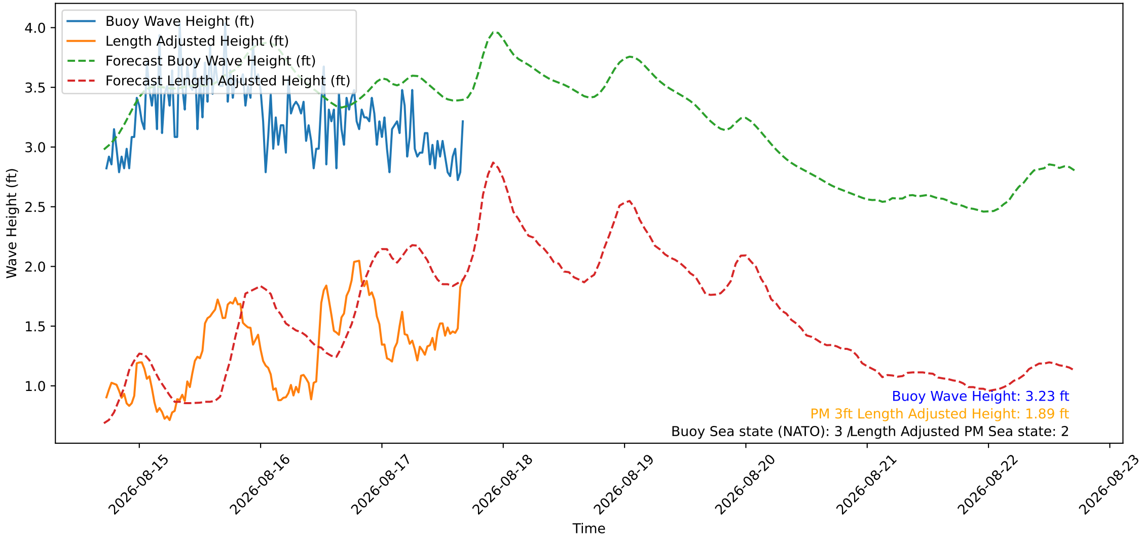
Wave Heights over Time for Red Beach at 2026-08-17 17:00:46
