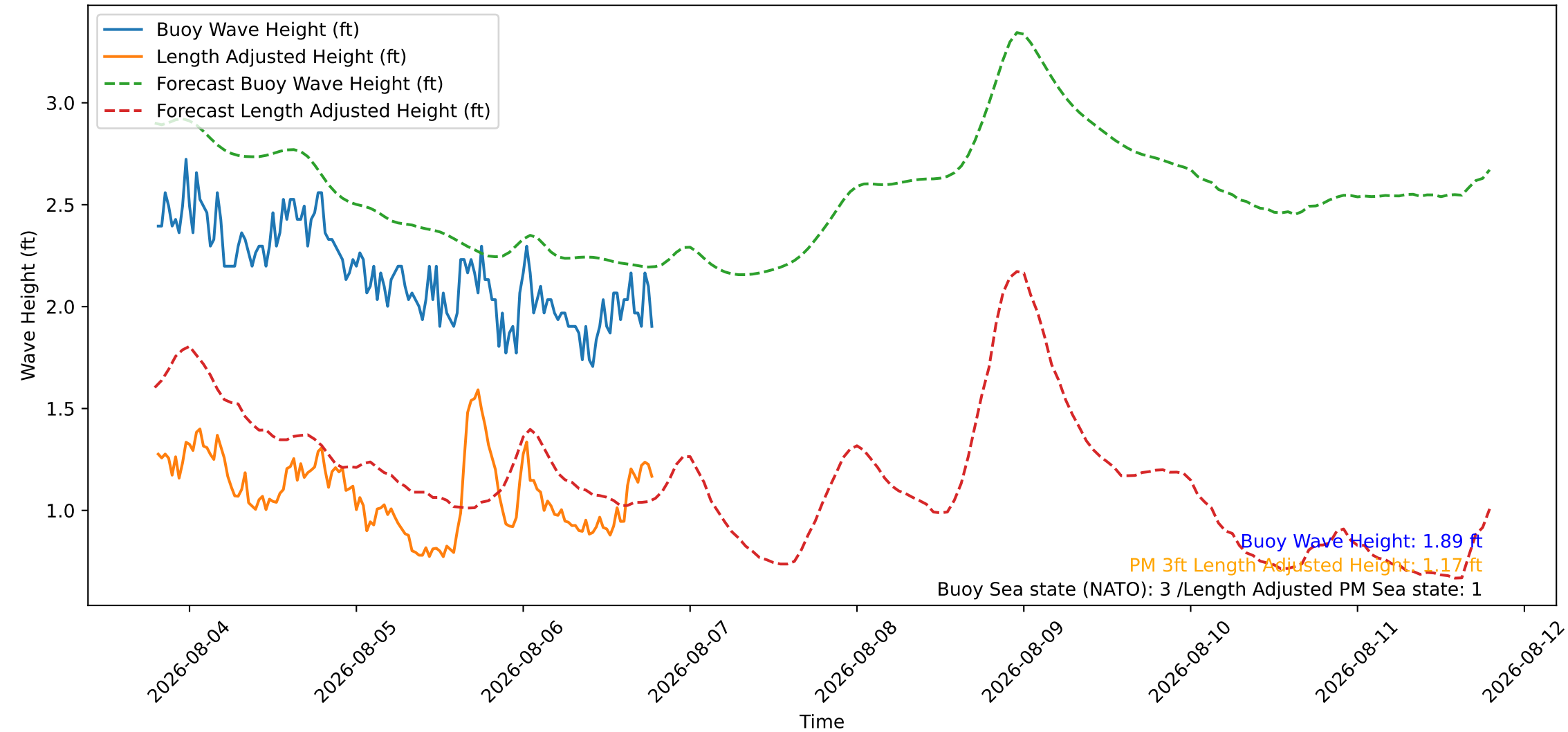
Wave Heights over Time for Oceanside Harbor at 2026-08-06 19:20:26
