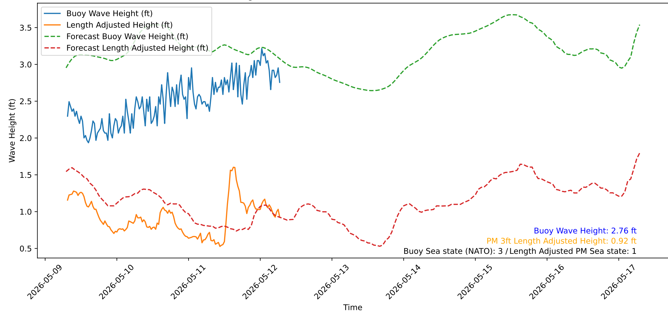
Wave Heights over Time for Red Beach at 2026-05-12 07:10:51
