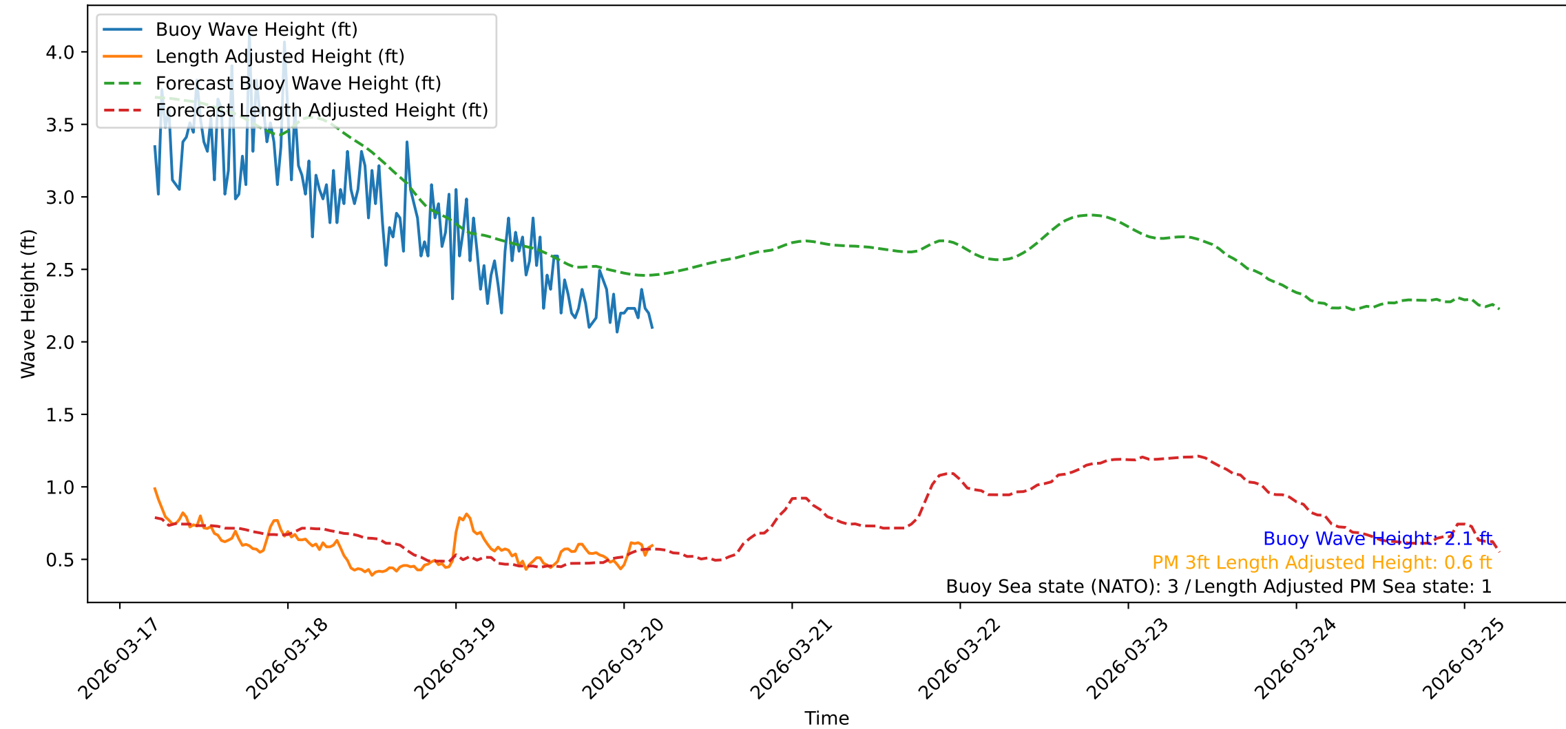
Wave Heights over Time for Green Beach at 2026-03-20 04:51:11
