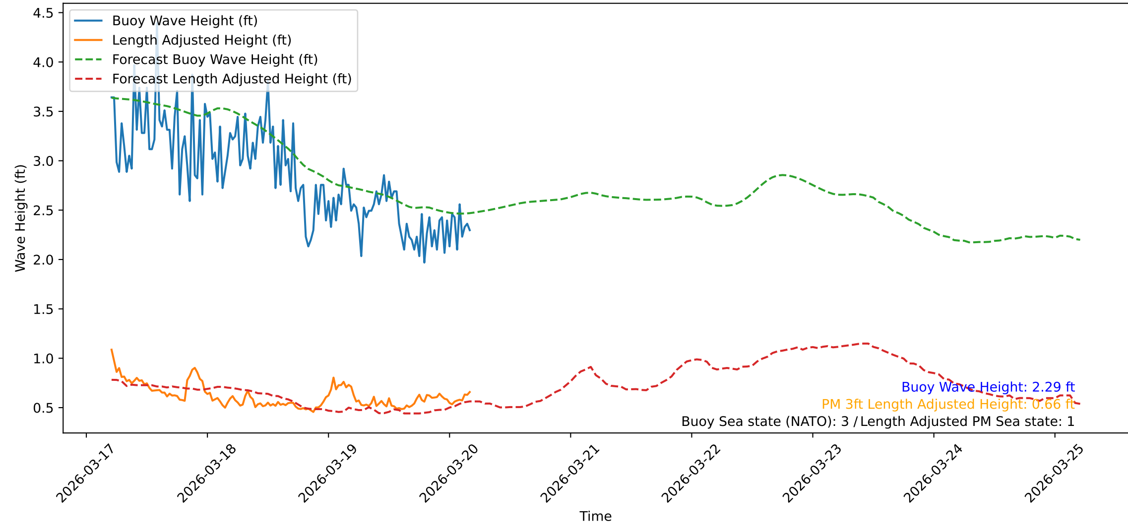
Wave Heights over Time for Oceanside Harbor at 2026-03-20 04:50:32
