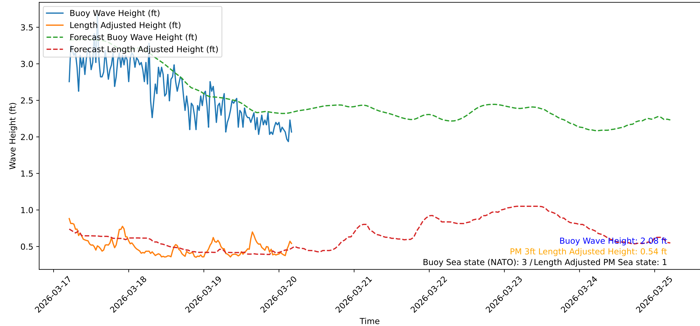
Wave Heights over Time for Red Beach at 2026-03-20 04:50:48
