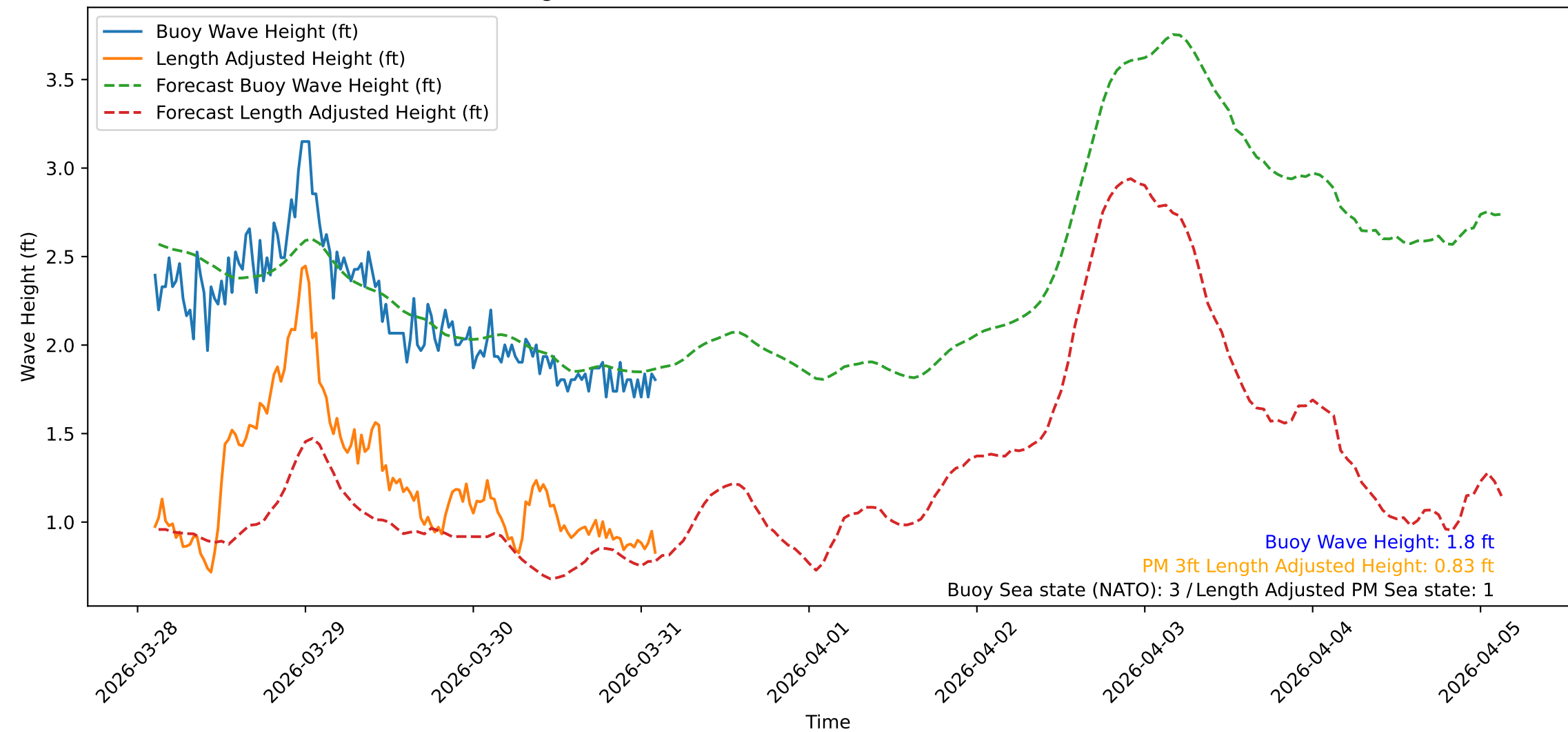
Wave Heights over Time for Oceanside Harbor at 2026-03-31 02:40:31
