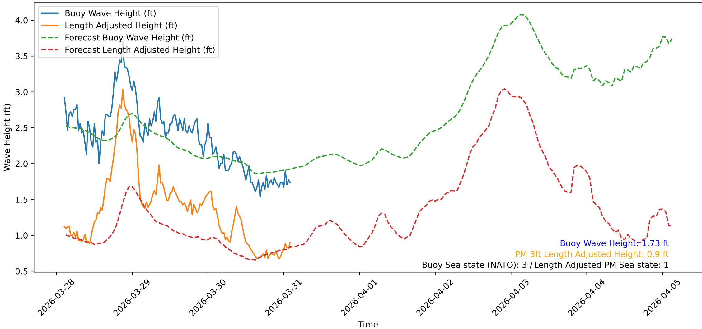
Wave Heights over Time for Green Beach at 2026-03-31 02:41:09
