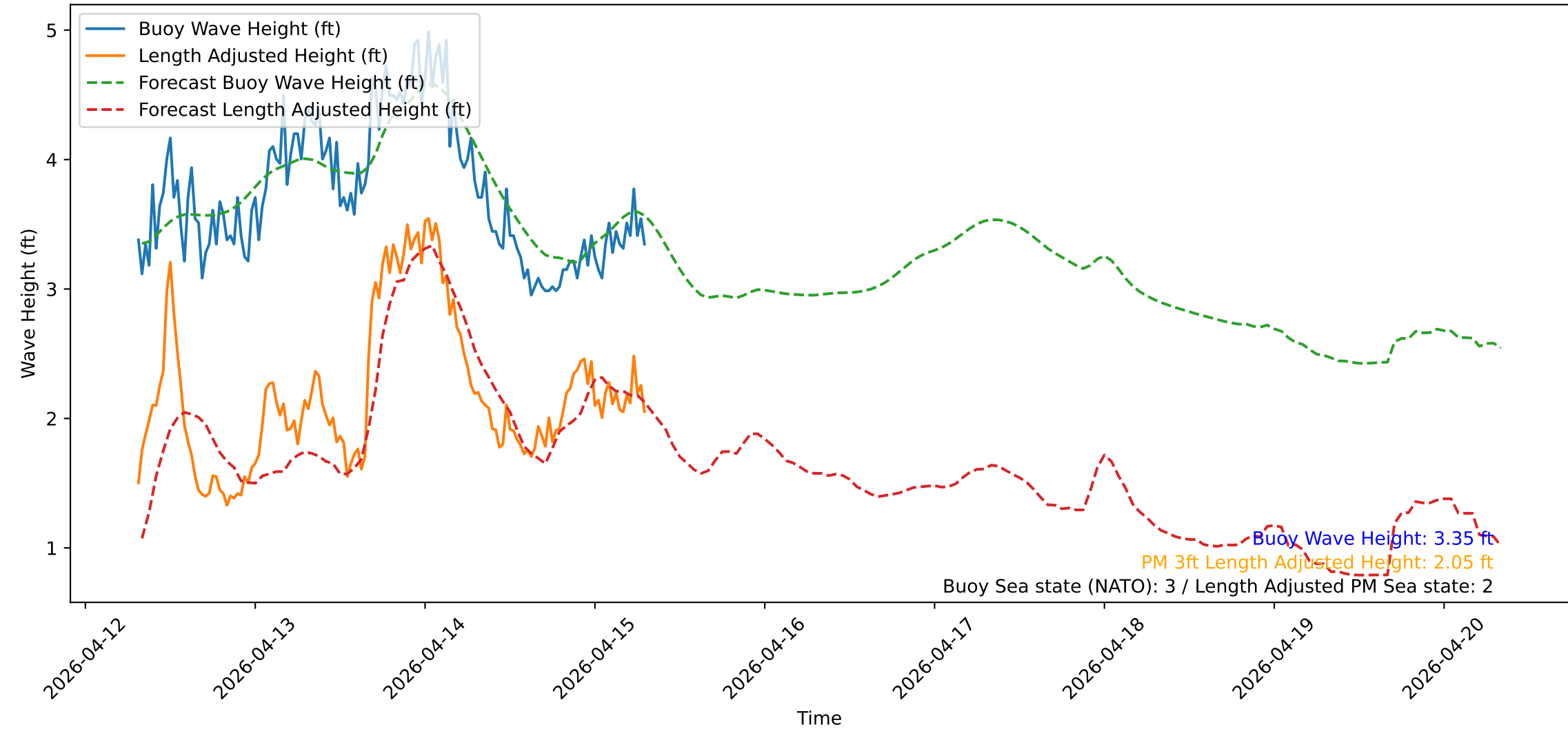
Wave Heights over Time for Green Beach at 2026-04-15 07:41:13
