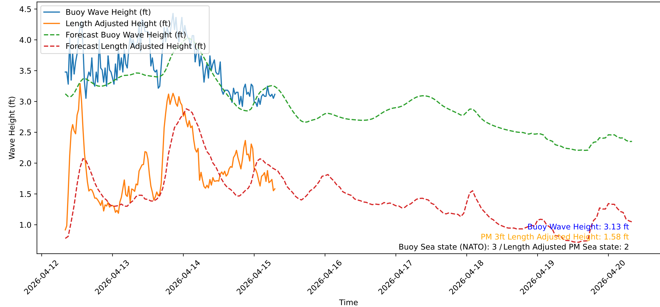
Wave Heights over Time for Red Beach at 2026-04-15 07:40:50
