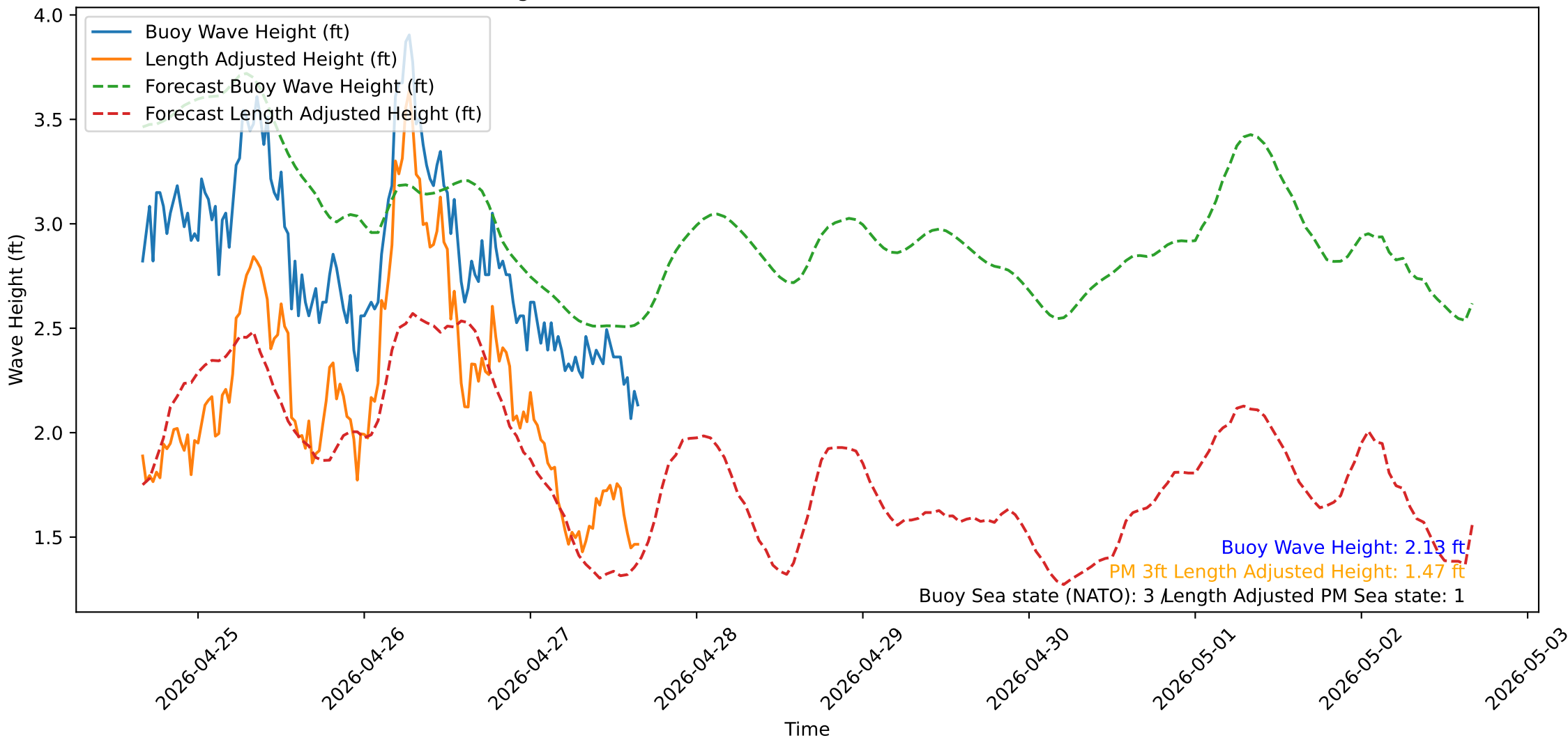
Wave Heights over Time for Oceanside Harbor at 2026-04-27 16:10:31
