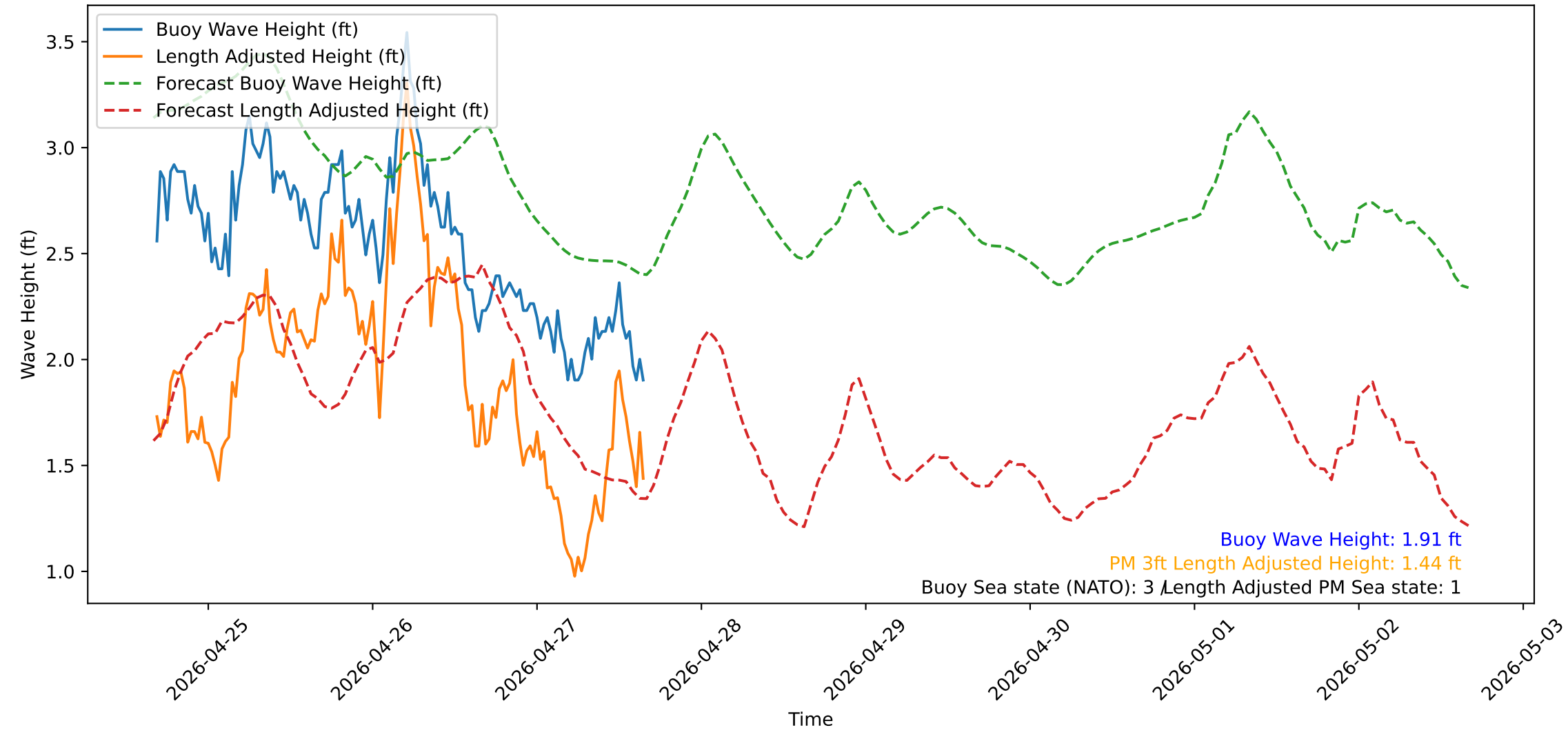
Wave Heights over Time for Red Beach at 2026-04-27 16:10:49
