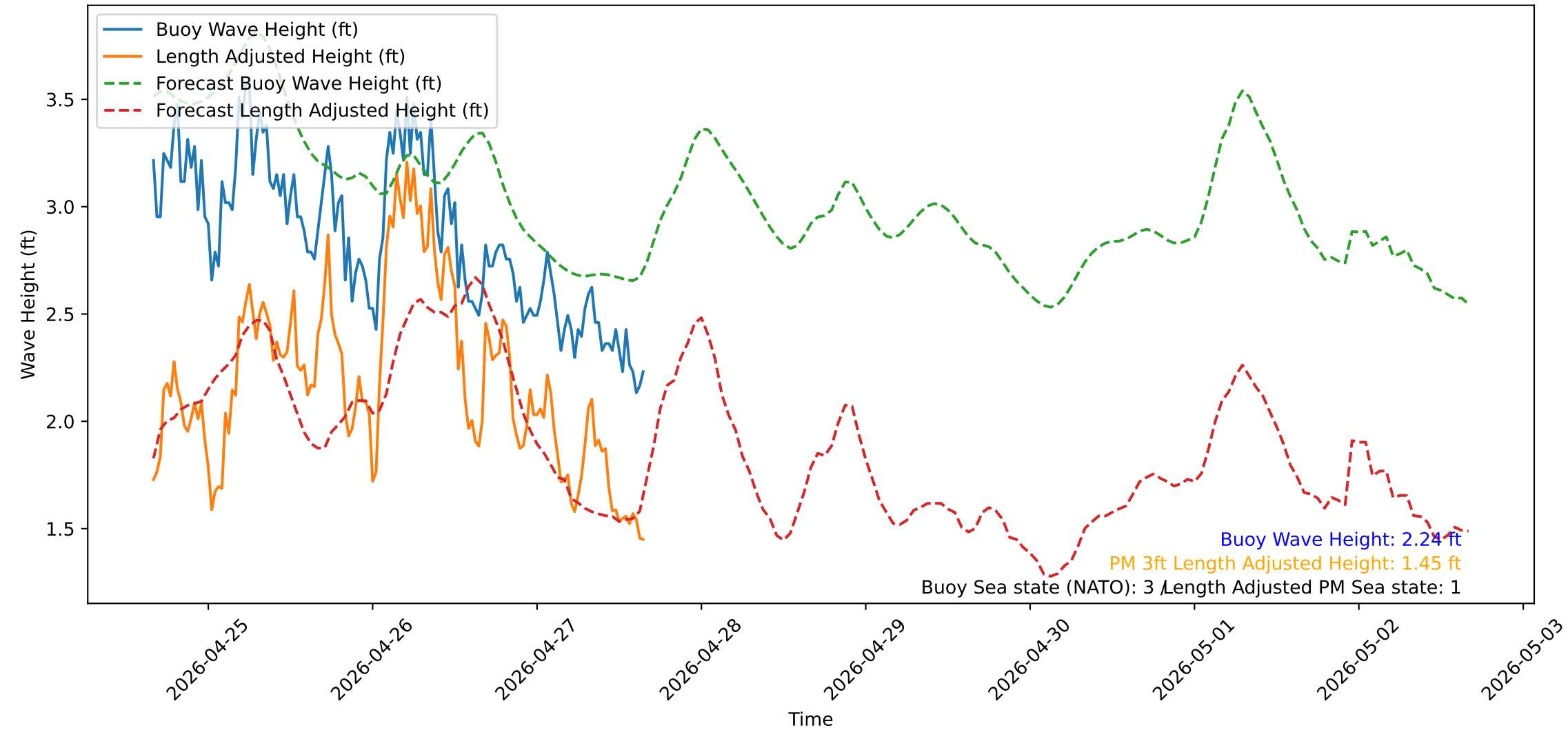
Wave Heights over Time for Green Beach at 2026-04-27 16:11:11
