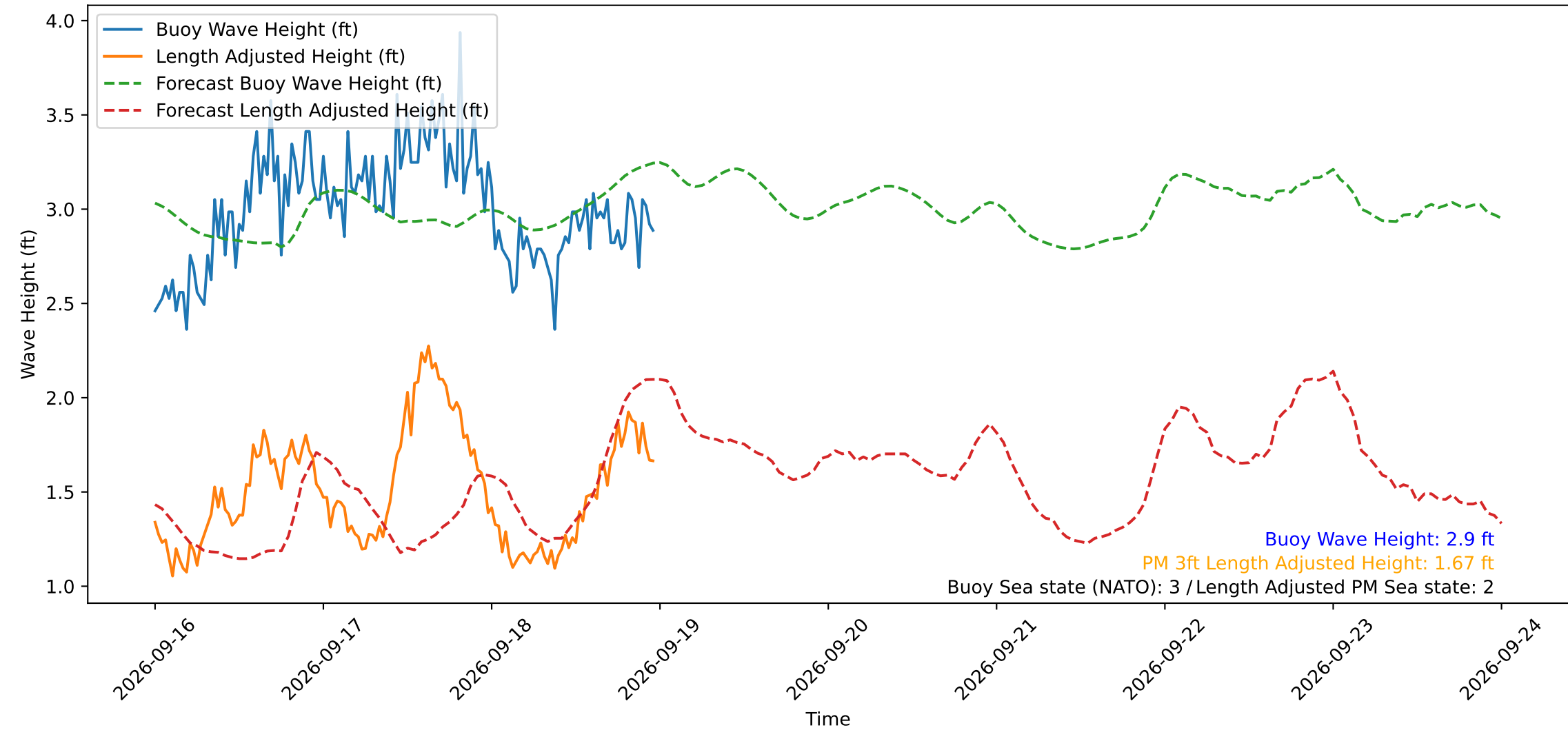
Wave Heights over Time for Oceanside Harbor at 2026-09-19 00:00:29
