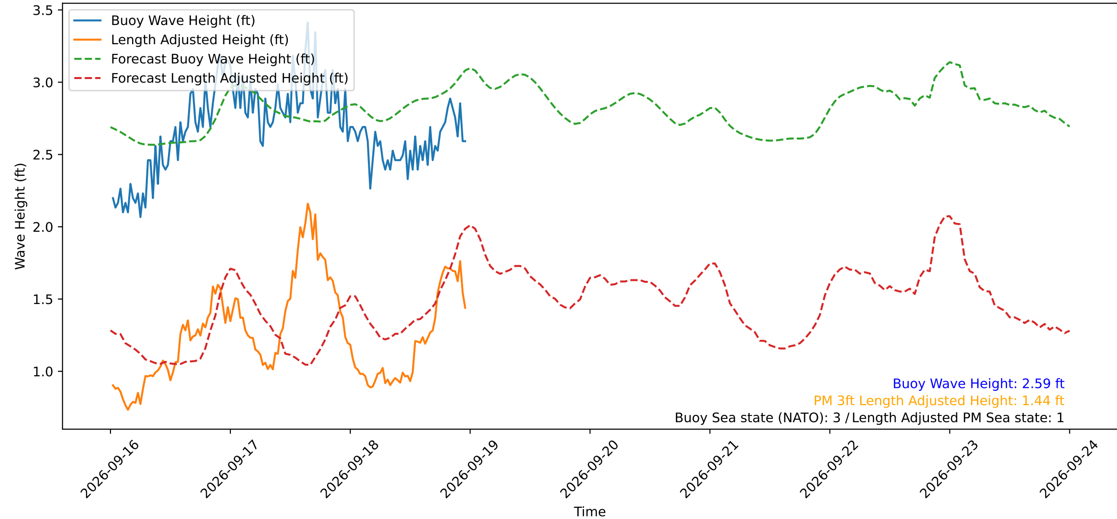
Wave Heights over Time for Red Beach at 2026-09-19 00:00:49
