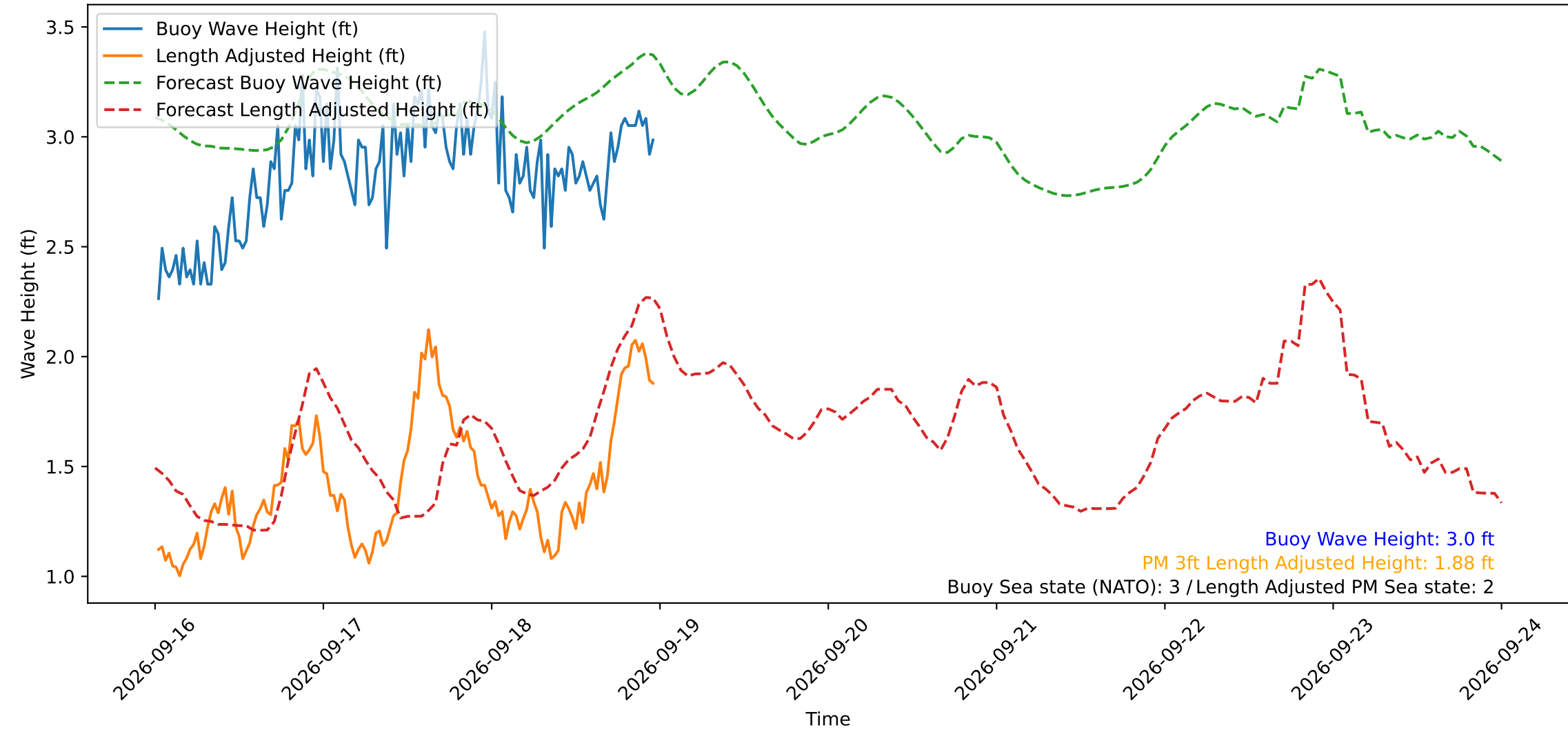
Wave Heights over Time for Green Beach at 2026-09-19 00:01:11
