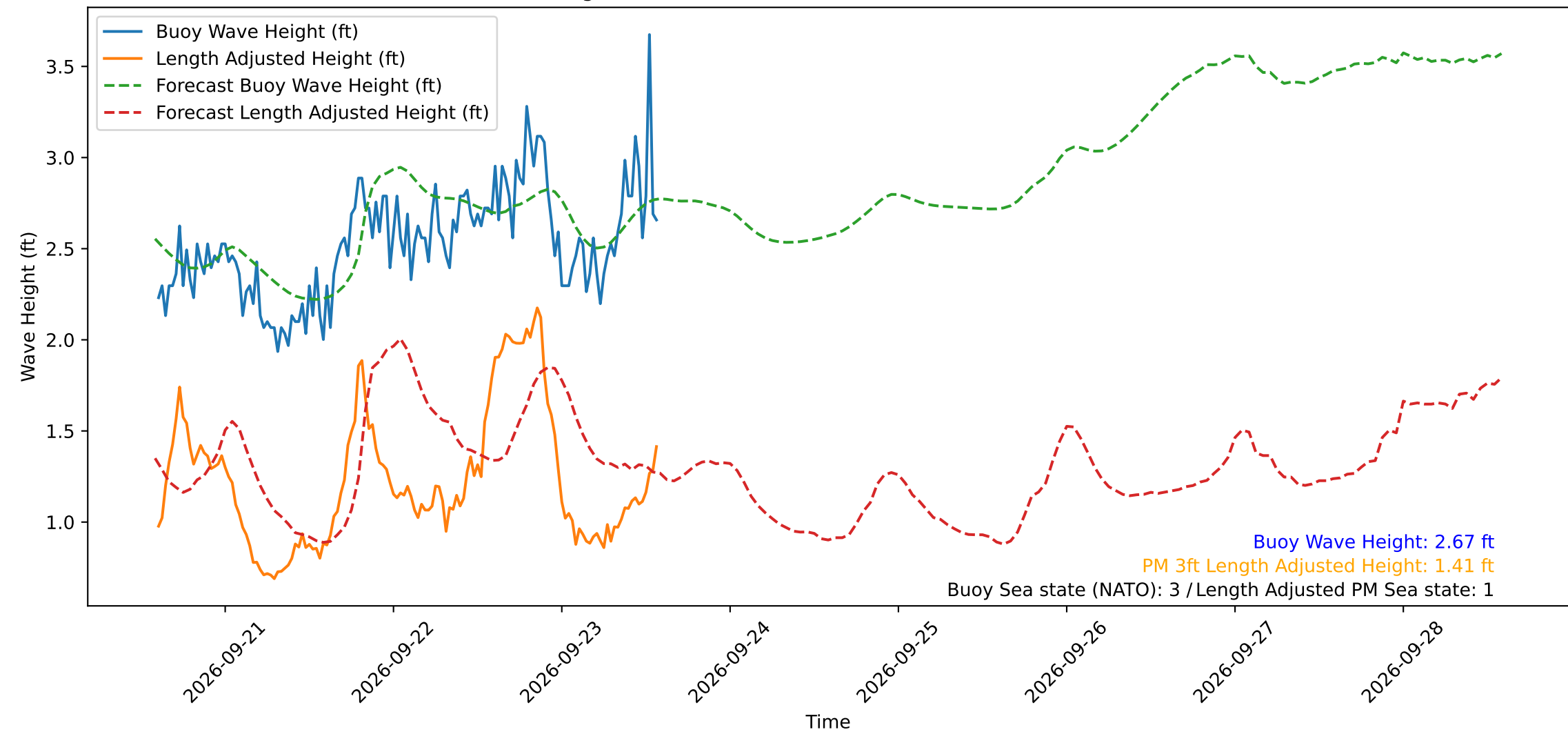
Wave Heights over Time for Red Beach at 2026-09-23 14:10:50
