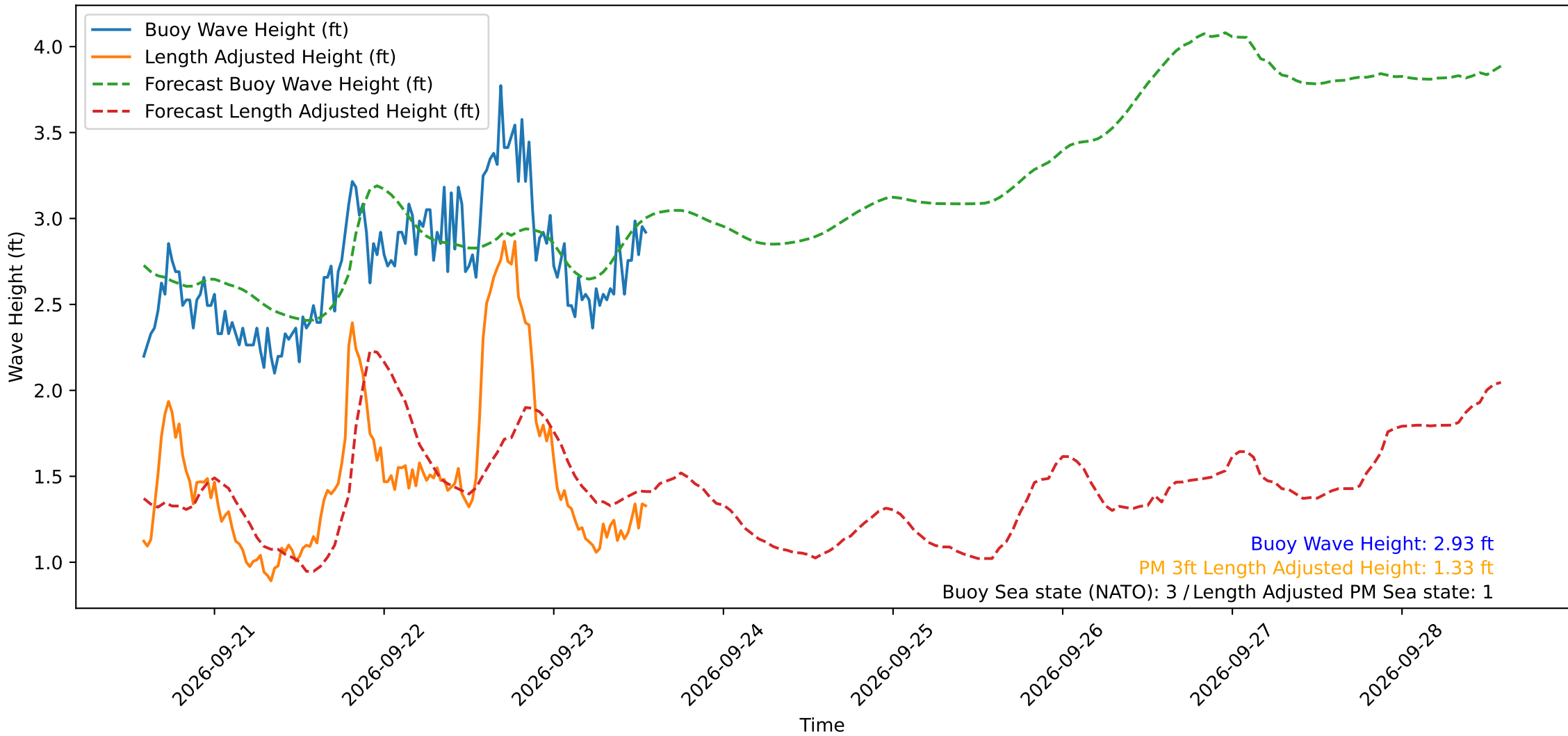
Wave Heights over Time for Oceanside Harbor at 2026-09-23 14:10:30
