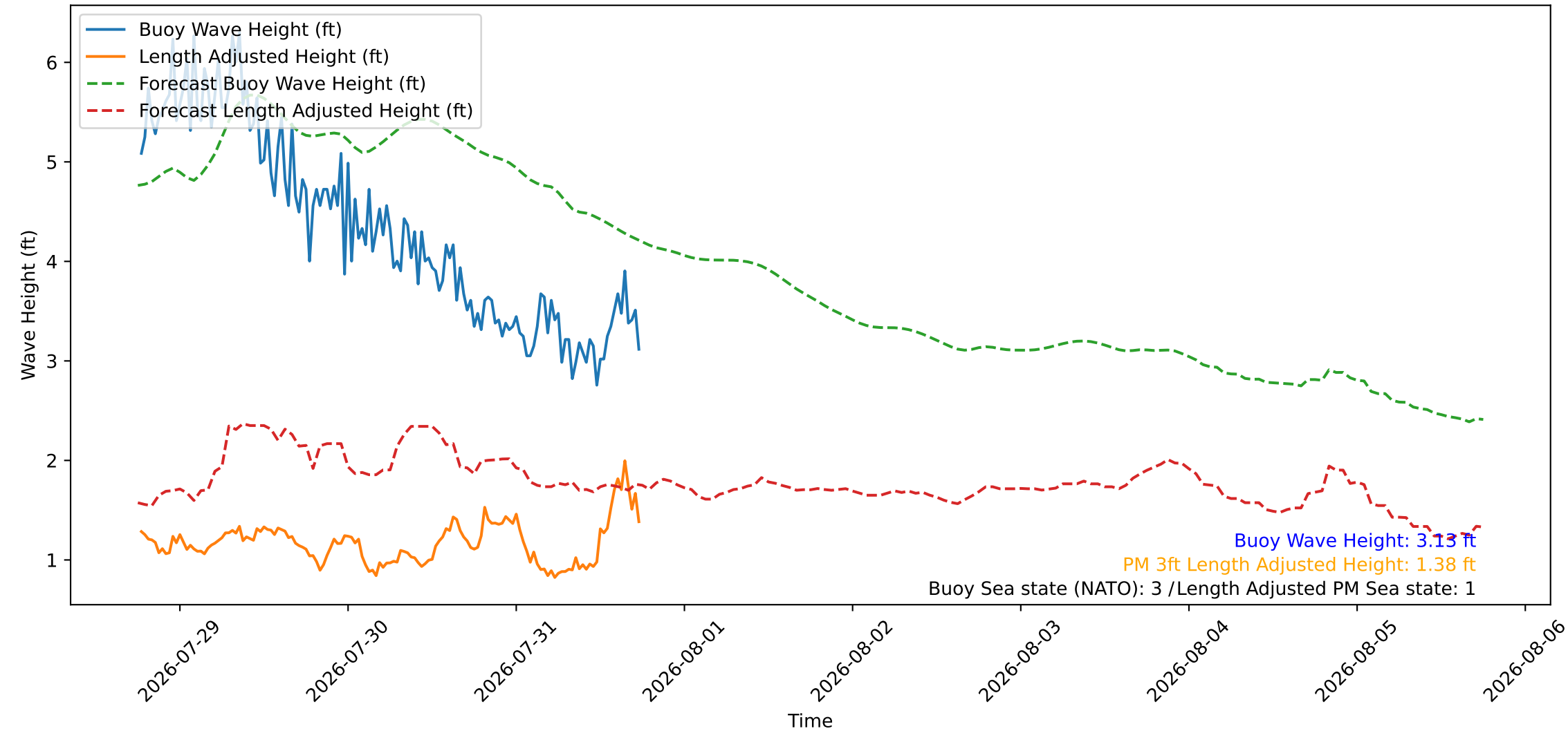
Wave Heights over Time for Green Beach at 2026-07-31 18:21:10
