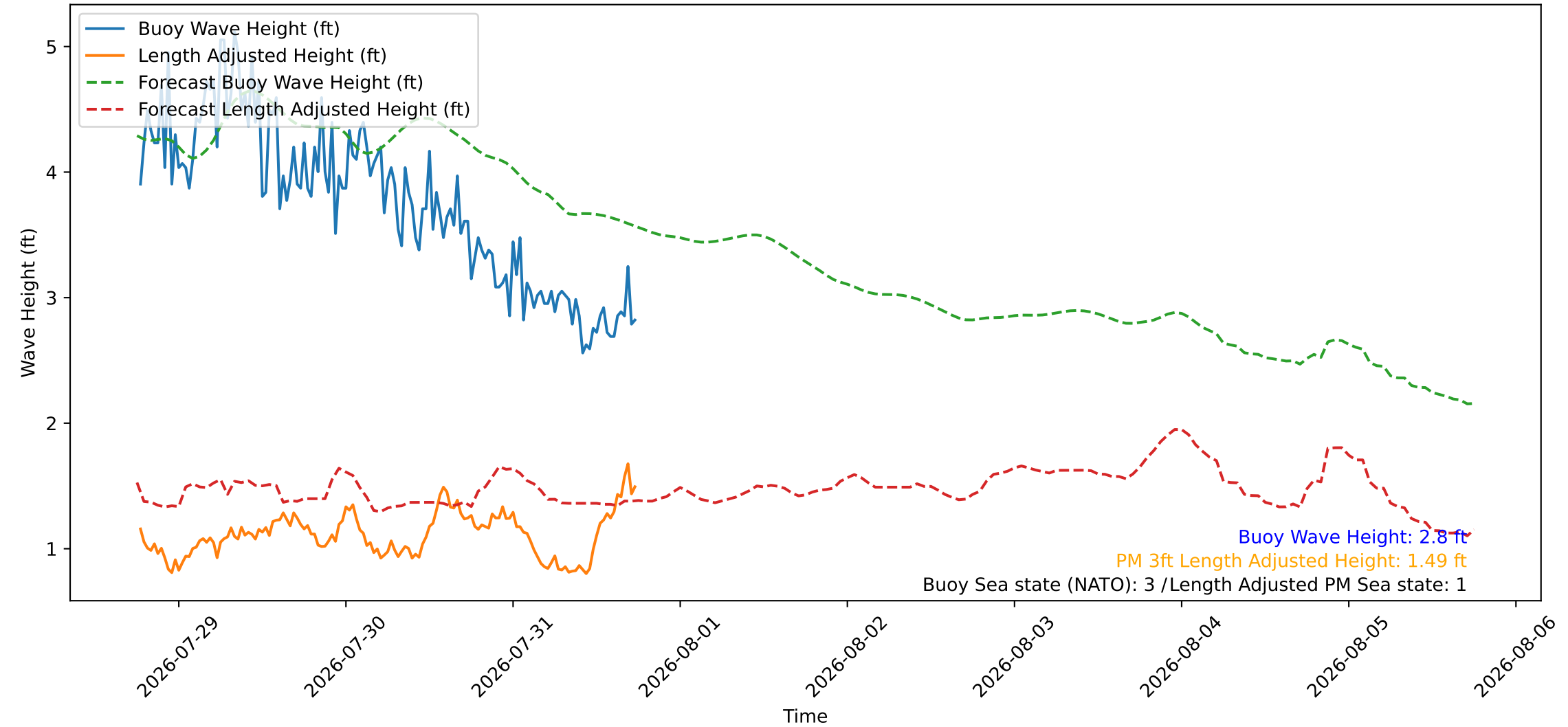
Wave Heights over Time for Red Beach at 2026-07-31 18:20:47
