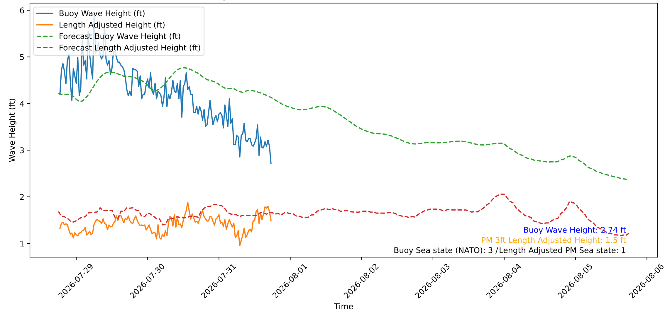
Wave Heights over Time for Oceanside Harbor at 2026-07-31 18:20:26
