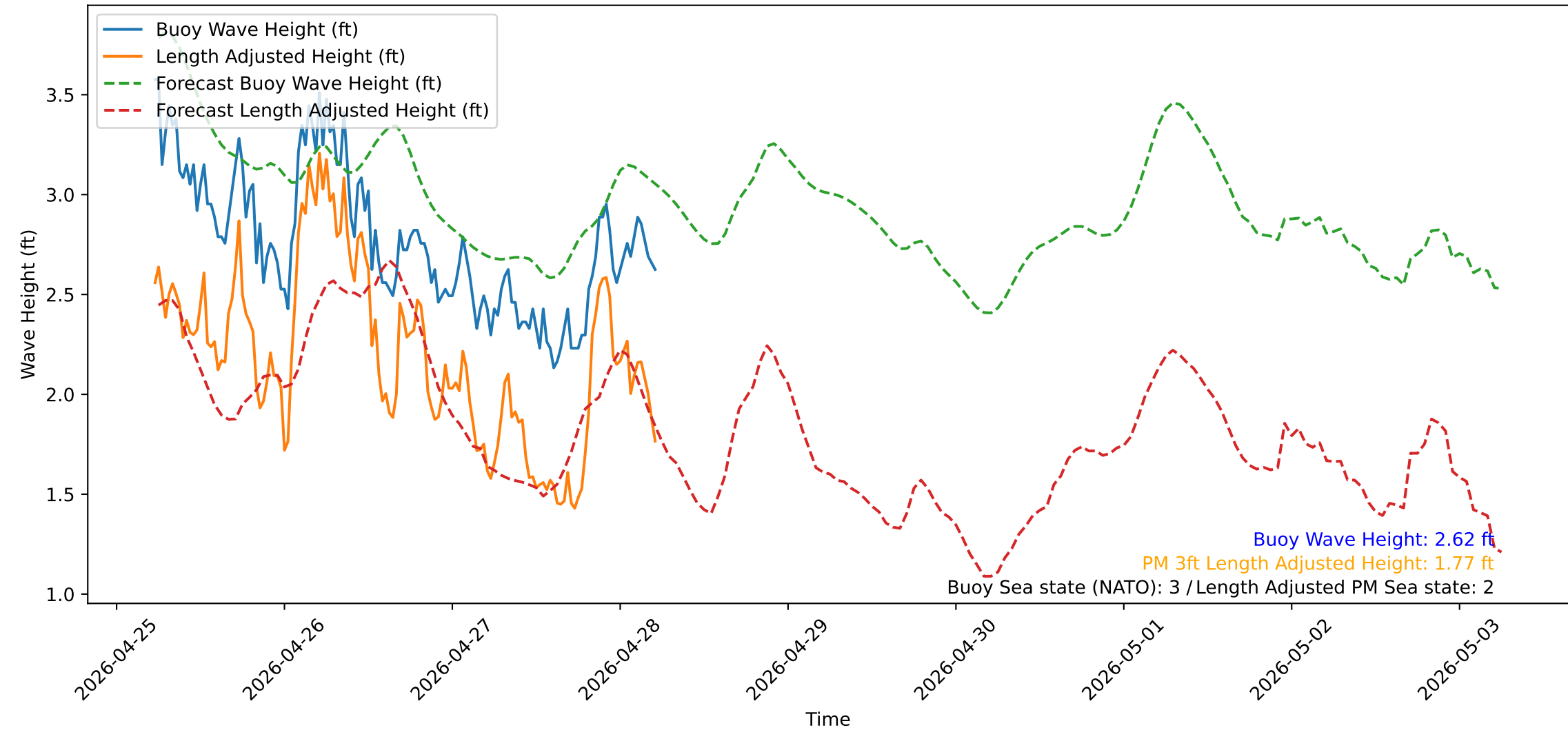
Wave Heights over Time for Green Beach at 2026-04-28 05:41:13
