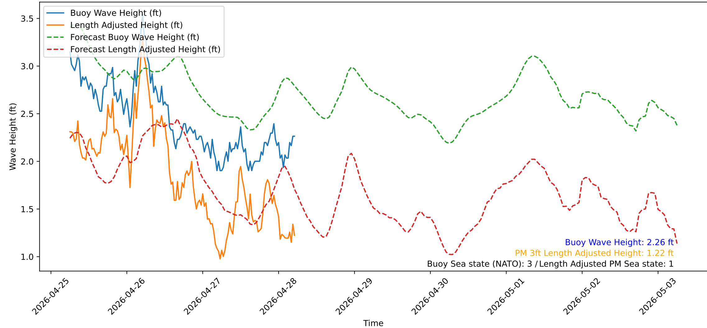
Wave Heights over Time for Red Beach at 2026-04-28 05:40:51
