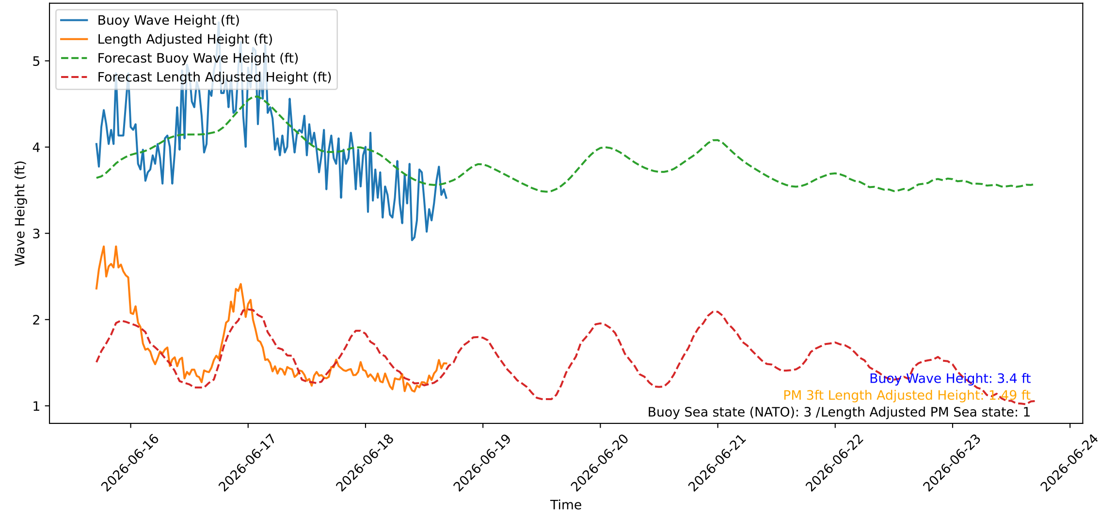
Wave Heights over Time for Oceanside Harbor at 2026-06-18 17:10:26
