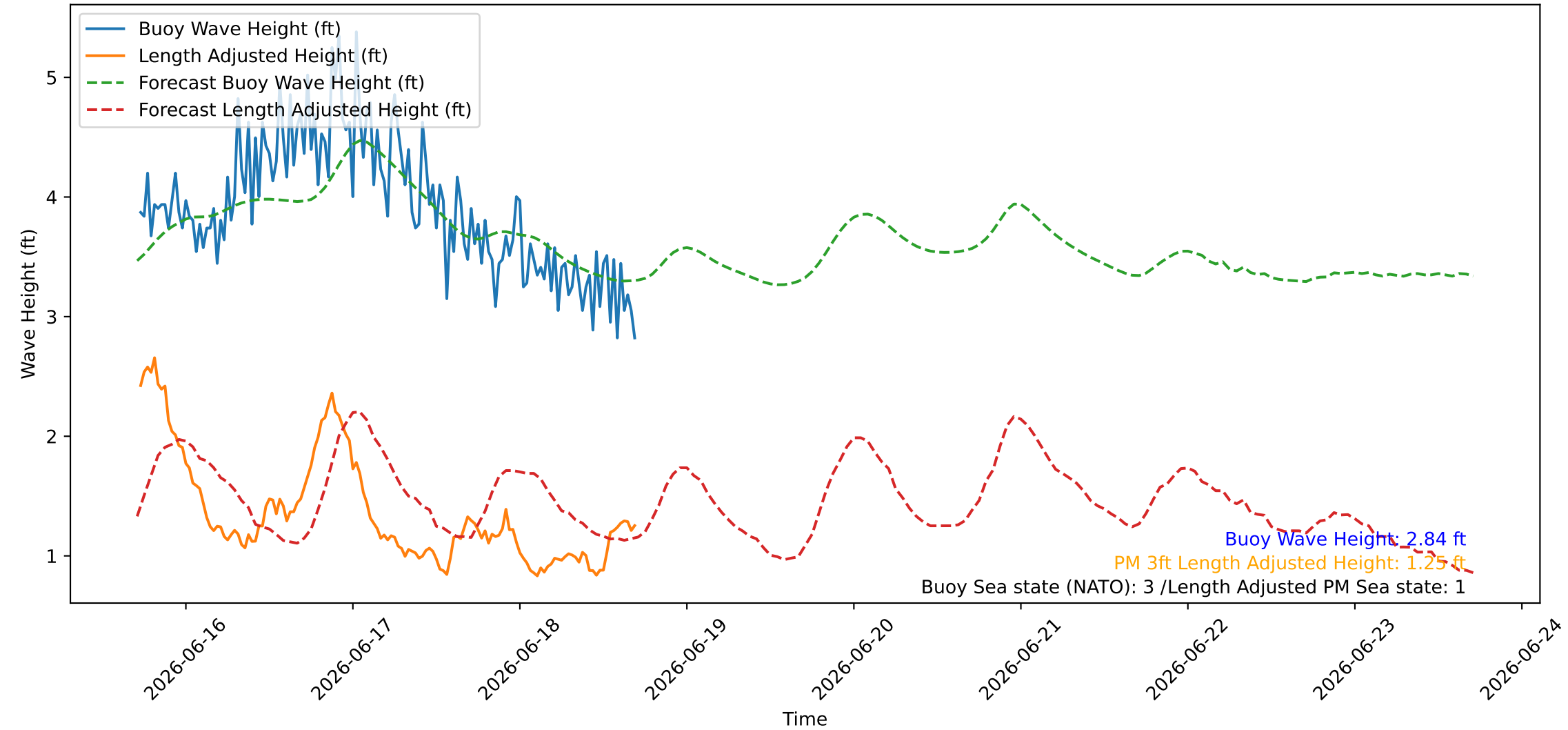
Wave Heights over Time for Red Beach at 2026-06-18 17:10:45
