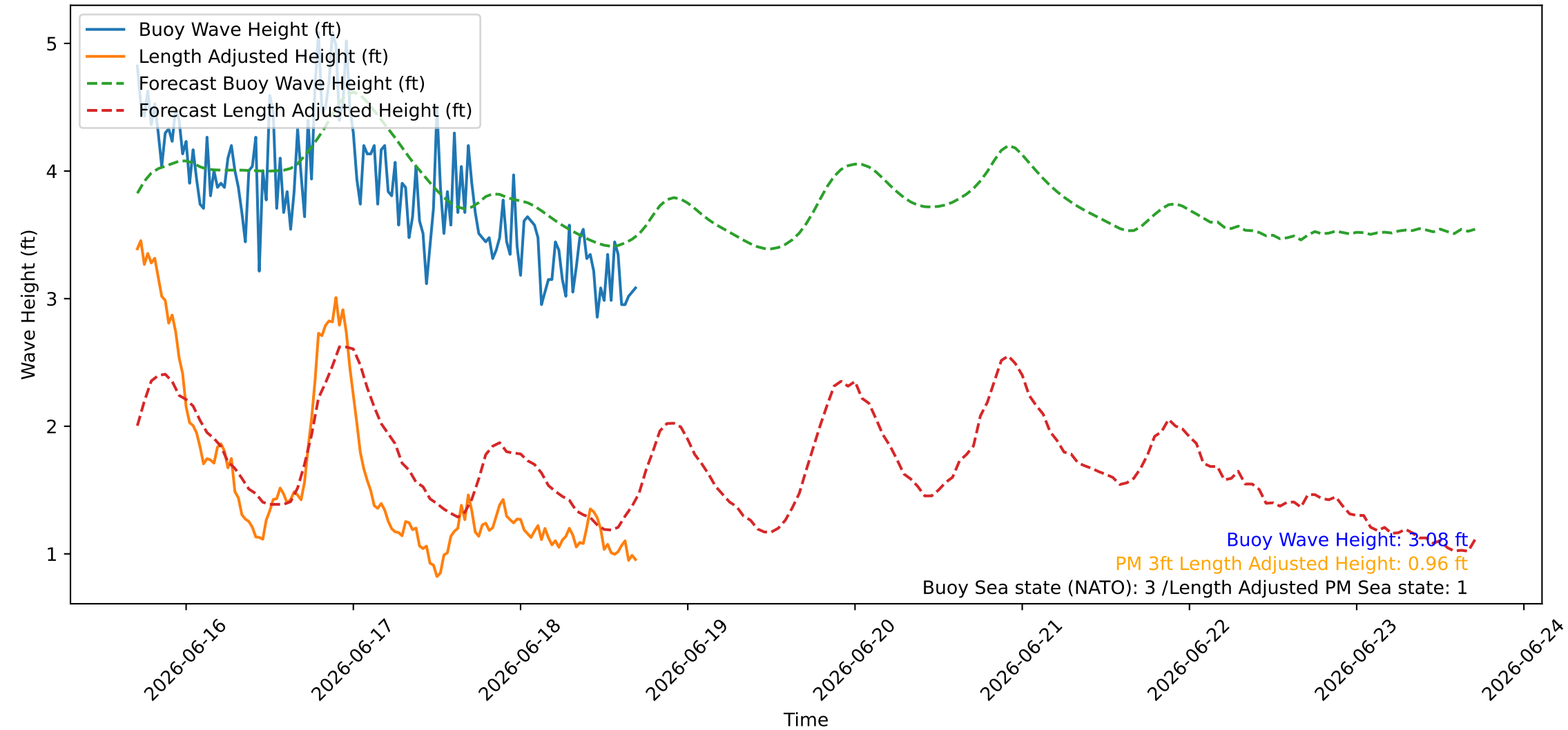
Wave Heights over Time for Green Beach at 2026-06-18 17:11:08
