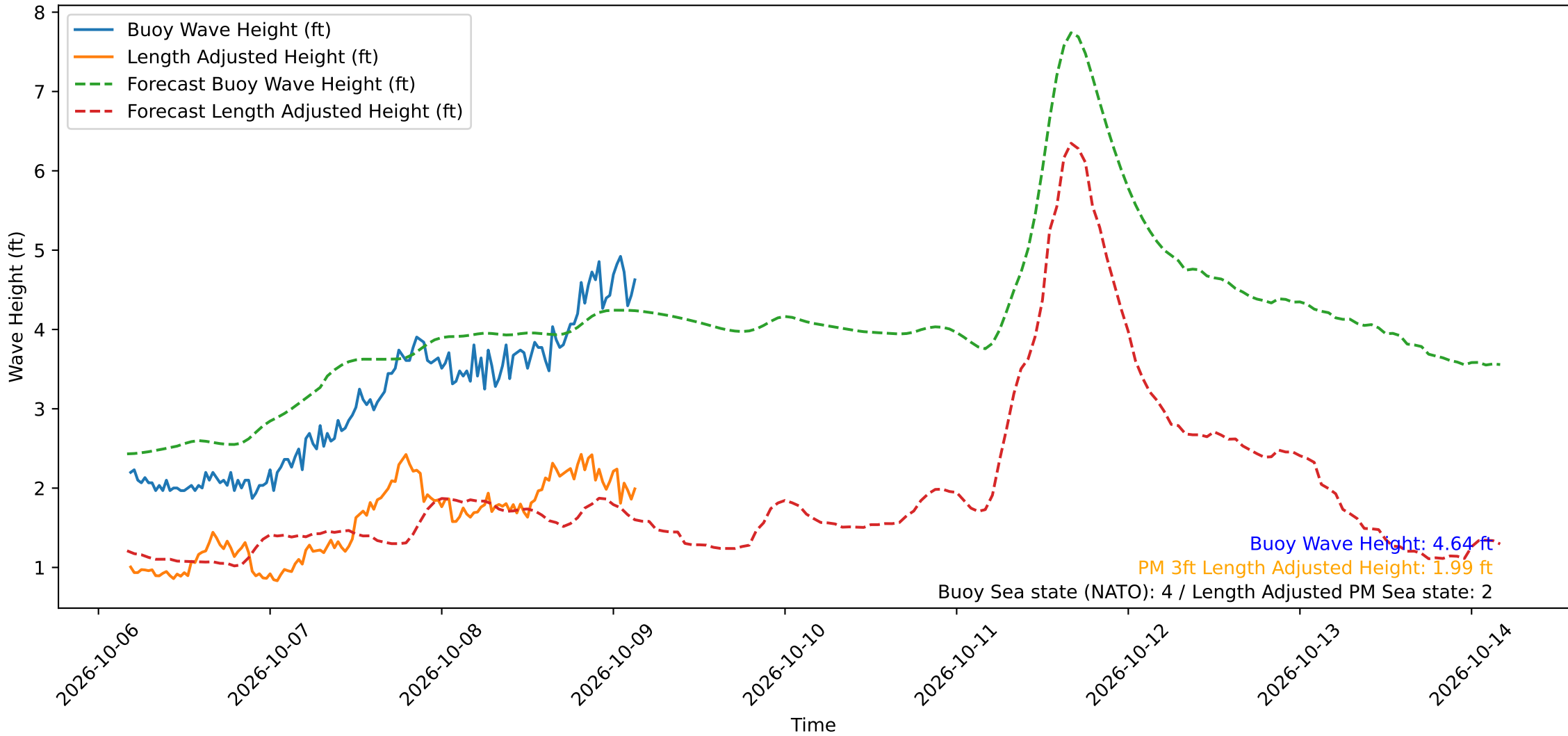
Wave Heights over Time for Red Beach at 2026-10-09 04:10:49
