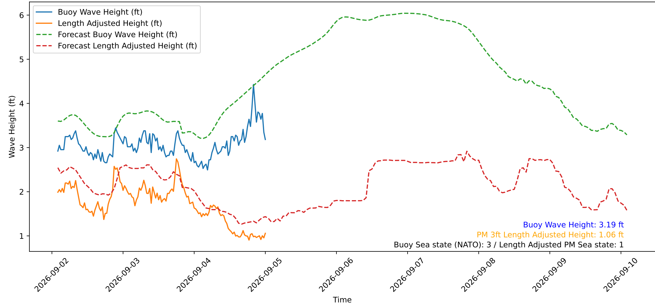
Wave Heights over Time for Green Beach at 2026-09-05 01:31:13
