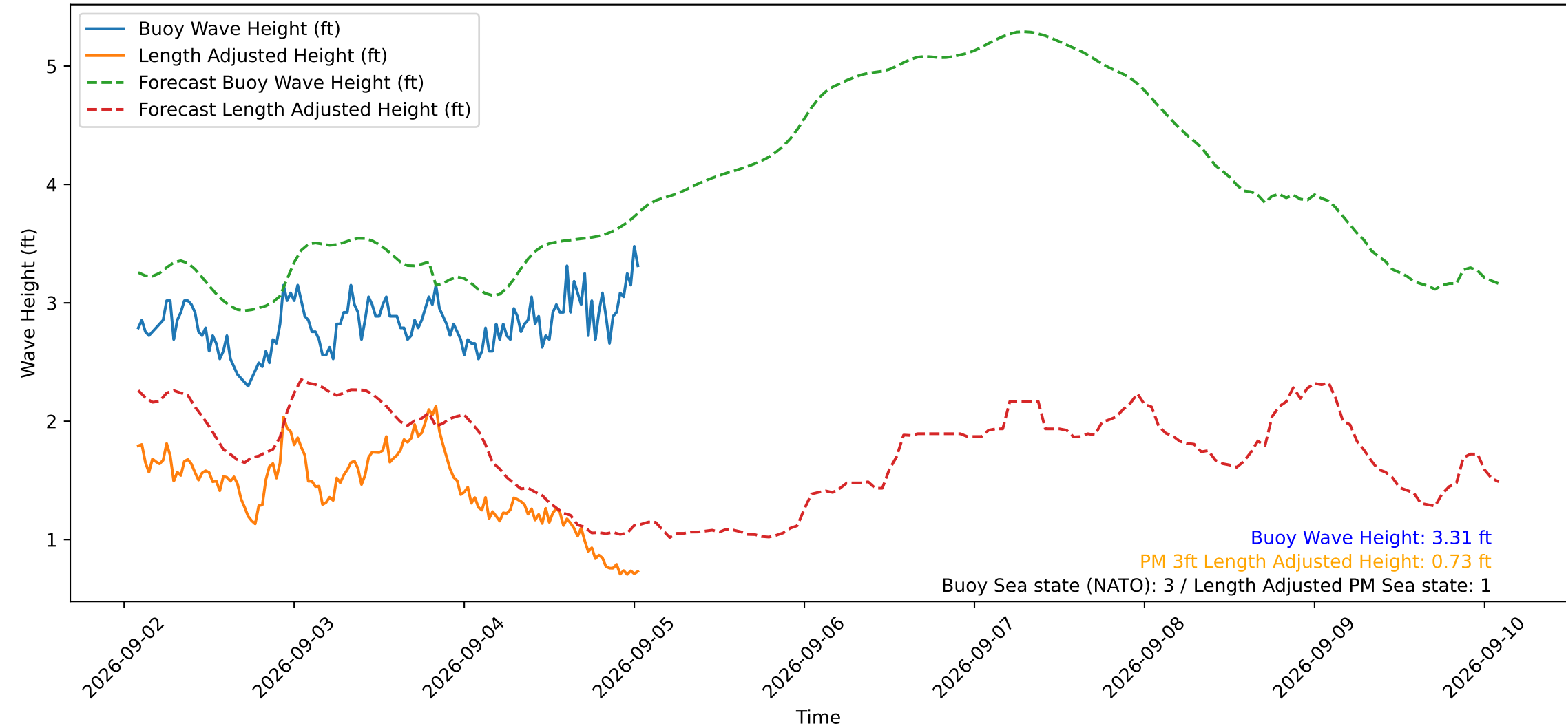
Wave Heights over Time for Red Beach at 2026-09-05 01:30:50
