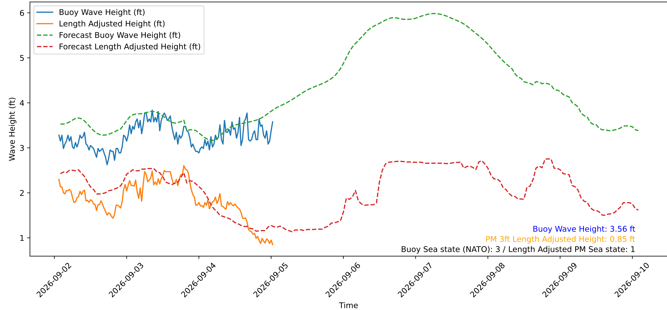
Wave Heights over Time for Oceanside Harbor at 2026-09-05 01:30:30
