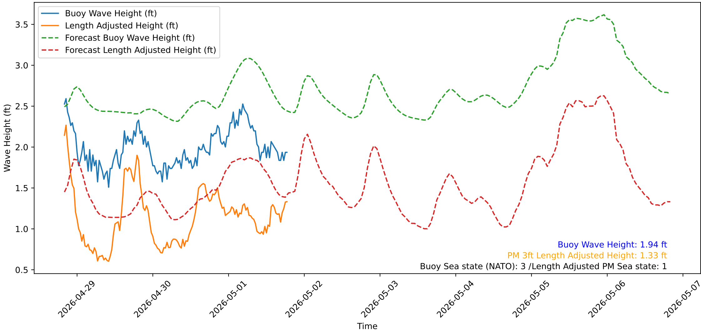
Wave Heights over Time for Red Beach at 2026-05-01 19:30:50
