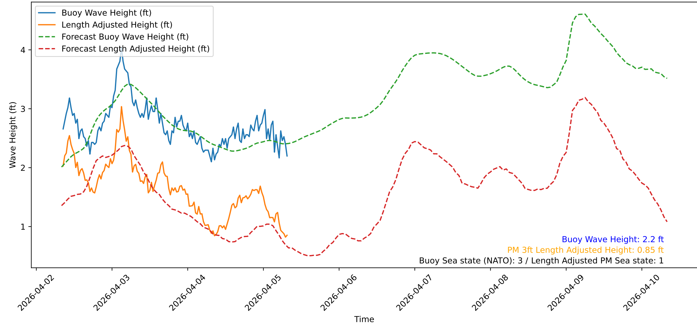
Wave Heights over Time for Oceanside Harbor at 2026-04-05 08:20:35
