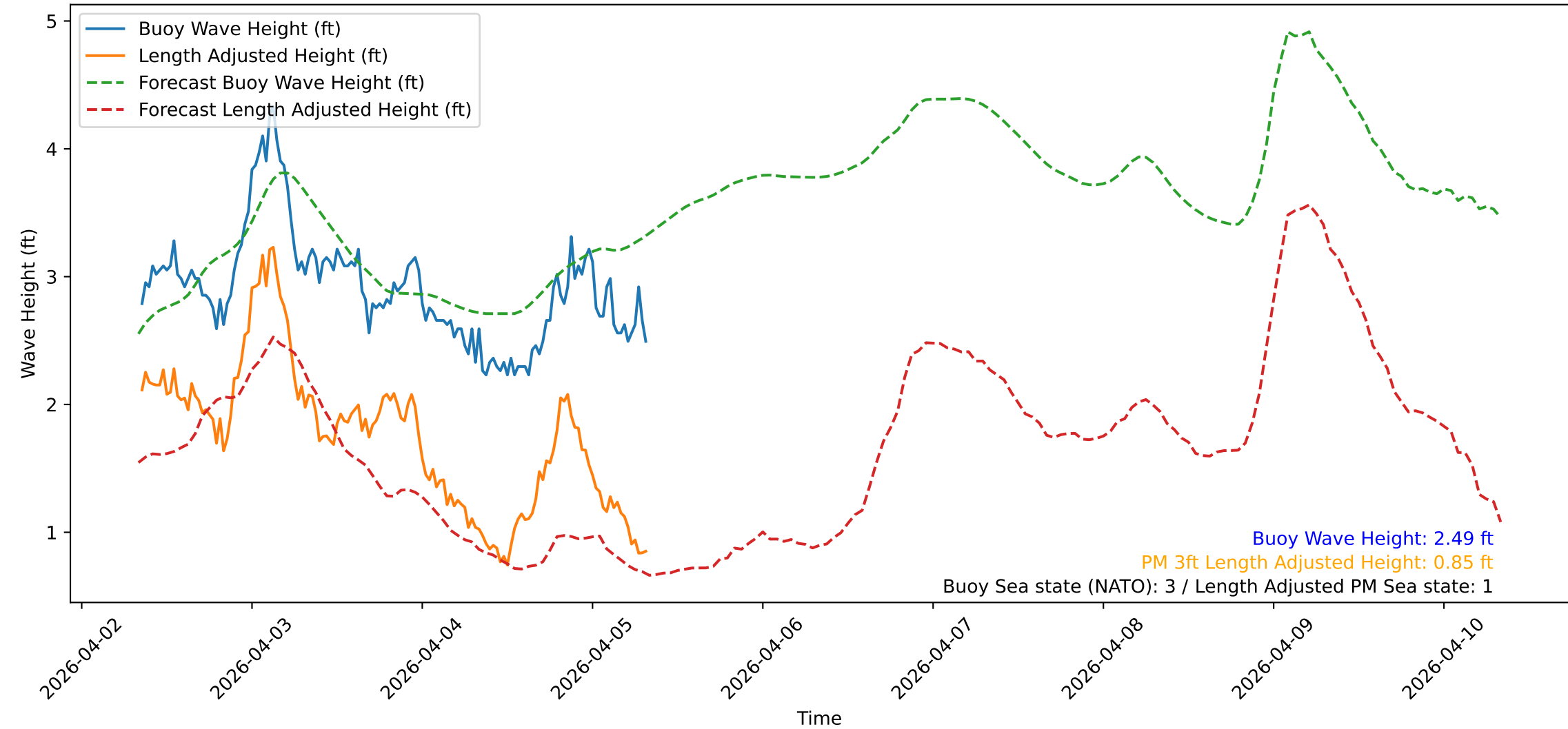
Wave Heights over Time for Green Beach at 2026-04-05 08:21:14
