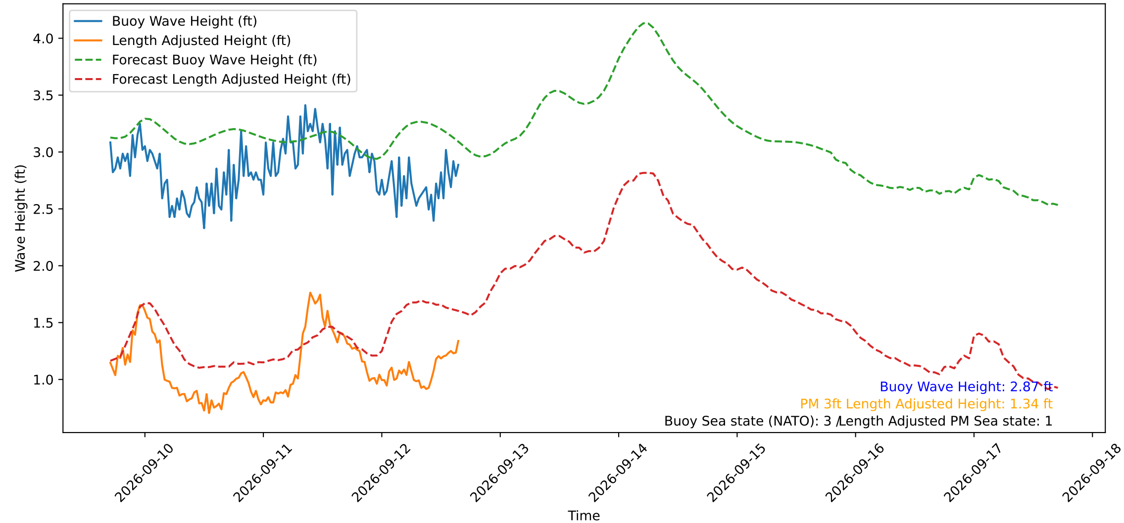
Wave Heights over Time for Red Beach at 2026-09-12 16:40:50
