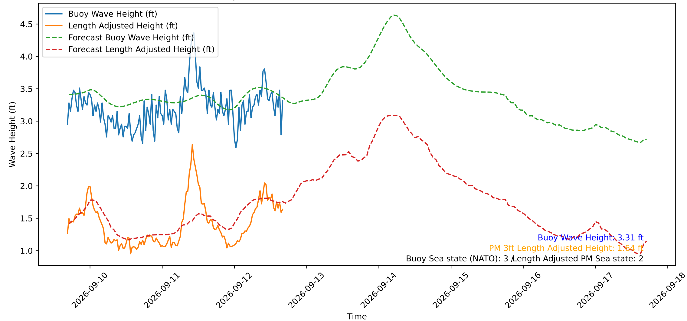
Wave Heights over Time for Oceanside Harbor at 2026-09-12 16:40:30
