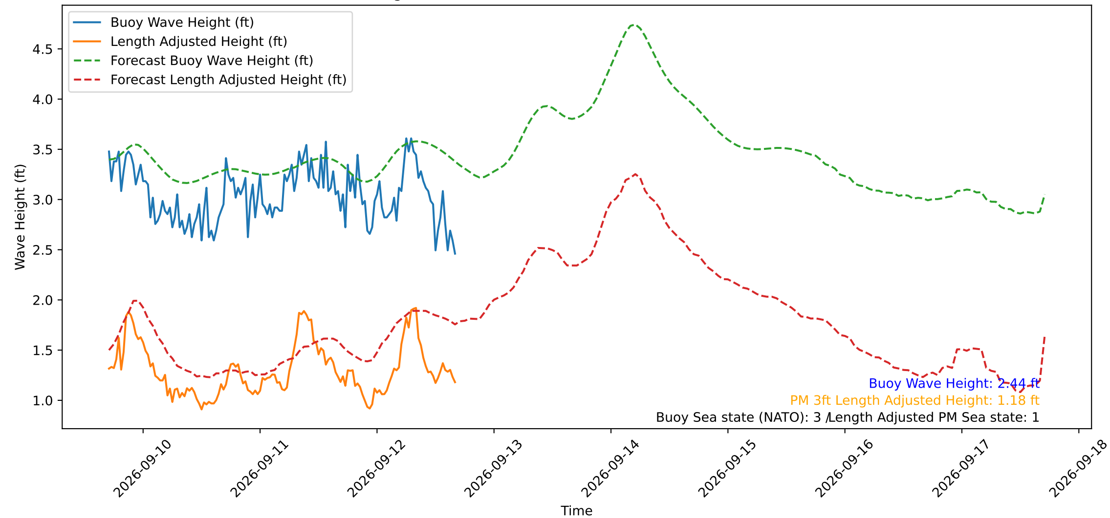
Wave Heights over Time for Green Beach at 2026-09-12 16:41:13
