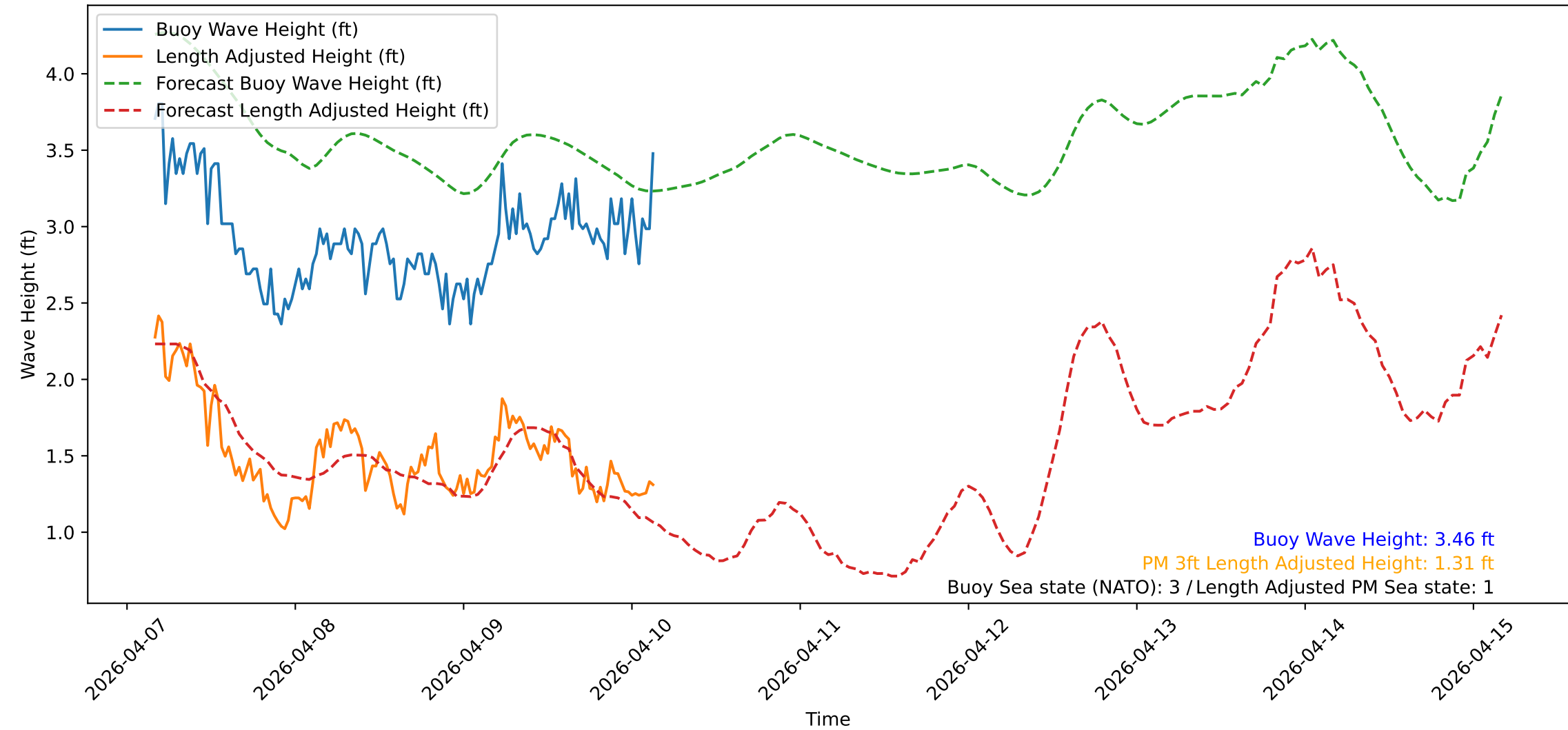
Wave Heights over Time for Green Beach at 2026-04-10 03:51:13
