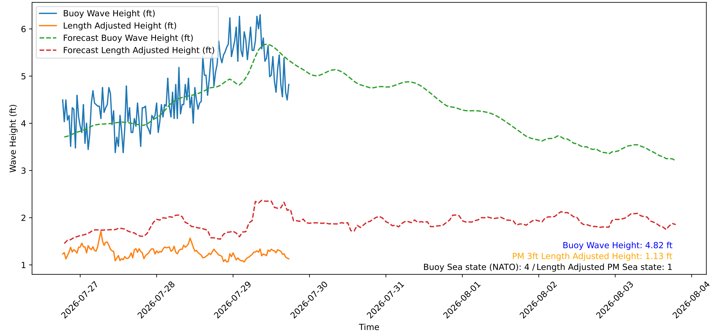
Wave Heights over Time for Green Beach at 2026-07-29 18:31:08
