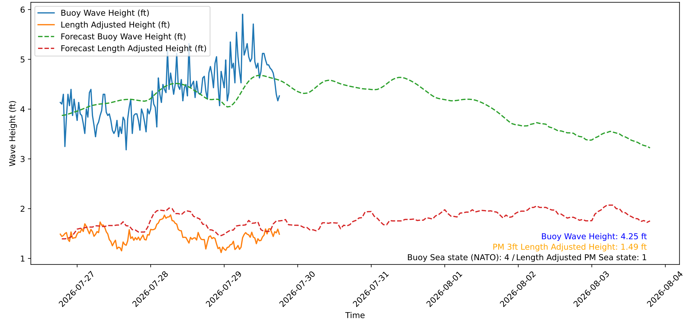
Wave Heights over Time for Oceanside Harbor at 2026-07-29 18:30:26
