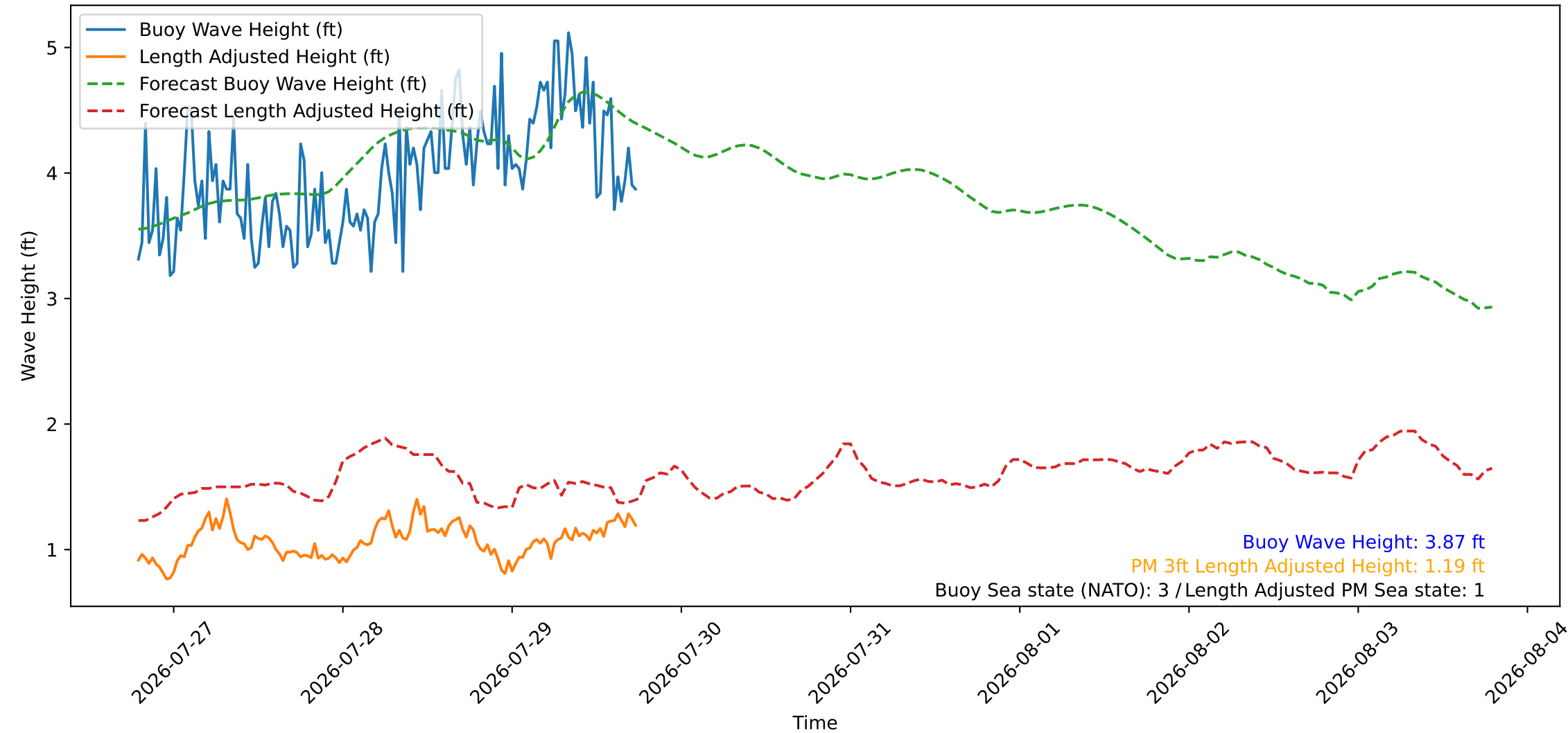
Wave Heights over Time for Red Beach at 2026-07-29 18:30:46
