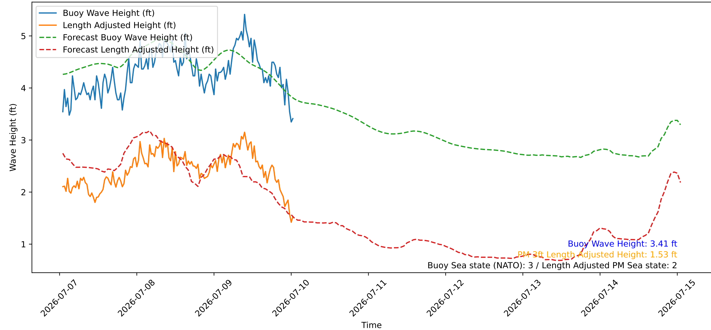
Wave Heights over Time for Oceanside Harbor at 2026-07-10 01:00:26
