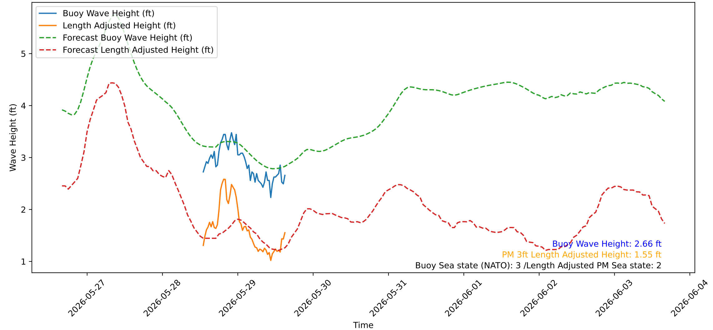
Wave Heights over Time for Oceanside Harbor at 2026-05-29 16:00:21
