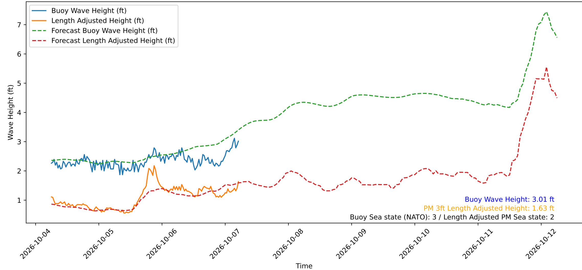
Wave Heights over Time for Oceanside Harbor at 2026-10-07 06:00:30
