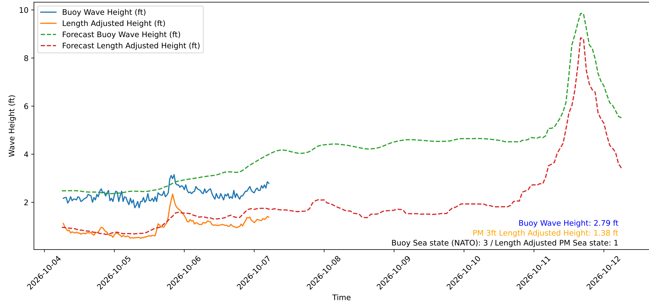
Wave Heights over Time for Green Beach at 2026-10-07 06:01:11
