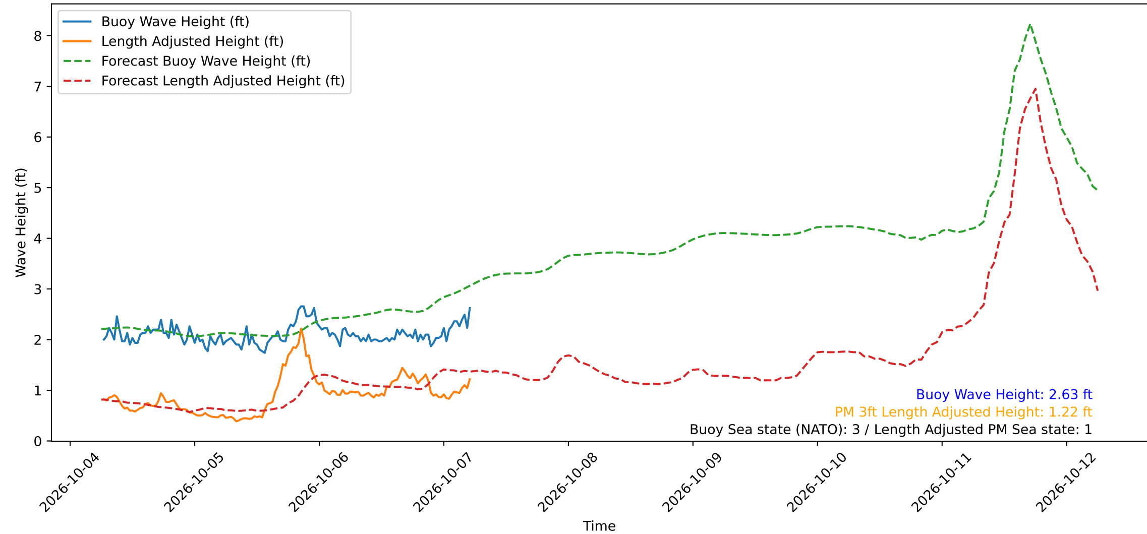
Wave Heights over Time for Red Beach at 2026-10-07 06:00:49
