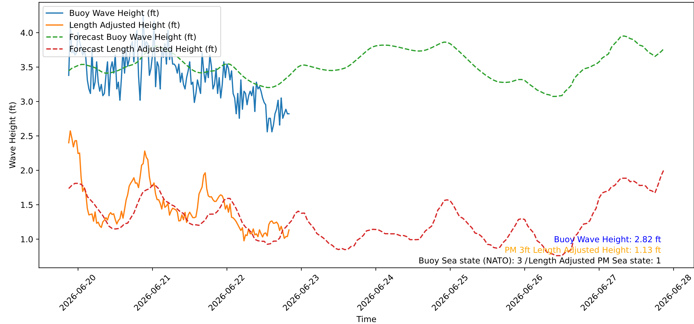
Wave Heights over Time for Oceanside Harbor at 2026-06-22 21:00:27
