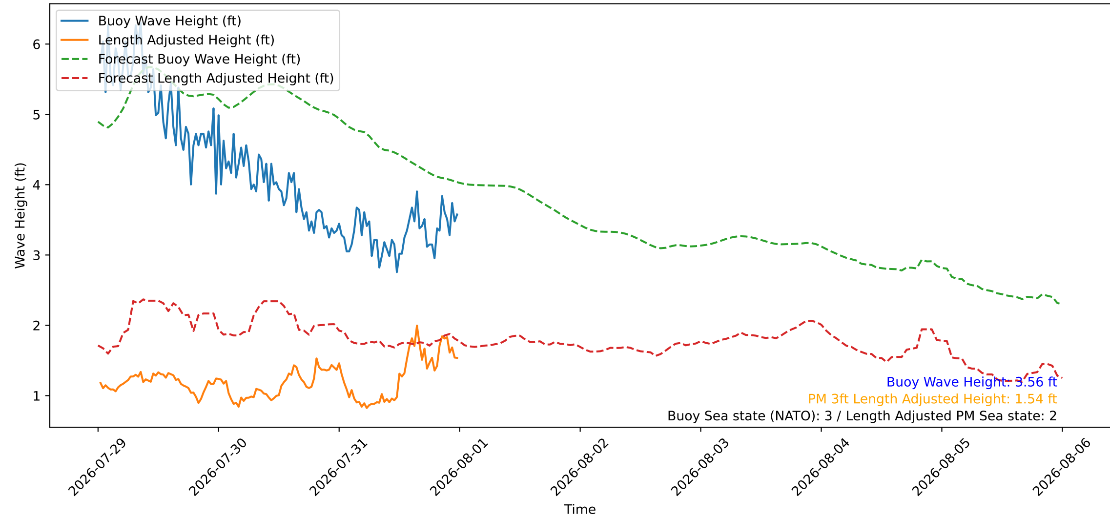
Wave Heights over Time for Green Beach at 2026-08-01 00:21:09
