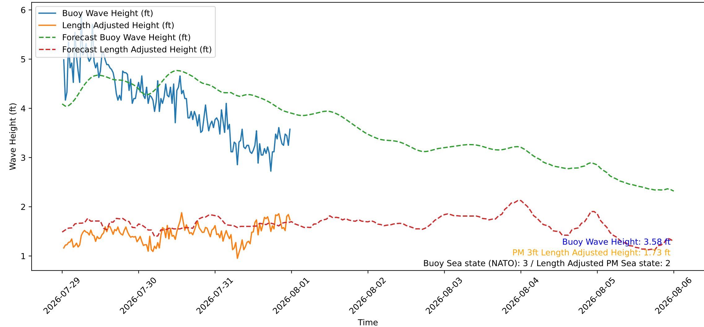
Wave Heights over Time for Oceanside Harbor at 2026-08-01 00:20:26
