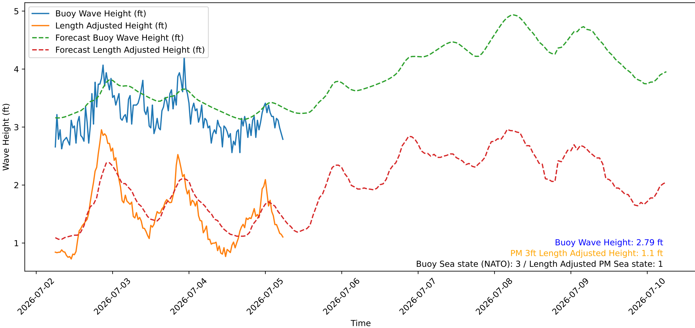
Wave Heights over Time for Green Beach at 2026-07-05 06:11:07
