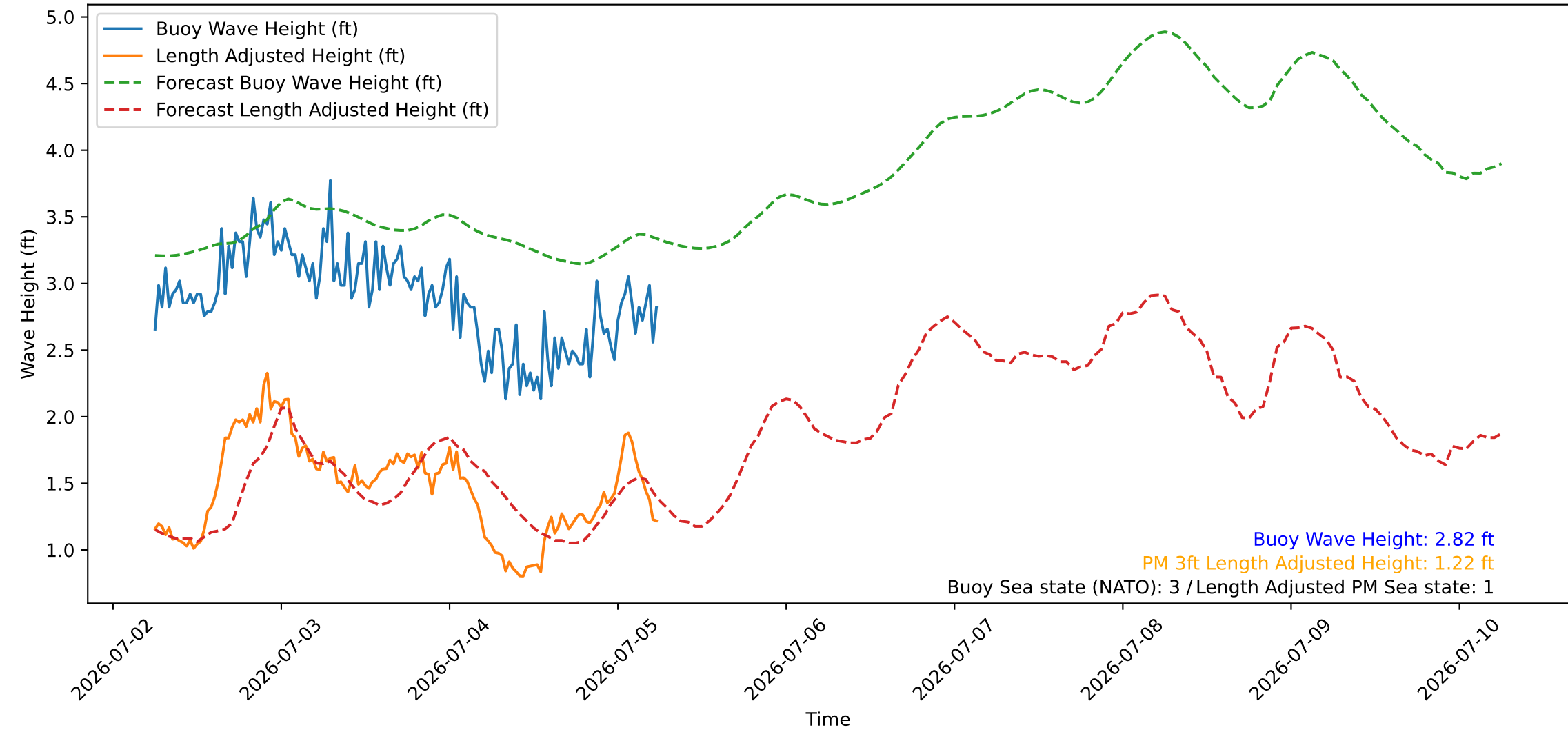
Wave Heights over Time for Oceanside Harbor at 2026-07-05 06:10:26
