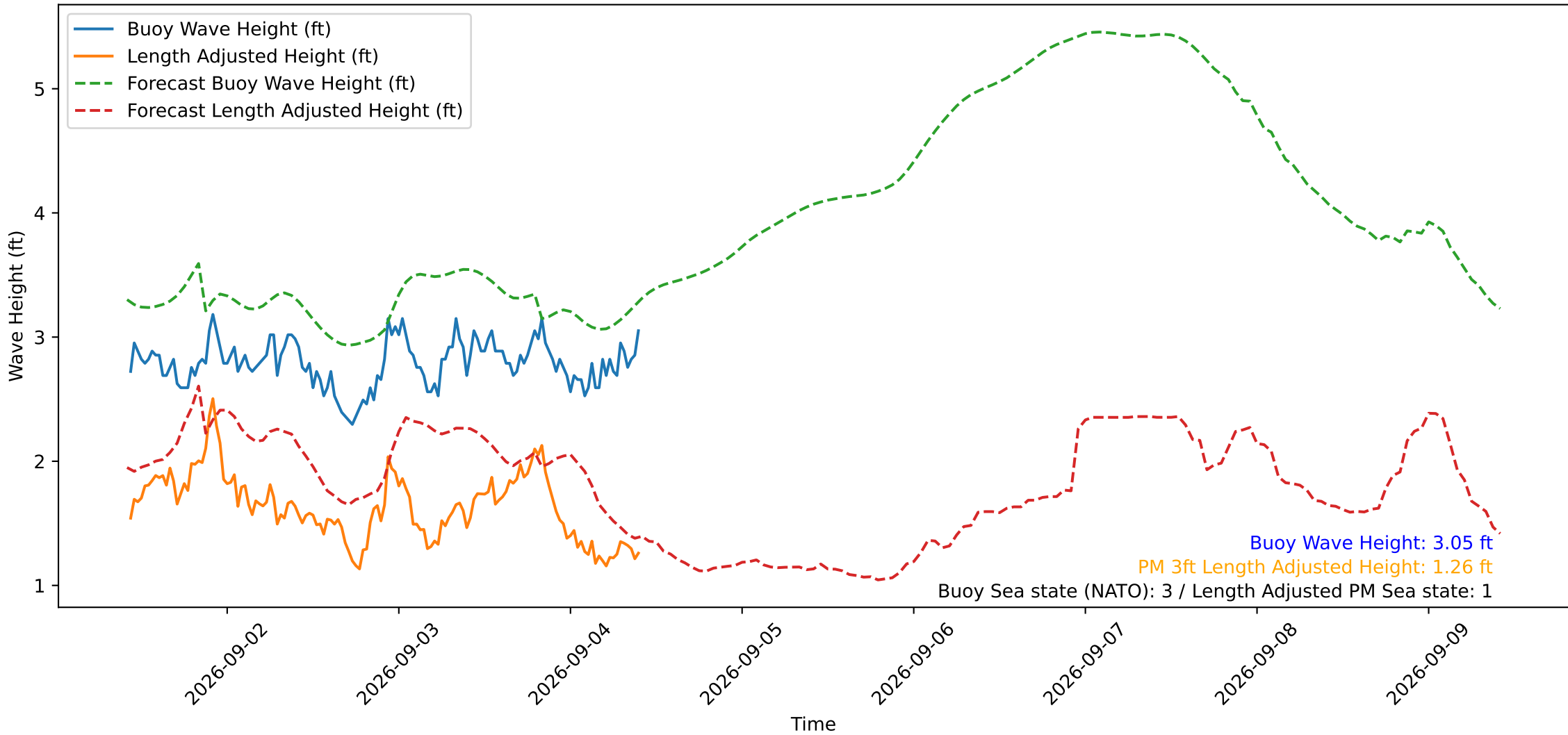
Wave Heights over Time for Red Beach at 2026-09-04 10:20:51
