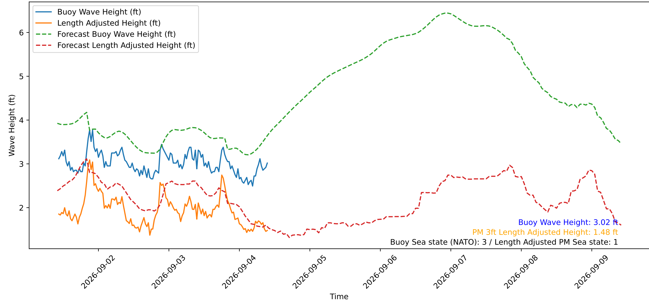
Wave Heights over Time for Green Beach at 2026-09-04 10:21:15
