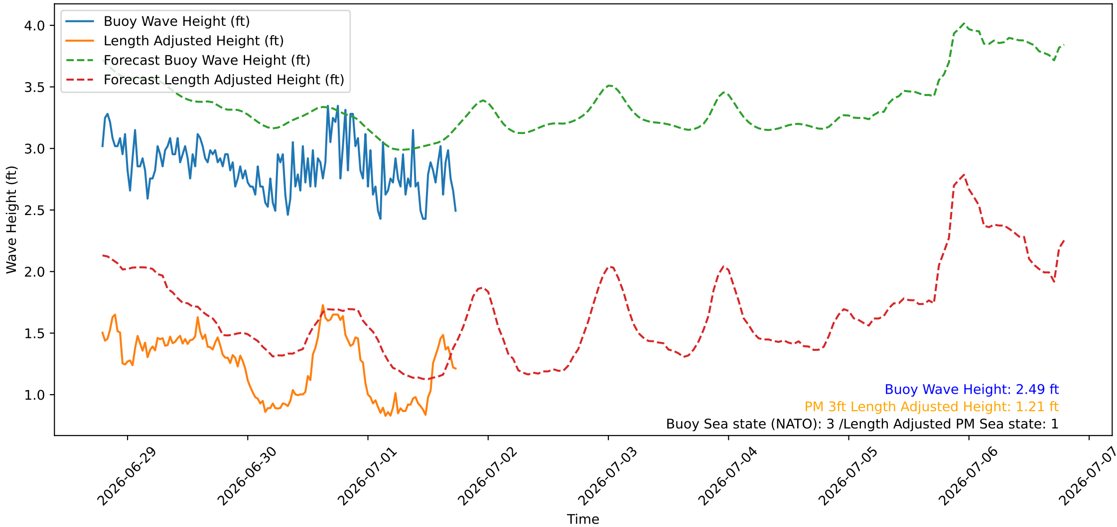
Wave Heights over Time for Red Beach at 2026-07-01 18:30:45
