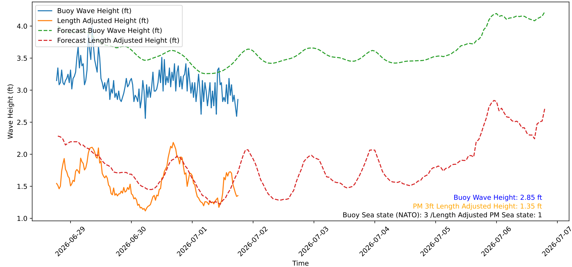
Wave Heights over Time for Oceanside Harbor at 2026-07-01 18:30:26
