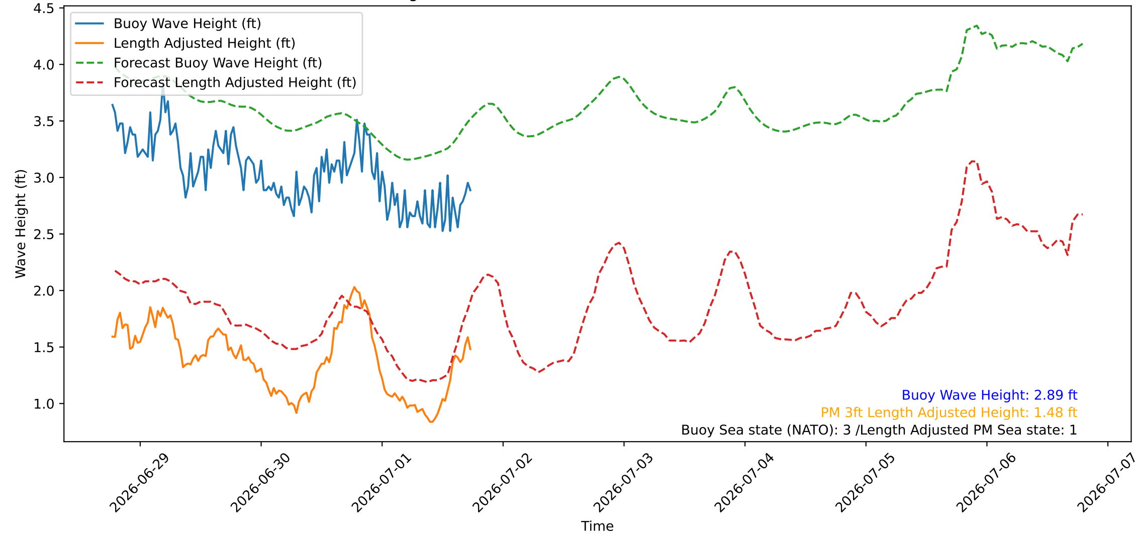
Wave Heights over Time for Green Beach at 2026-07-01 18:31:08
