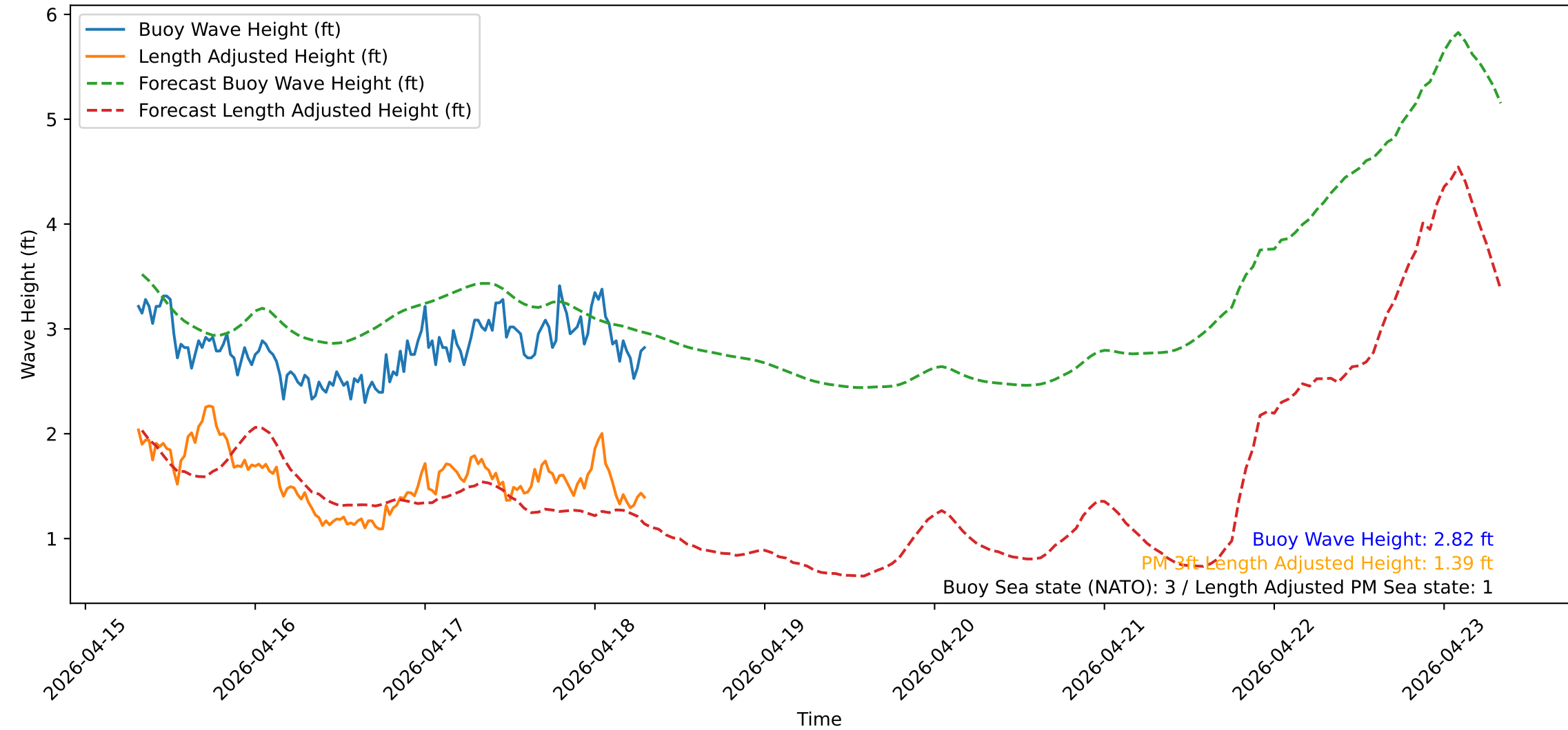
Wave Heights over Time for Oceanside Harbor at 2026-04-18 07:30:31
