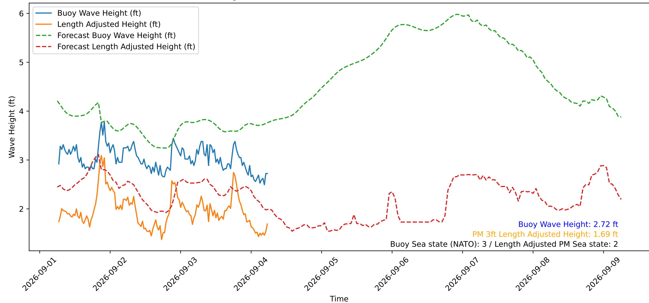
Wave Heights over Time for Green Beach at 2026-09-04 06:11:13
