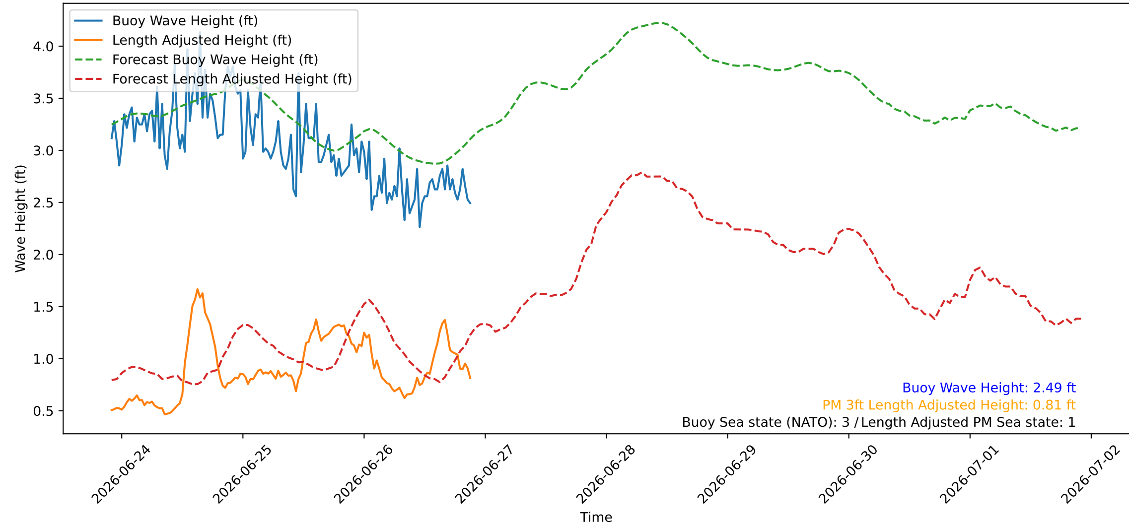
Wave Heights over Time for Red Beach at 2026-06-26 21:50:47
