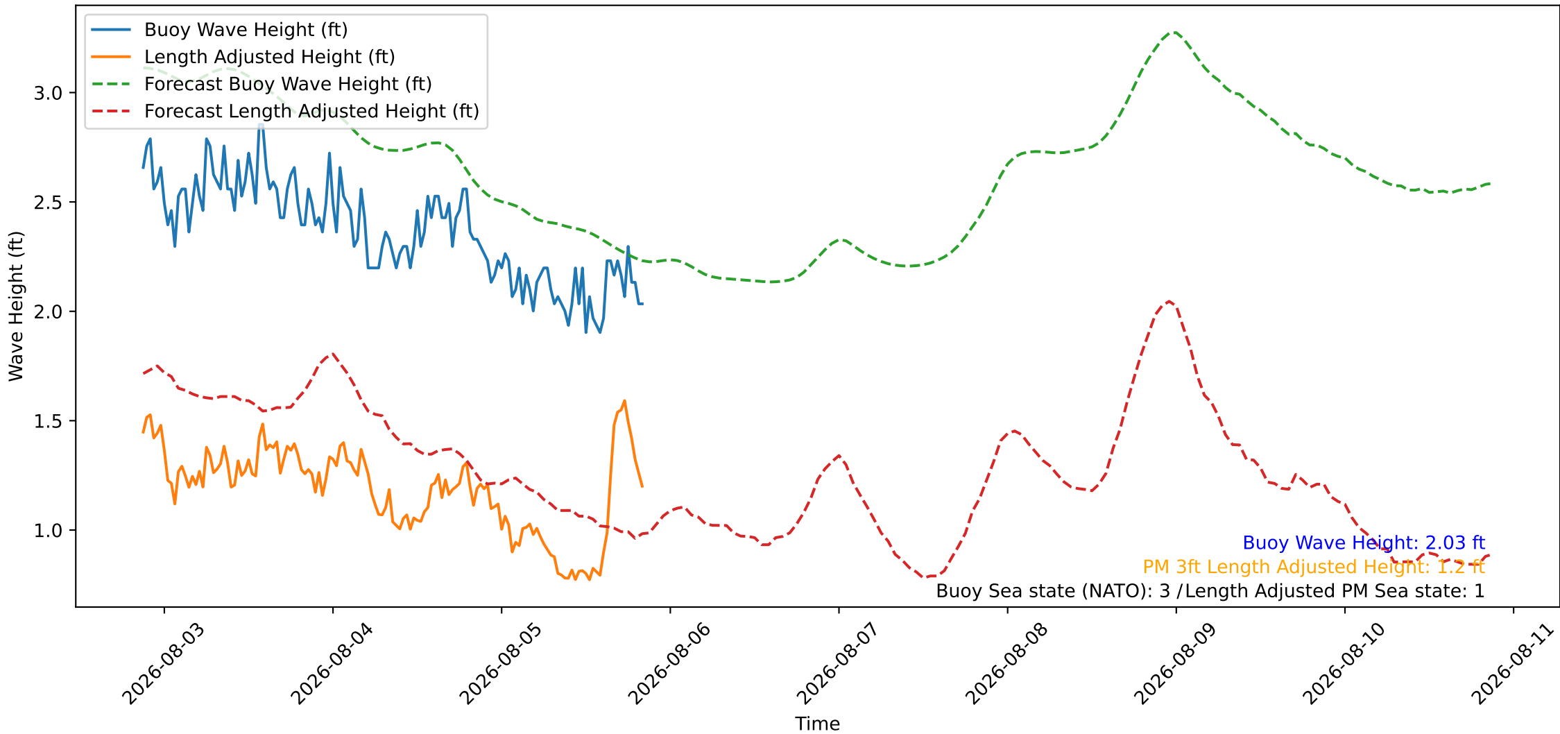
Wave Heights over Time for Oceanside Harbor at 2026-08-05 21:00:26
