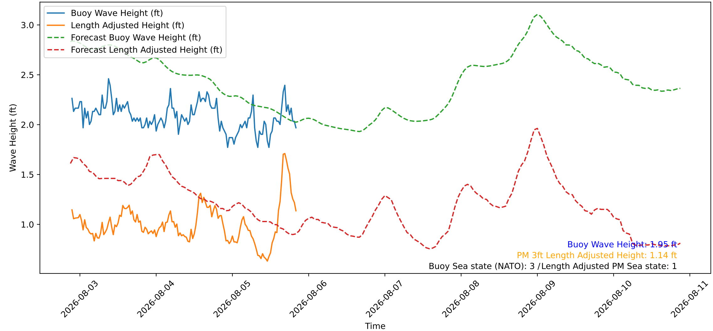
Wave Heights over Time for Red Beach at 2026-08-05 21:00:46
