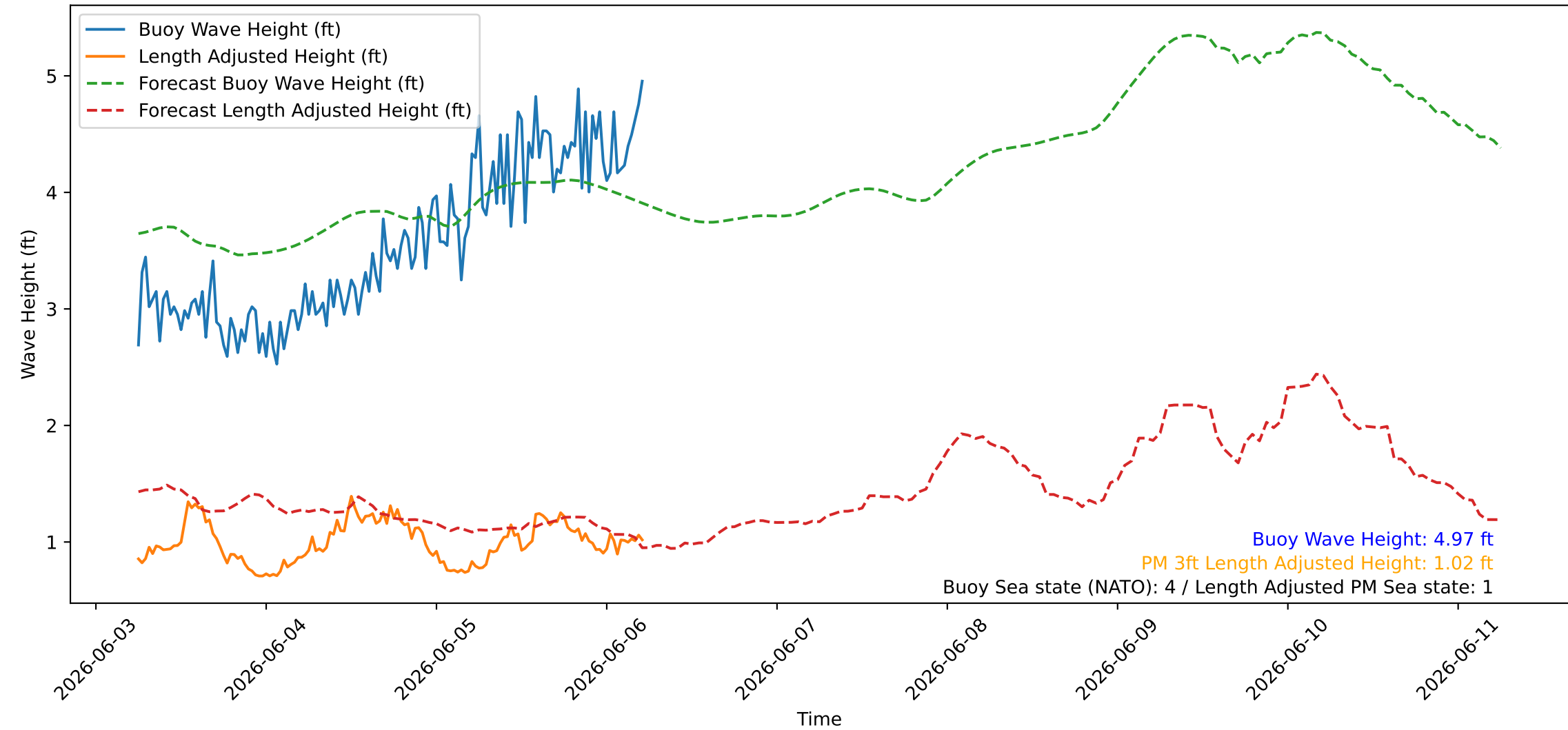
Wave Heights over Time for Red Beach at 2026-06-06 05:50:46
