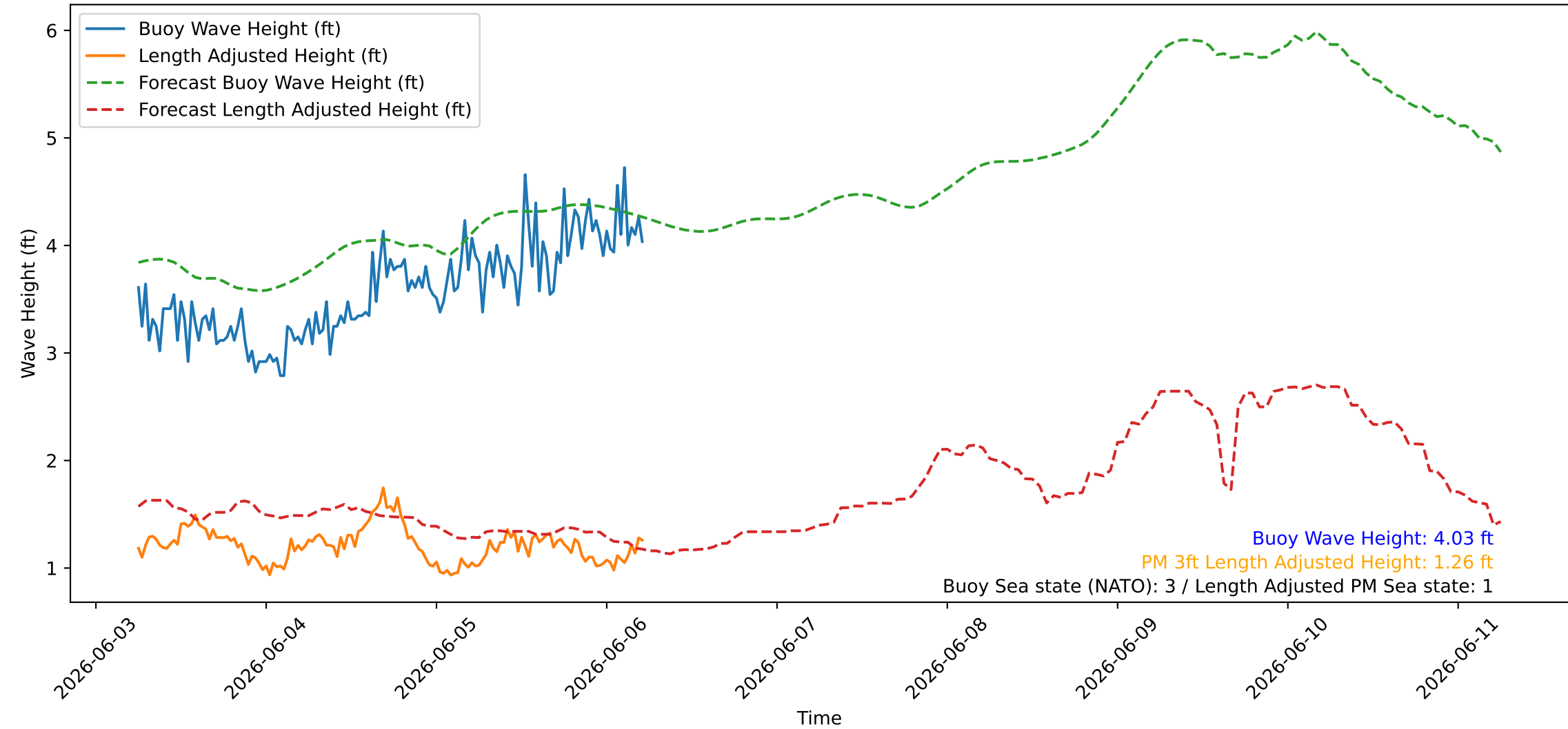
Wave Heights over Time for Green Beach at 2026-06-06 05:51:08
