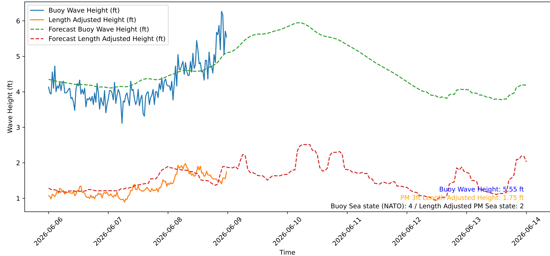
Wave Heights over Time for Green Beach at 2026-06-09 00:11:08
