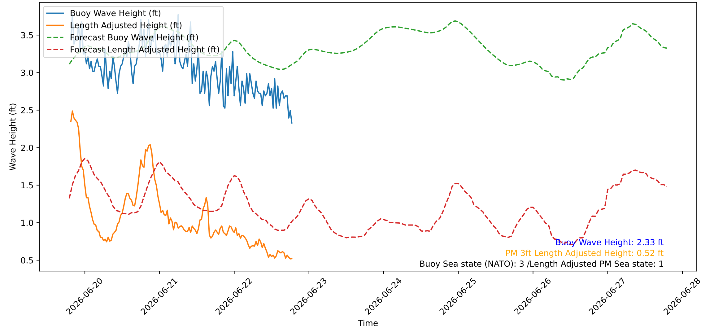
Wave Heights over Time for Red Beach at 2026-06-22 19:20:48
