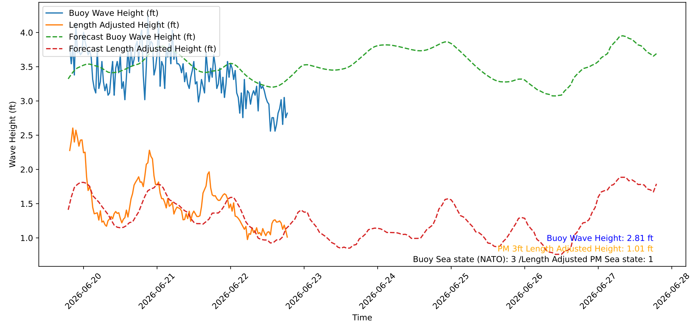
Wave Heights over Time for Oceanside Harbor at 2026-06-22 19:20:26
