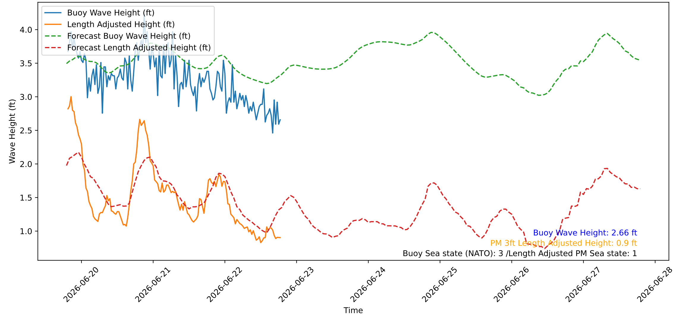
Wave Heights over Time for Green Beach at 2026-06-22 19:21:10
