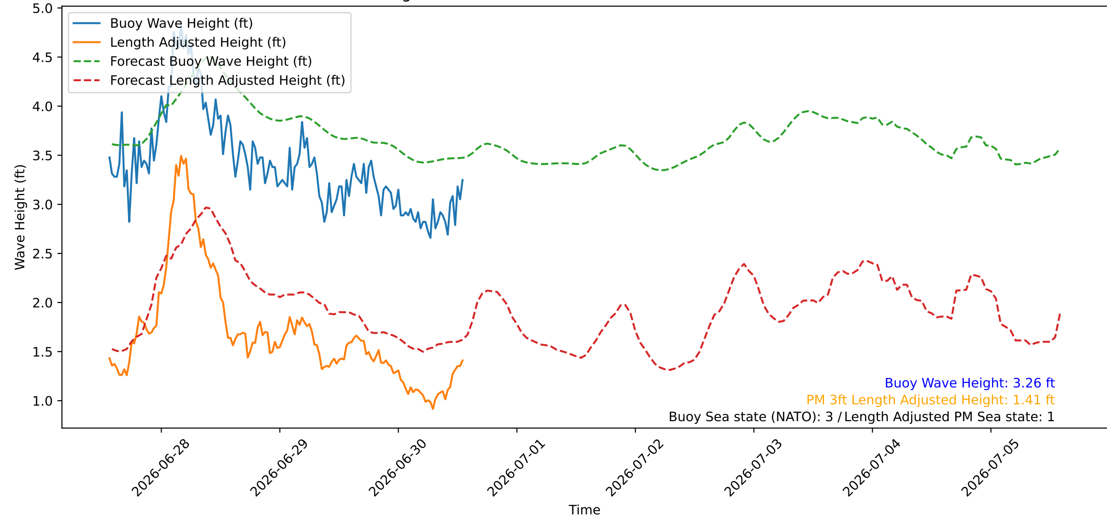
Wave Heights over Time for Green Beach at 2026-06-30 13:41:08
