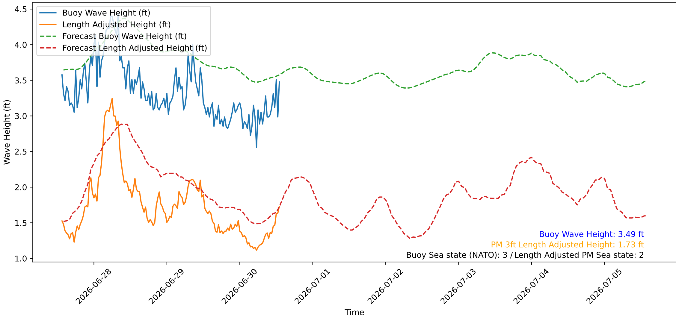
Wave Heights over Time for Oceanside Harbor at 2026-06-30 13:40:26
