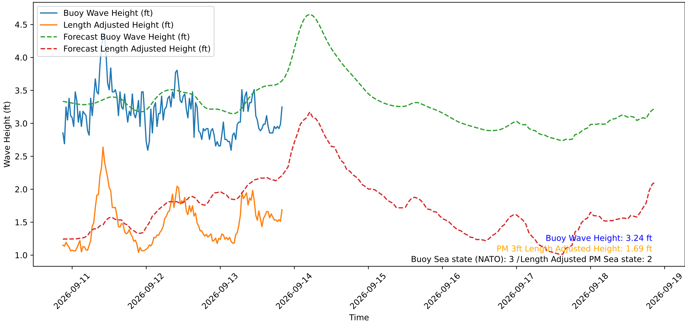
Wave Heights over Time for Oceanside Harbor at 2026-09-13 20:50:29
