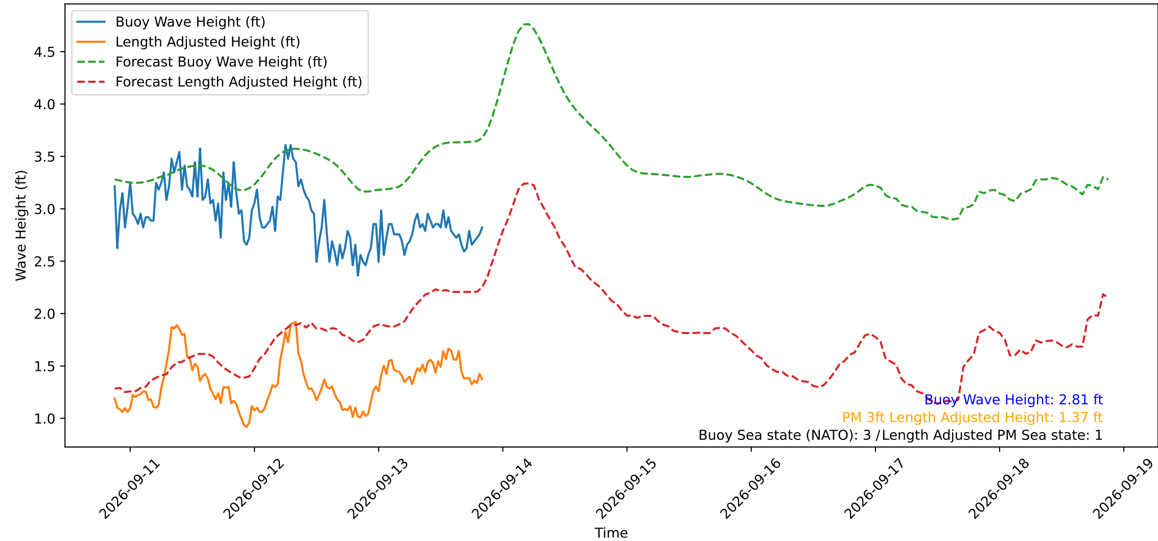
Wave Heights over Time for Green Beach at 2026-09-13 20:51:14
