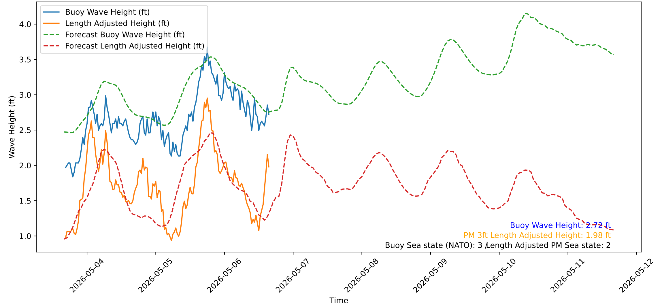
Wave Heights over Time for Green Beach at 2026-05-06 16:21:14
