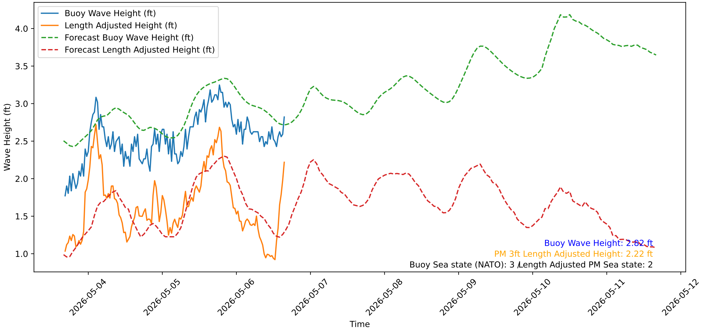
Wave Heights over Time for Oceanside Harbor at 2026-05-06 16:20:31
