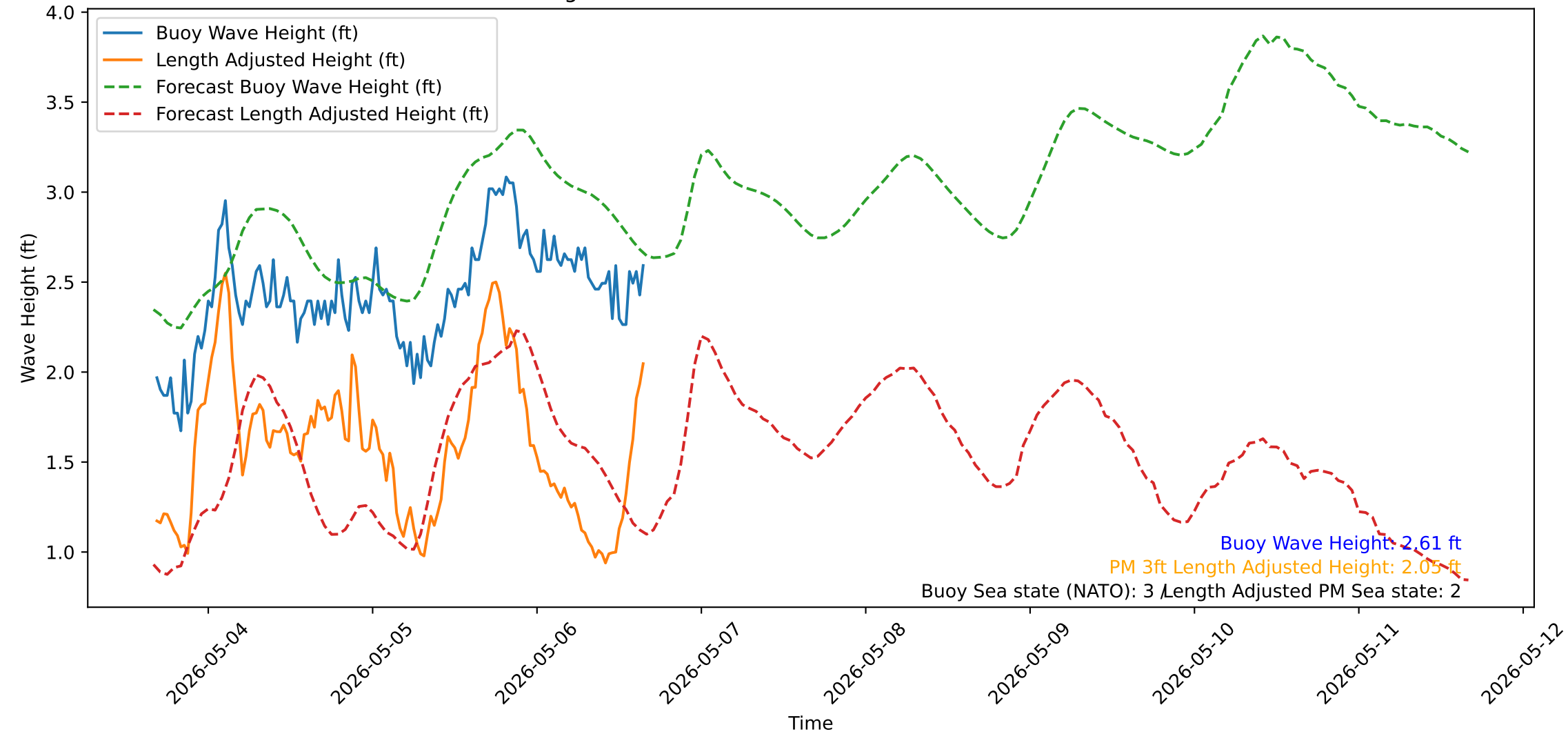
Wave Heights over Time for Red Beach at 2026-05-06 16:20:51
