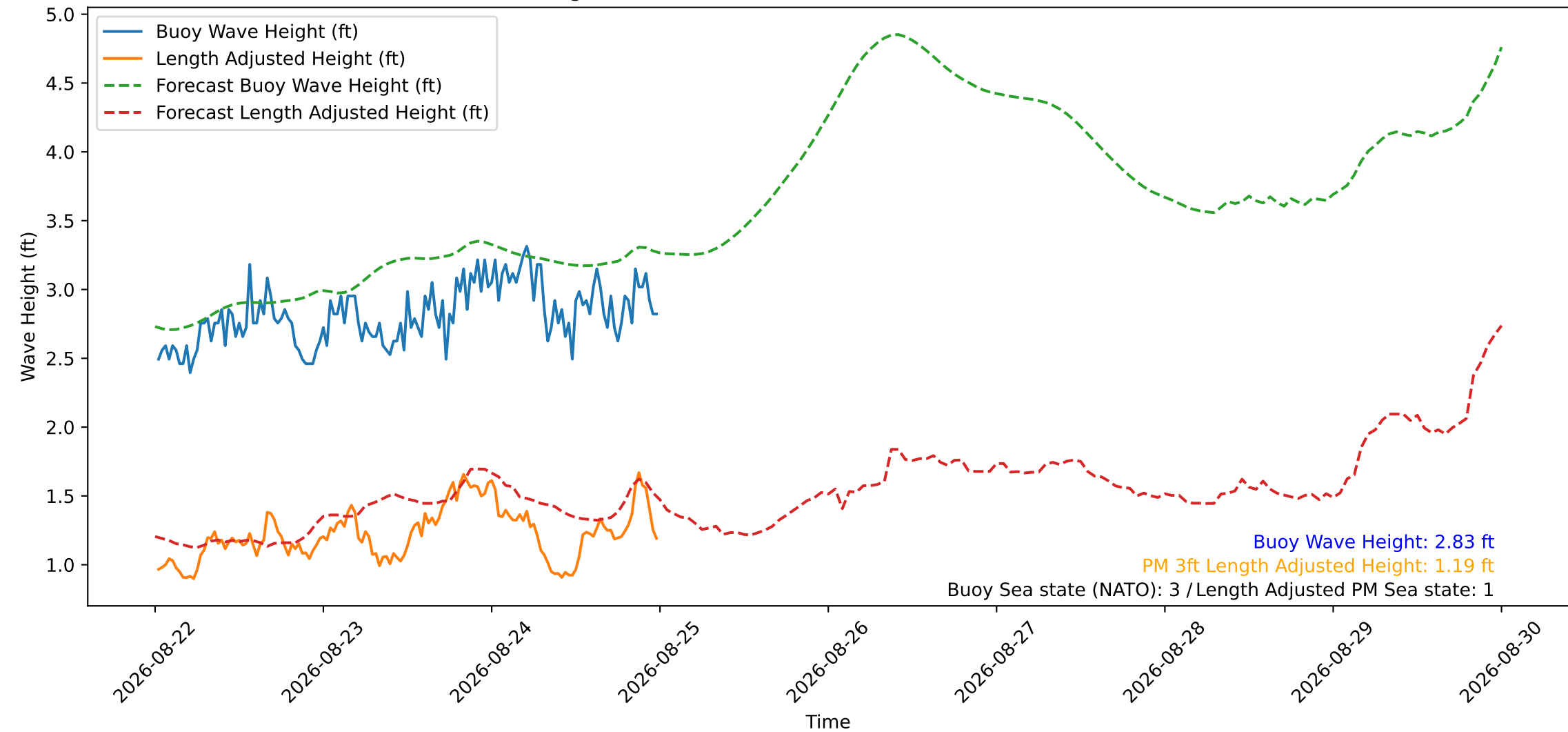
Wave Heights over Time for Green Beach at 2026-08-25 00:11:12
