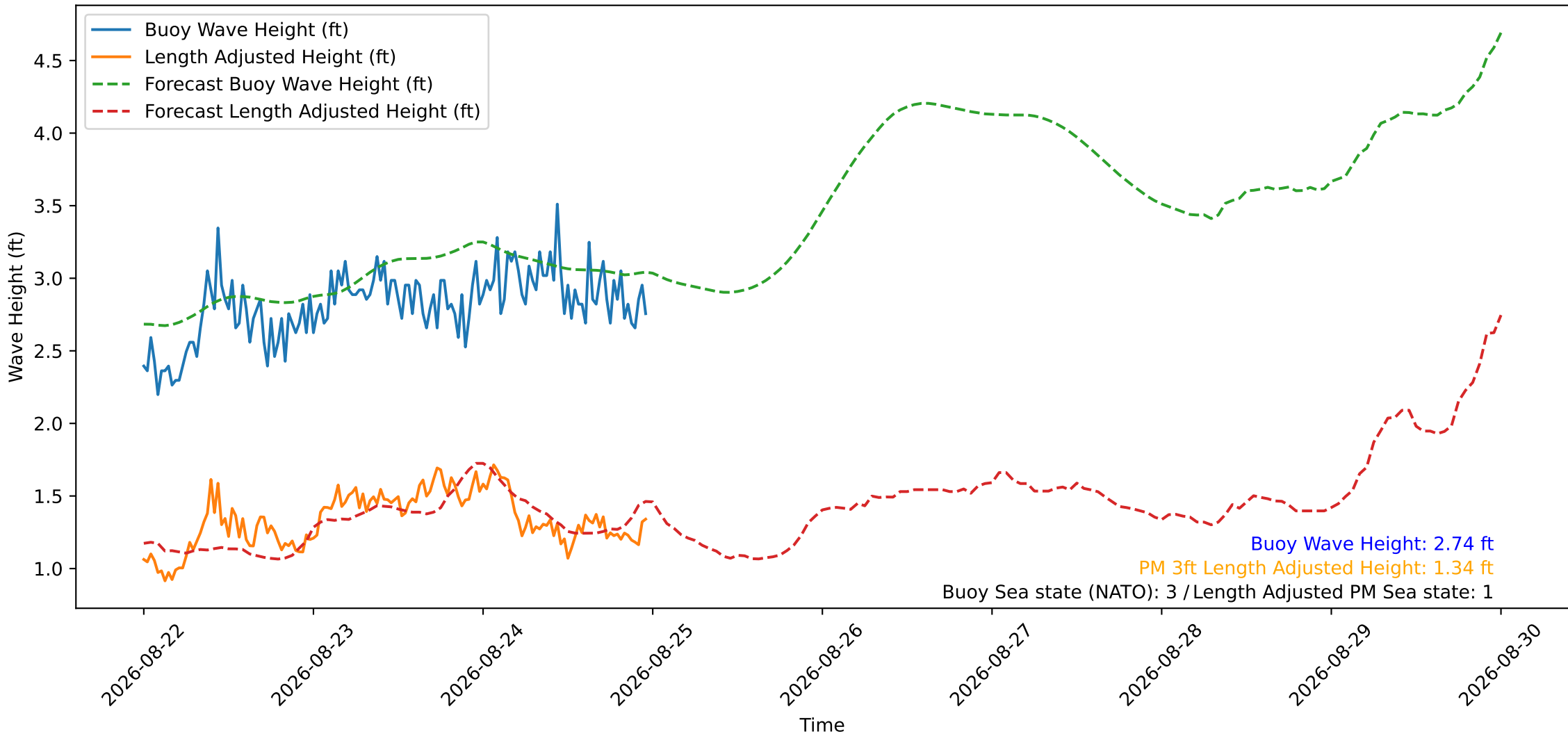
Wave Heights over Time for Oceanside Harbor at 2026-08-25 00:10:29
