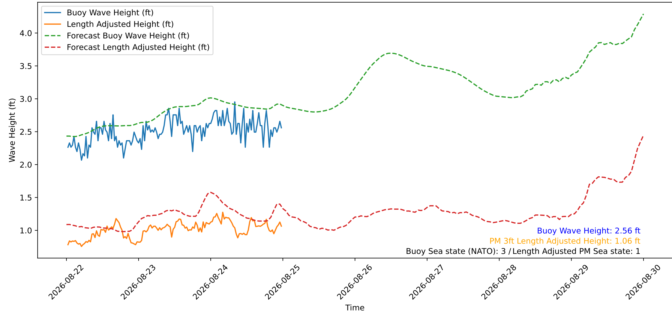
Wave Heights over Time for Red Beach at 2026-08-25 00:10:49
