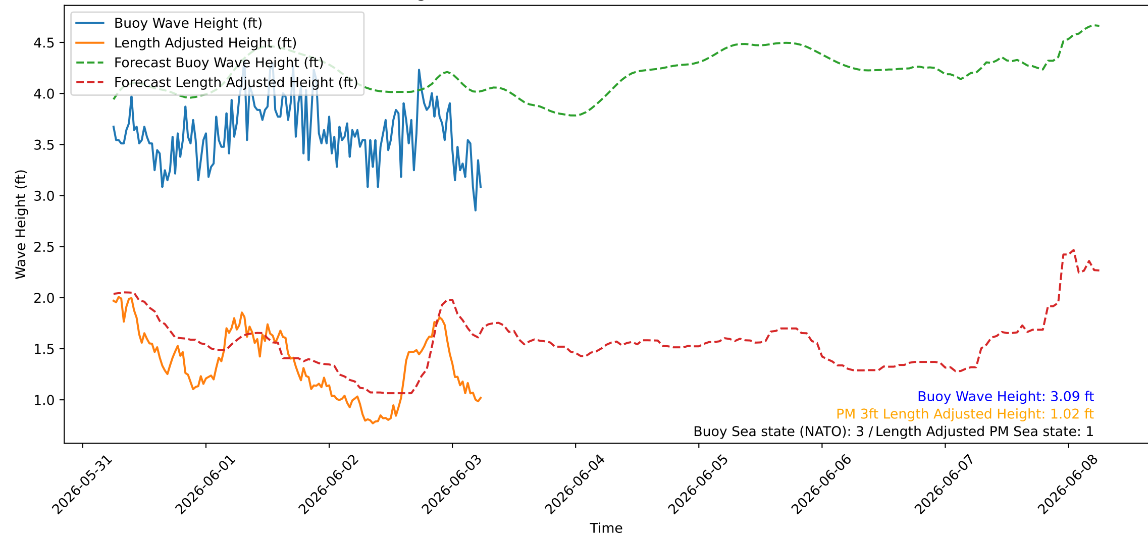
Wave Heights over Time for Green Beach at 2026-06-03 06:11:07
