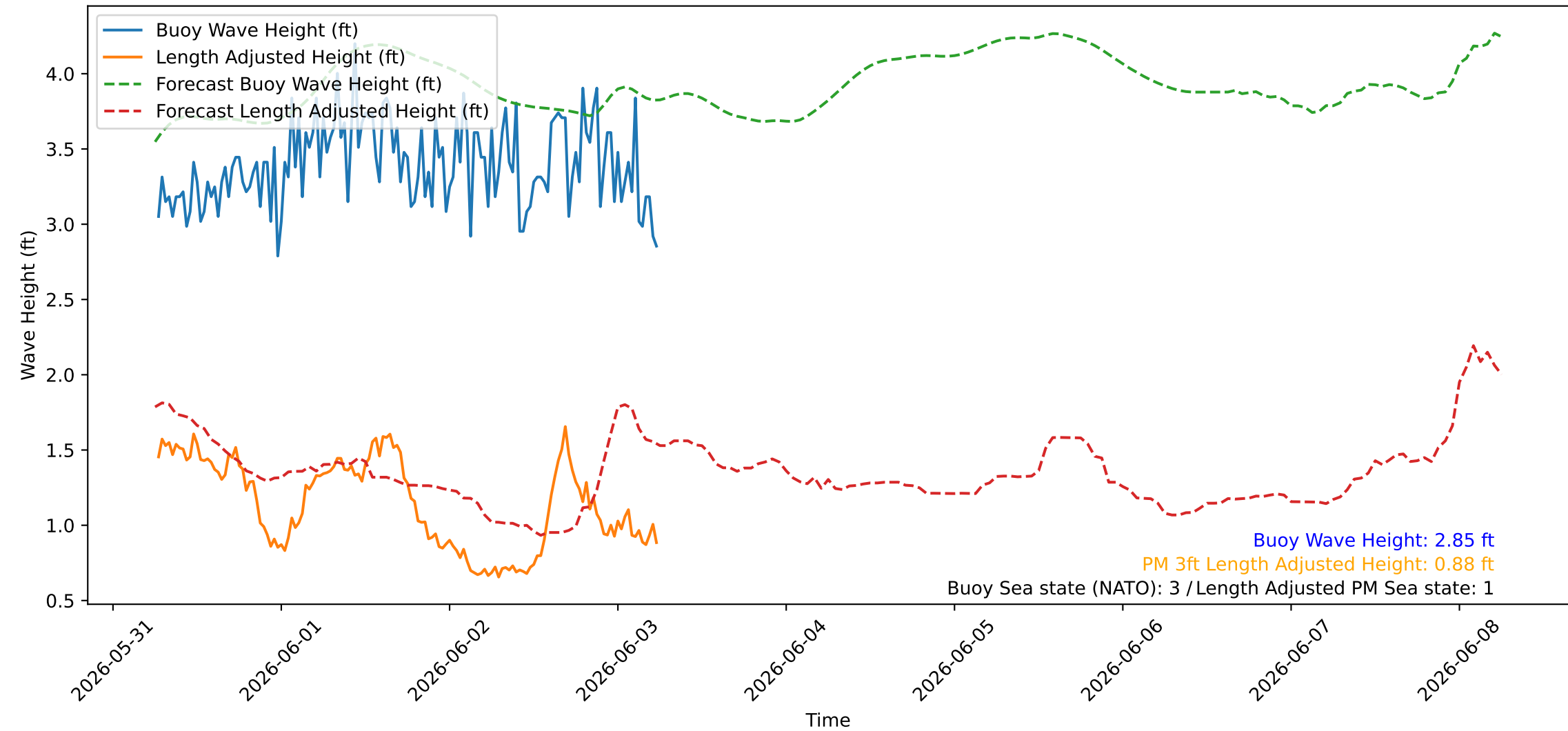
Wave Heights over Time for Red Beach at 2026-06-03 06:10:45
