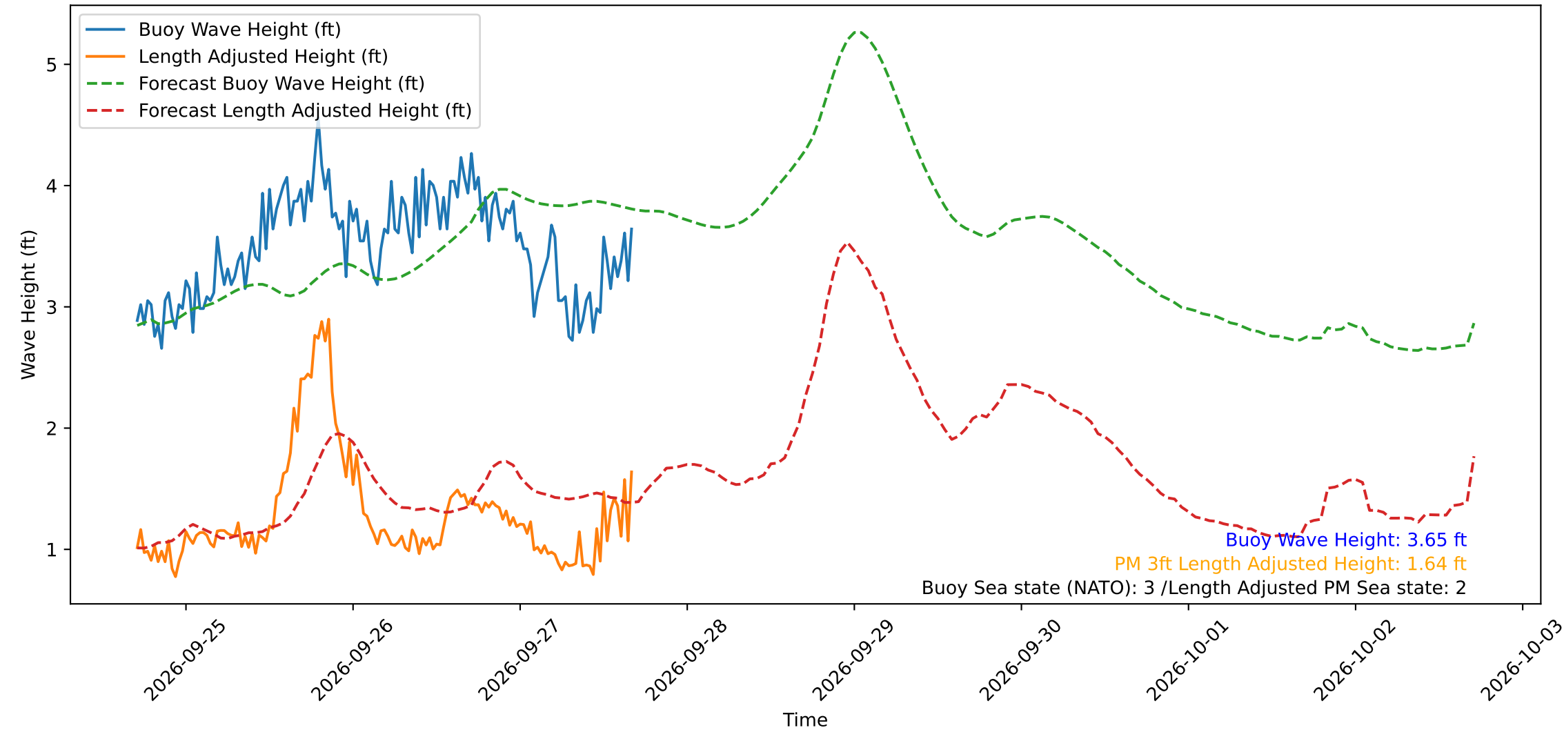
Wave Heights over Time for Green Beach at 2026-09-27 16:51:15
