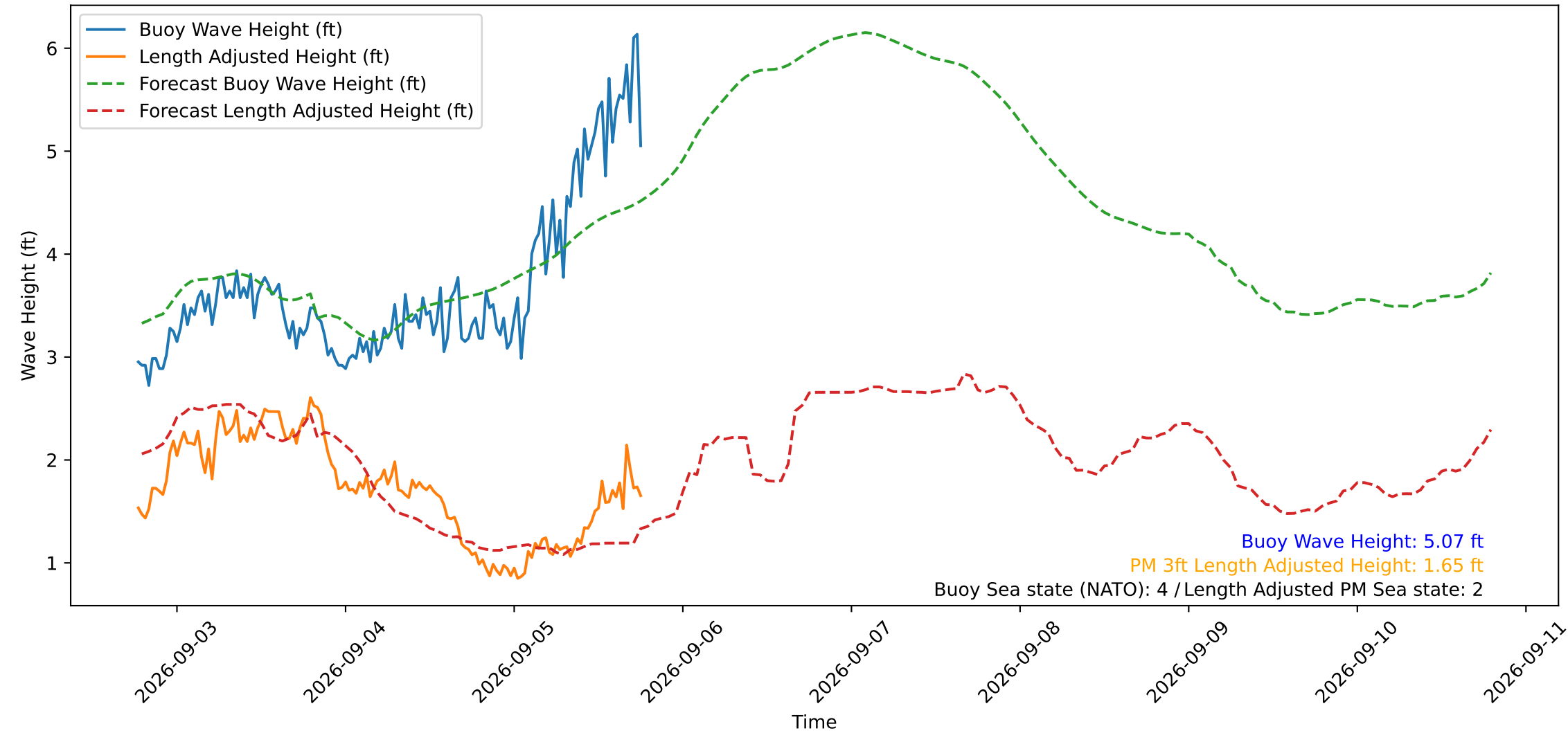
Wave Heights over Time for Oceanside Harbor at 2026-09-05 18:40:29
