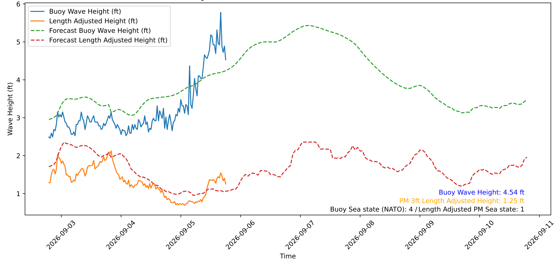
Wave Heights over Time for Red Beach at 2026-09-05 18:40:49
