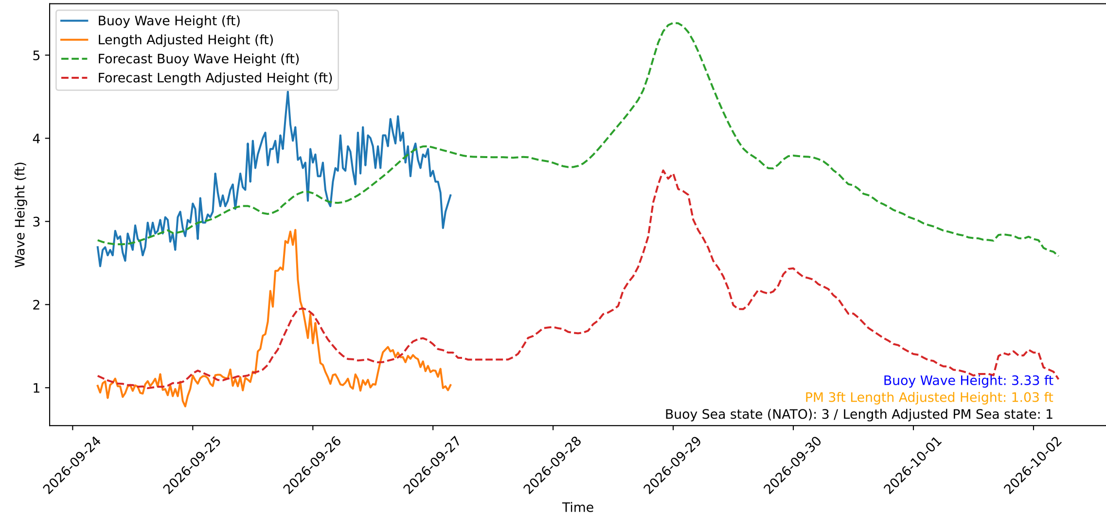
Wave Heights over Time for Green Beach at 2026-09-27 04:31:12
