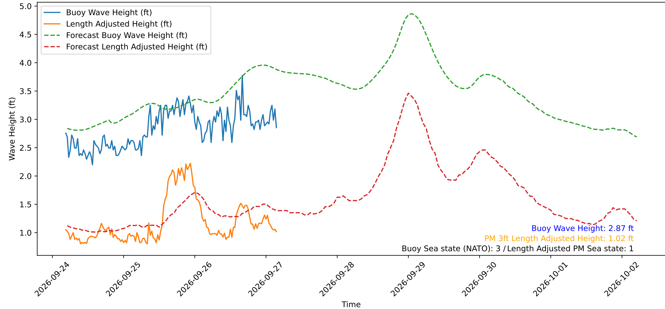
Wave Heights over Time for Oceanside Harbor at 2026-09-27 04:30:30
