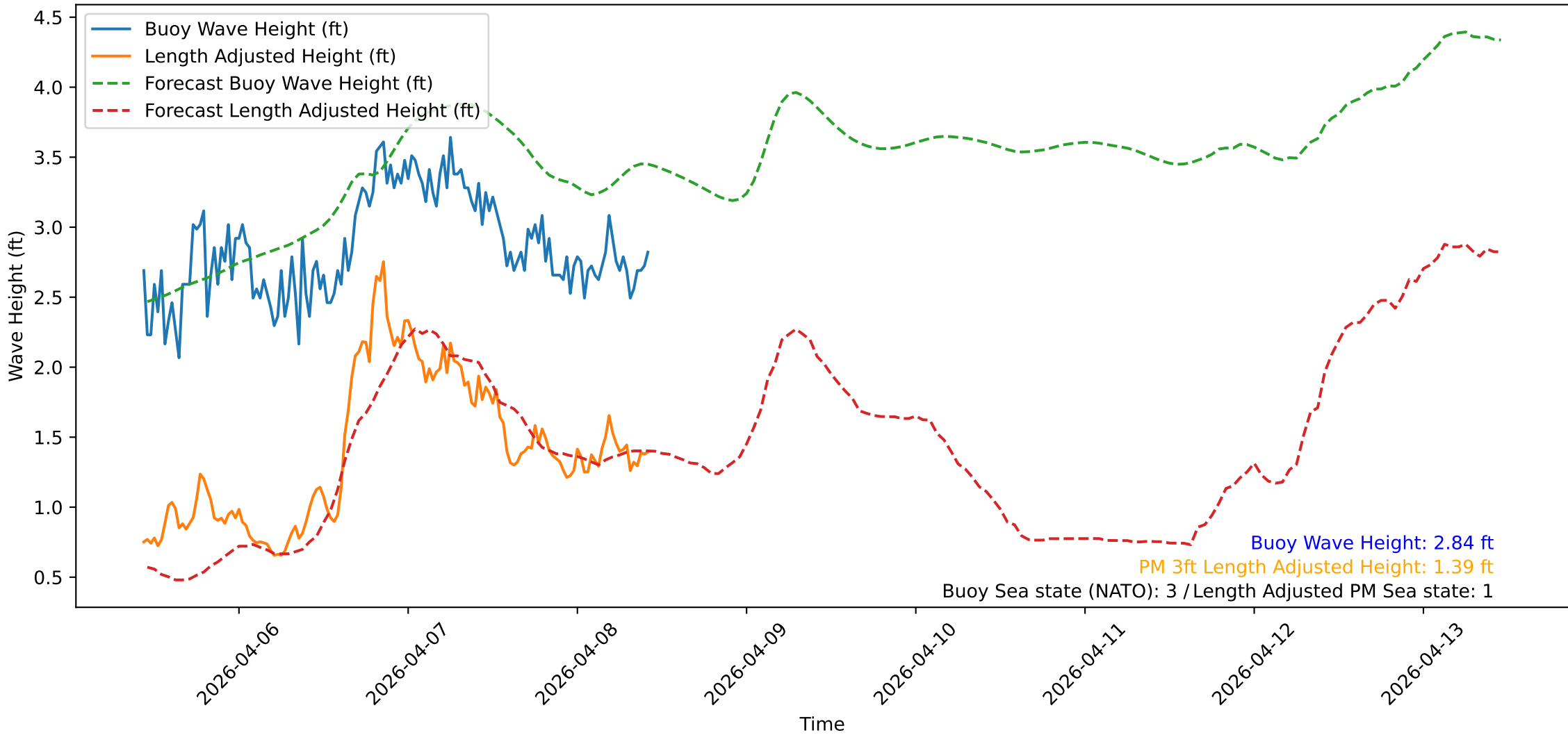
Wave Heights over Time for Oceanside Harbor at 2026-04-08 10:40:32
