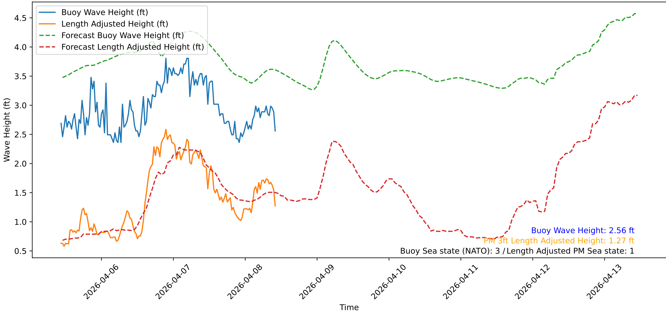
Wave Heights over Time for Green Beach at 2026-04-08 10:41:10
