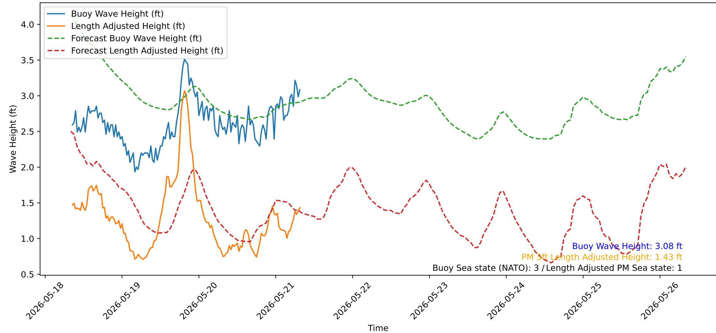
Wave Heights over Time for Red Beach at 2026-05-21 08:20:52
