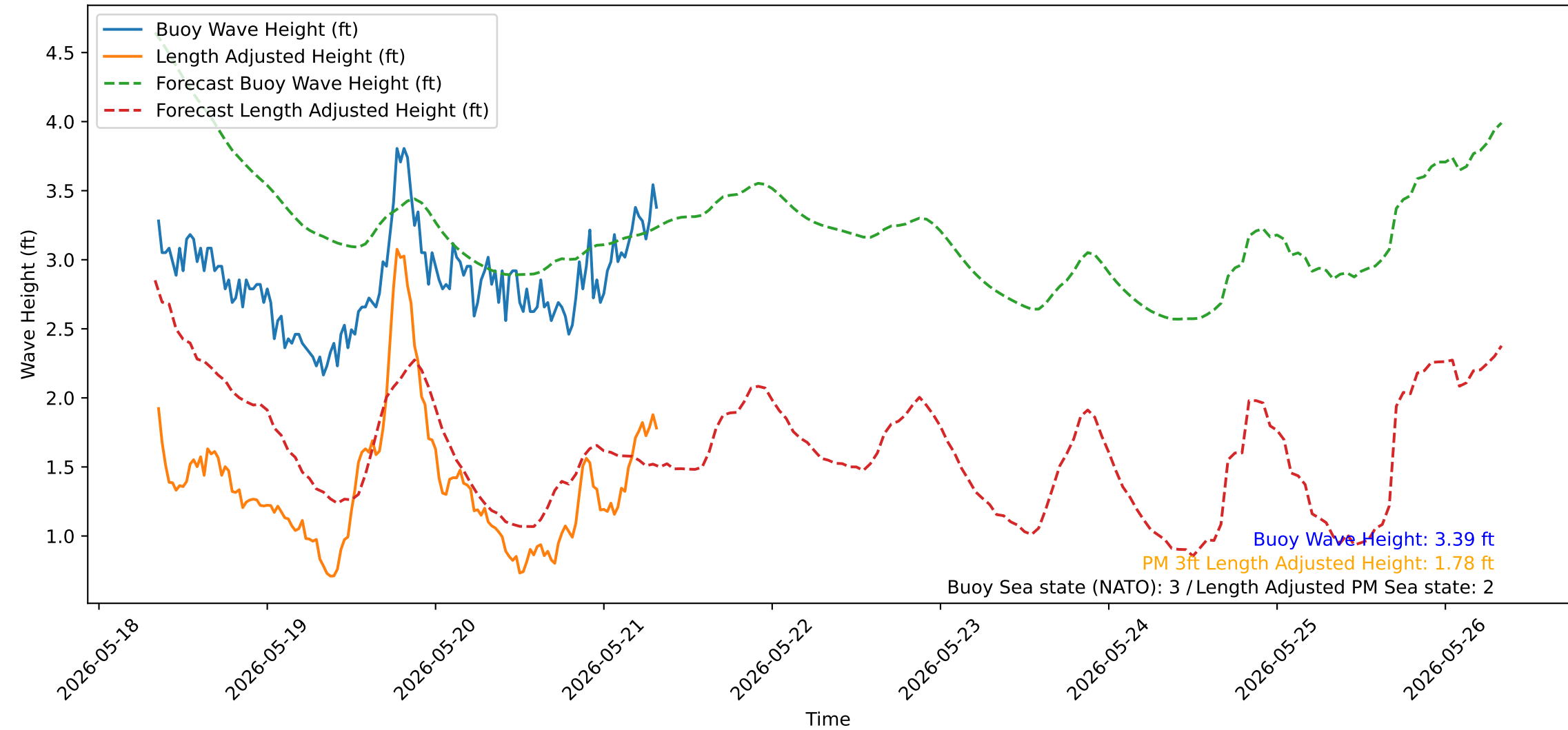
Wave Heights over Time for Green Beach at 2026-05-21 08:21:14
