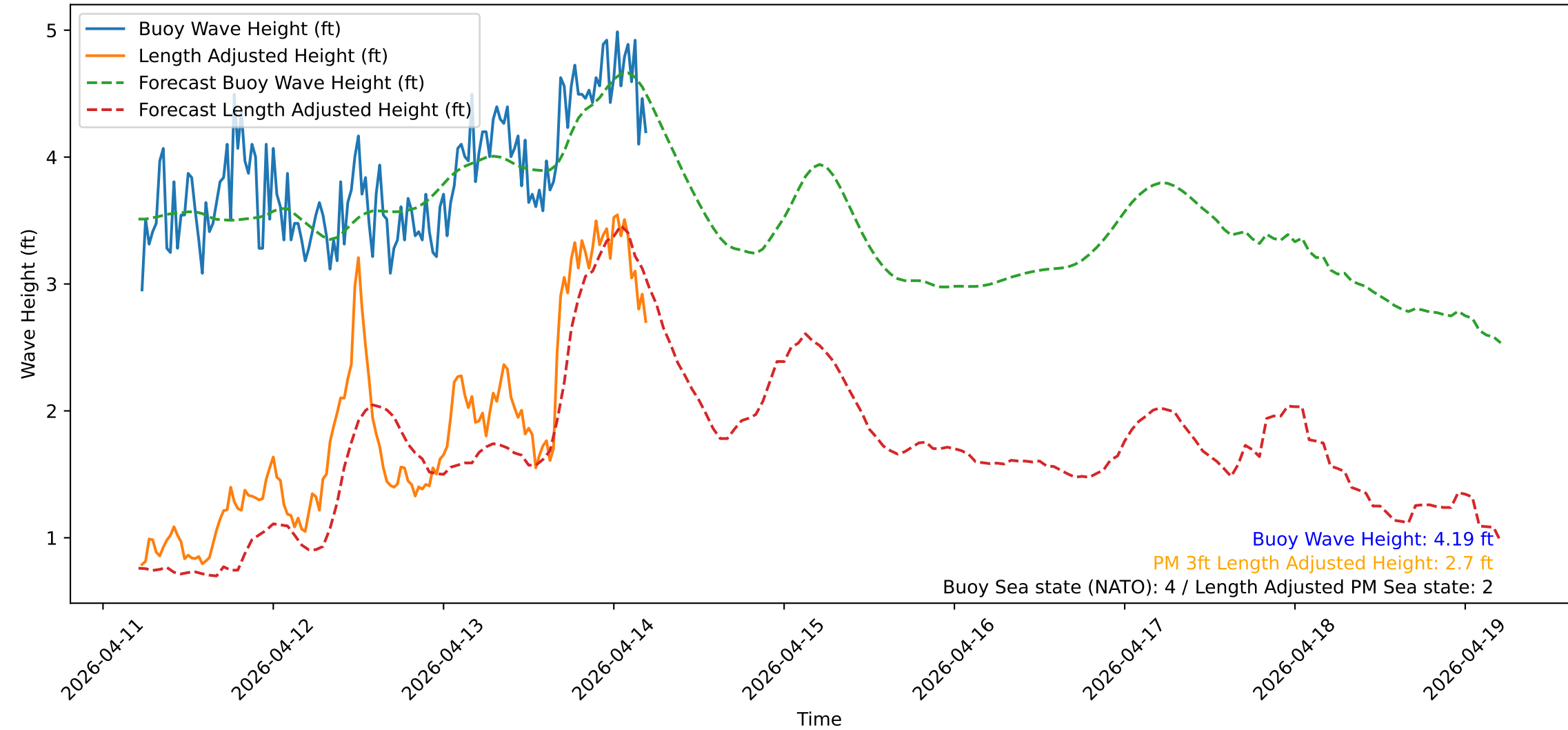
Wave Heights over Time for Green Beach at 2026-04-14 05:21:14
