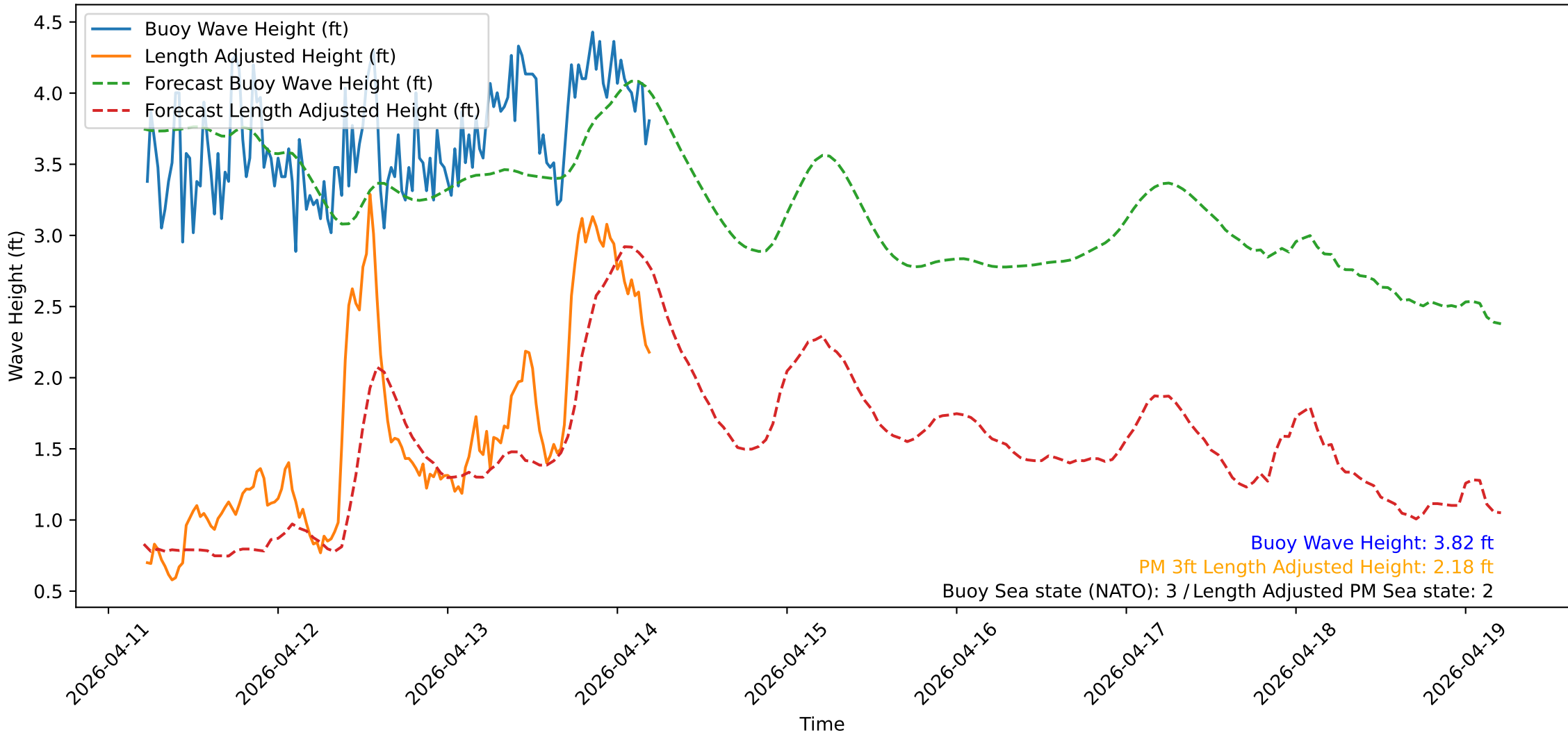
Wave Heights over Time for Red Beach at 2026-04-14 05:20:52
