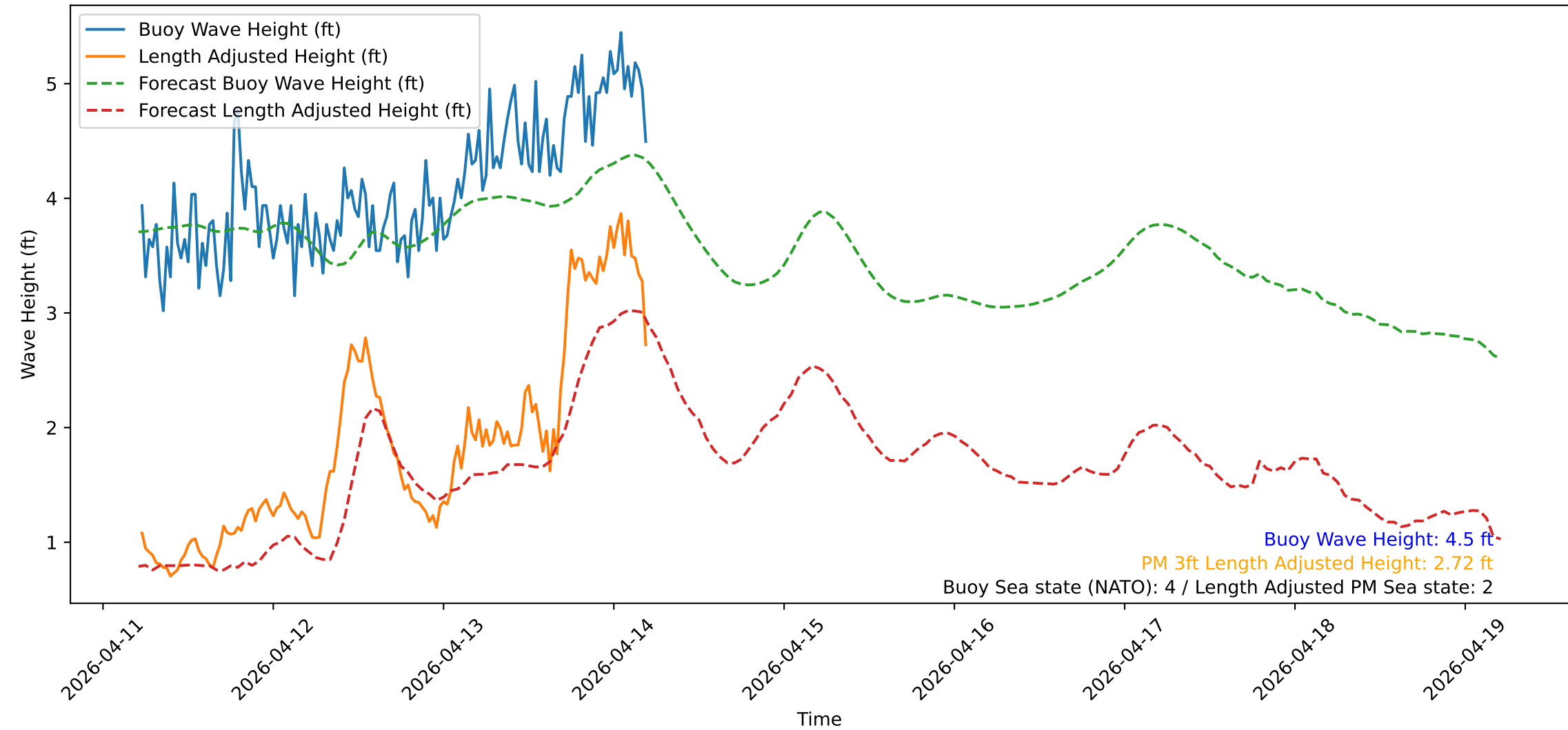
Wave Heights over Time for Oceanside Harbor at 2026-04-14 05:20:31
