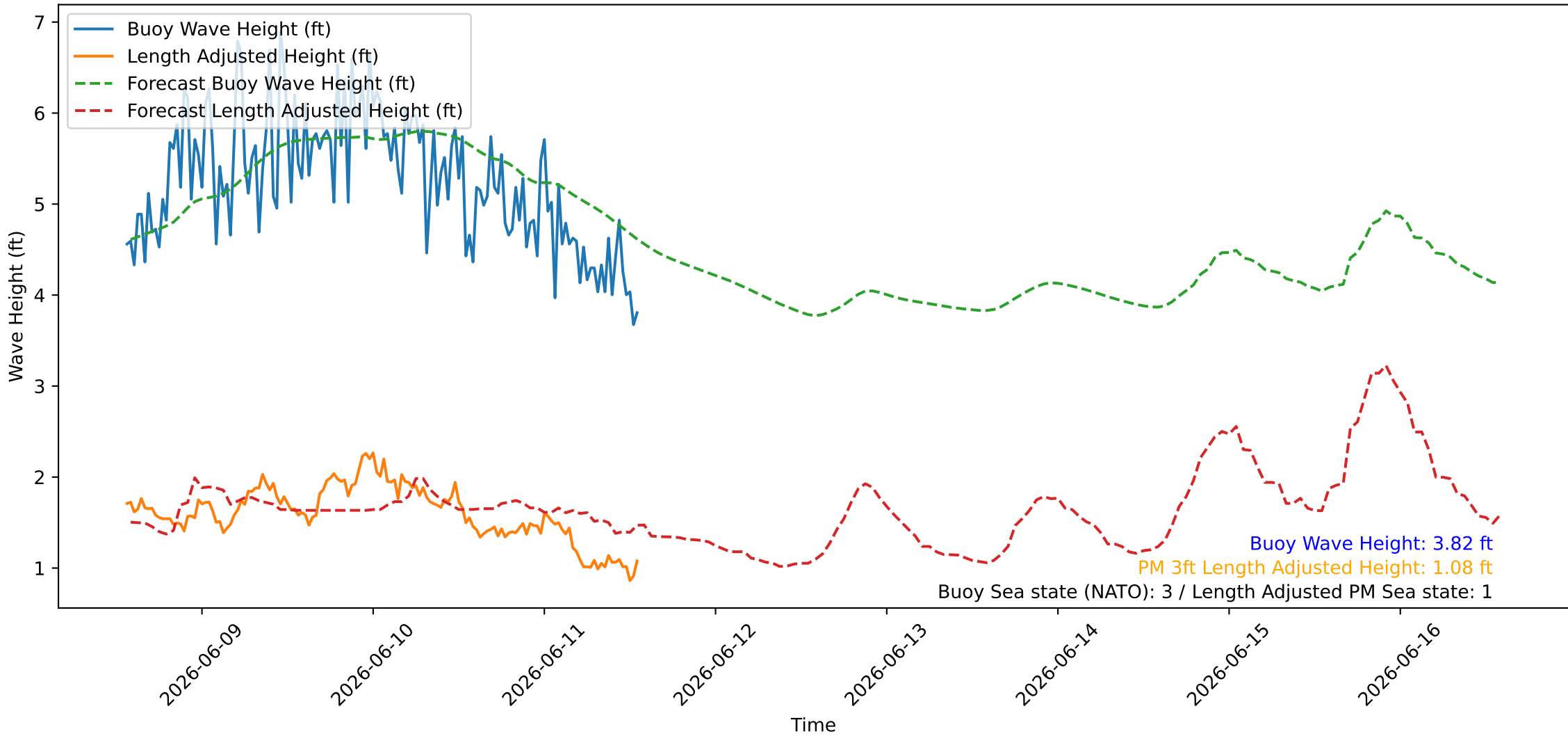
Wave Heights over Time for Green Beach at 2026-06-11 13:41:10
