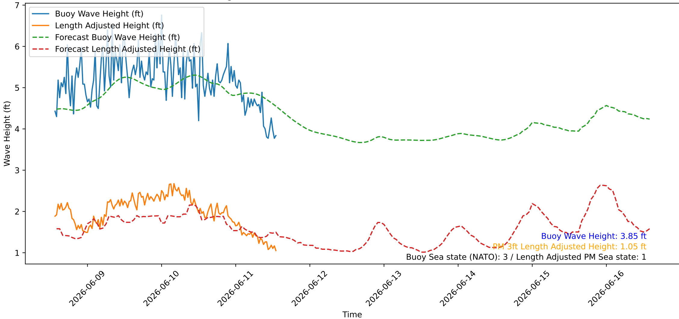
Wave Heights over Time for Oceanside Harbor at 2026-06-11 13:40:26
