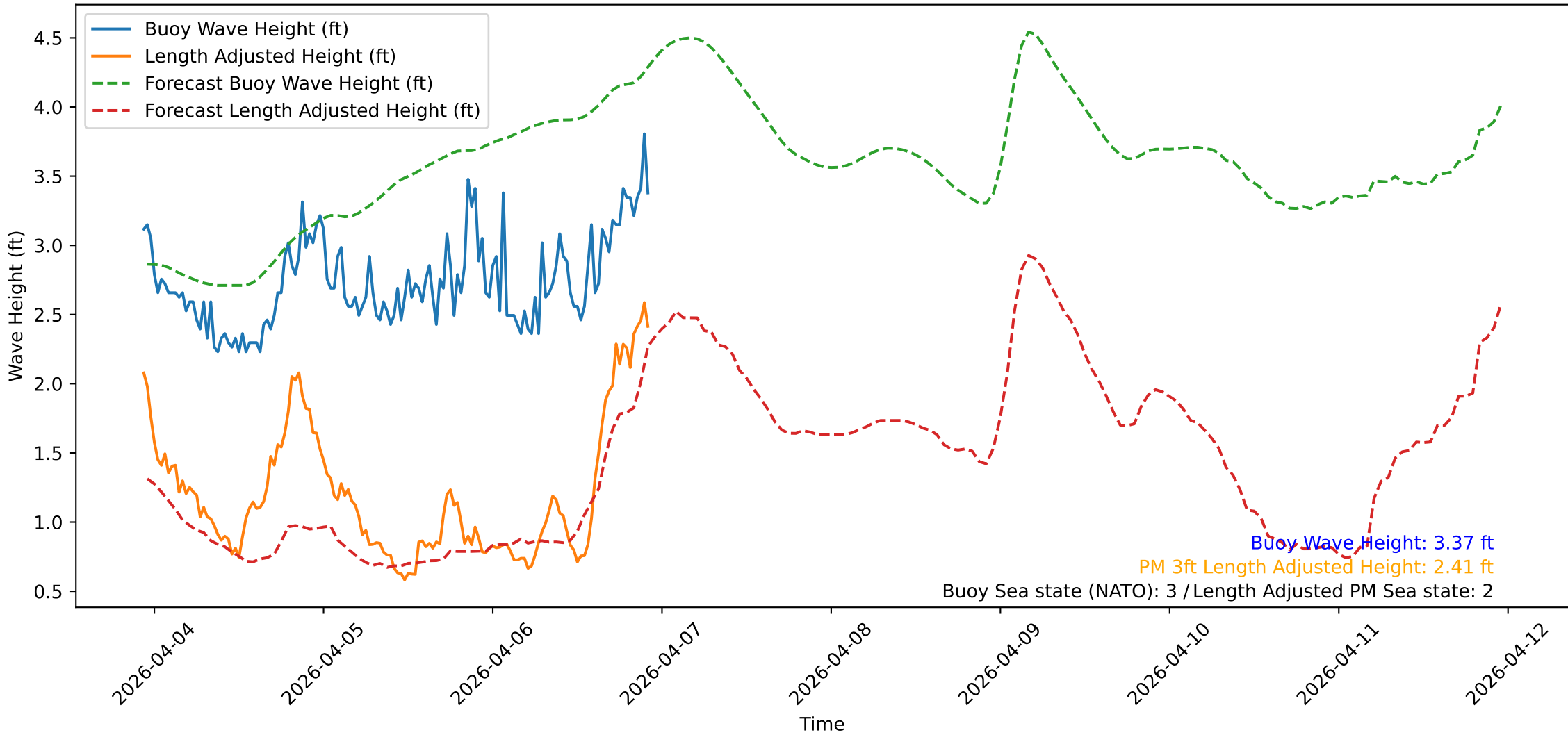
Wave Heights over Time for Green Beach at 2026-04-06 22:41:11
