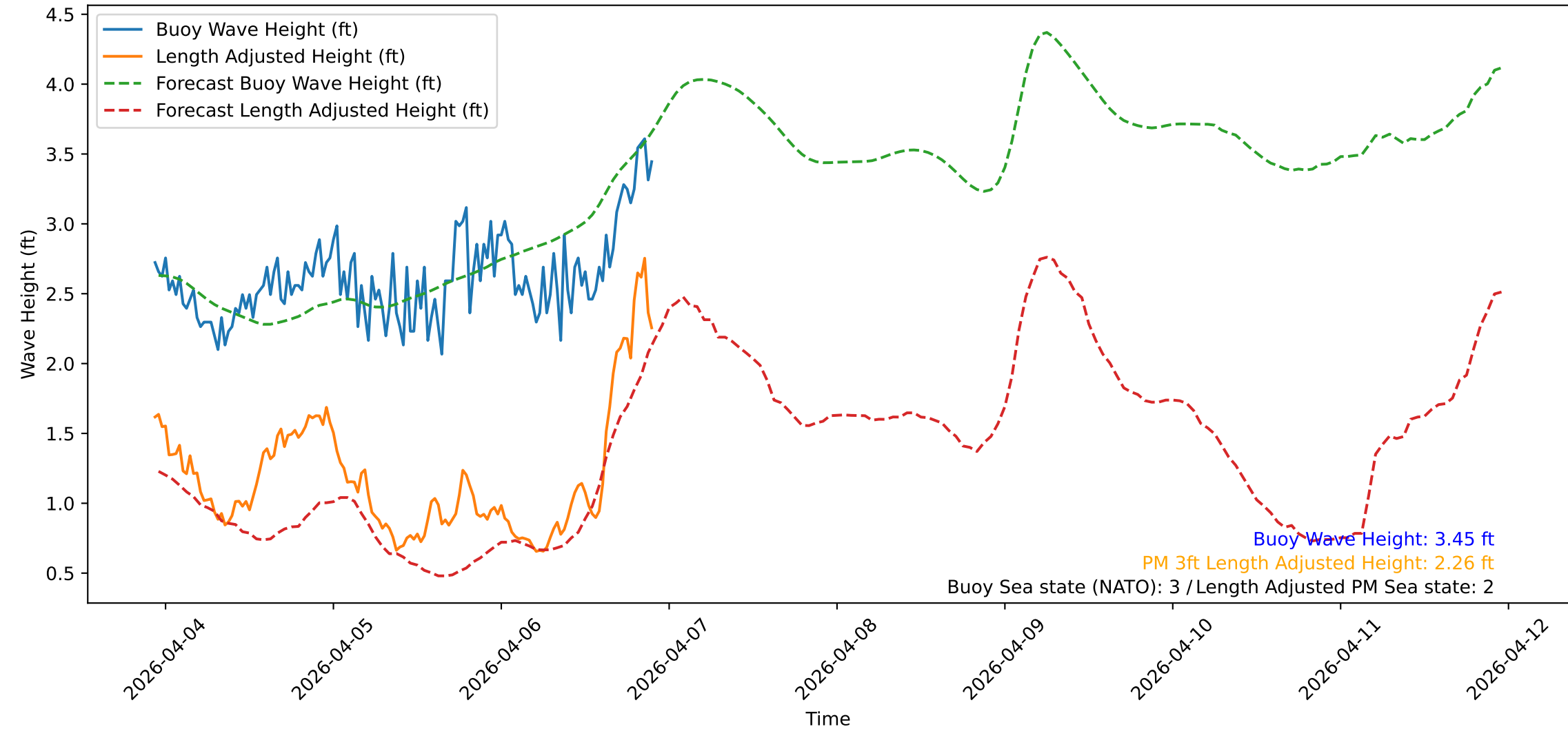
Wave Heights over Time for Oceanside Harbor at 2026-04-06 22:40:32
